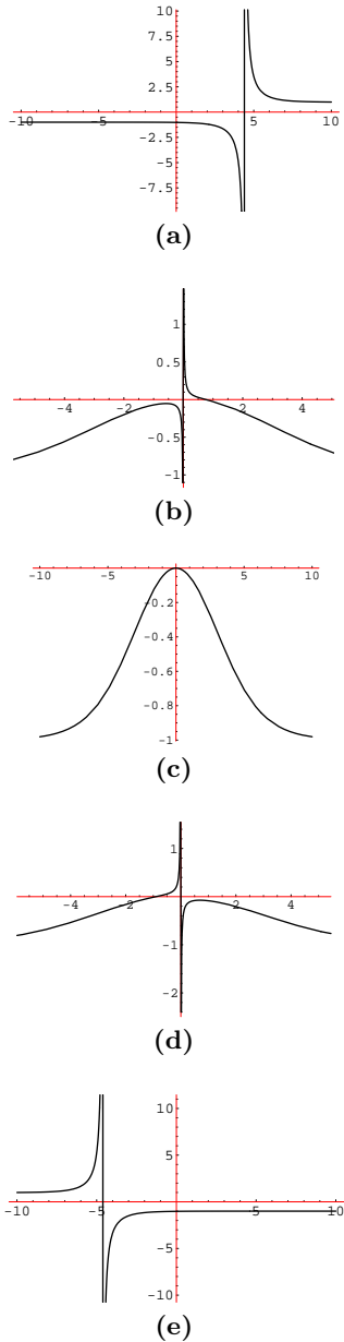
FIG. 2: (Color online) Interaction between singular soliton \coth \xi_1 and smooth soliton \tanh \xi_2 with parameters: (a) t = -3 , (b) t = -0.05 , (c) t = 0 , (d) t = 0.05 , (e) t = 3 .
