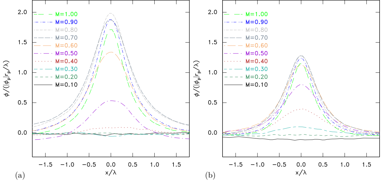
Figure 4: (Color Online) Wake transverse potential profile at y = 0 , z = 1 . (a) Collisionless plasma, (b) Collisional plasma. Near-linear regime: point charge \bar{Q} = -0.02 .
