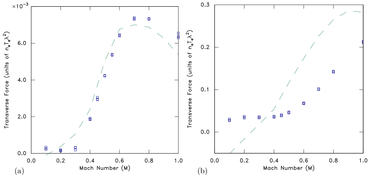
Figure 11: (Color Online) Transverse force in collisional plasma on an equal grain at downstream position z = 1 , x = 0.5 , y = 0 . versus flow mach number M . Points: two-grain simulation, total force; dashed line: gradient of one-grain wake potential. (a) near-linear regime: point charge \bar{Q} = -0.02 , (b) non-linear regime point charge \bar{Q} = -0.2 .
