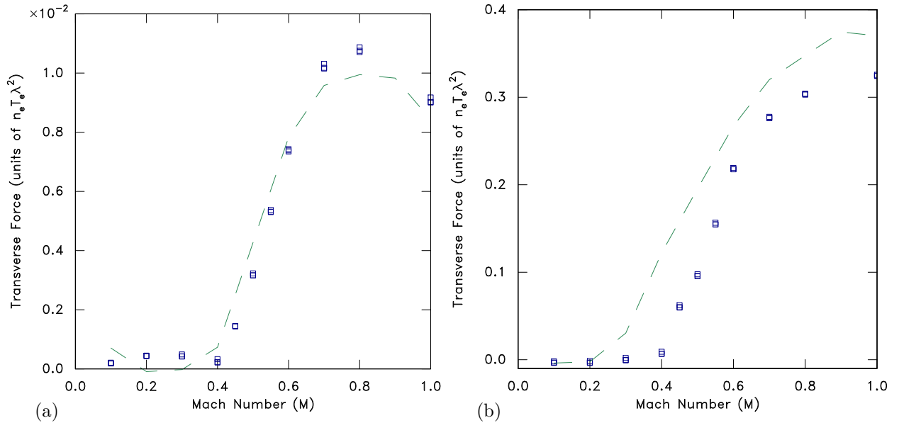
Figure 10: (Color Online) Transverse force in collisionless plasma on an equal grain at downstream position z = 1 , x = 0.5 , y = 0 . versus flow mach number M . Points: two-grain simulation, total force; dashed line: gradient of one-grain wake potential. (a) near-linear regime: point charge \bar{Q} = -0.02 , (b) non-linear regime point charge \bar{Q} = -0.2 .
