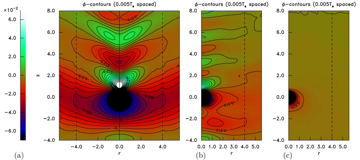
Figure 1: (Color Online) Wake potential contours for single grain. (a) M = 0.6 , (b) M = 0.4 , (c) M = 0.2 . Collisionless plasma, non-linear regime: point charge \bar{Q} = -0.2 .
