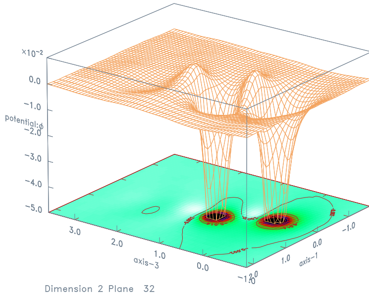
Figure 8: (Color Online) Wake potential for M = 0.3 . The slice shown is on the plane y = 0 . Collisionless plasma, near-linear regime: point charge \bar{Q} = -0.02 .
