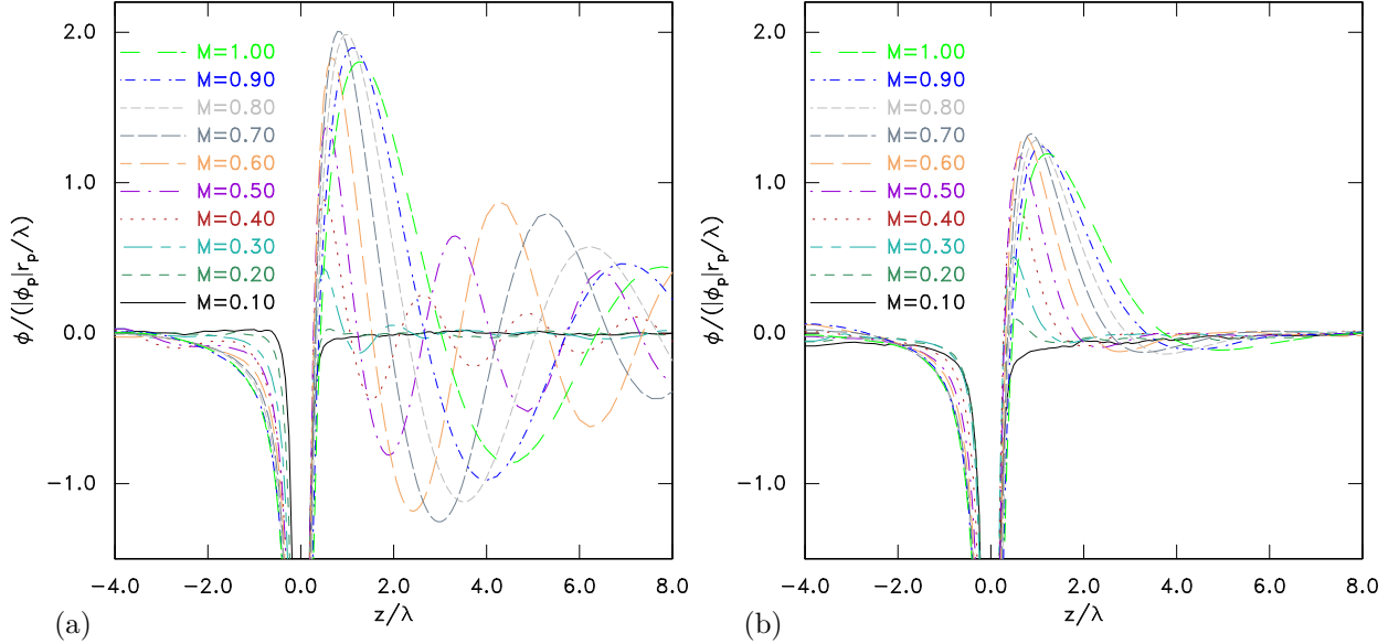
Figure 2: (Color Online) Wake axial potential profile for mach numbers M . Near-linear regime: point charge \bar{Q} = -0.02 . (a) Collisionless plasma, (b) Collisional plasma (collision time 1.3\lambda_{De}/c_s ).
