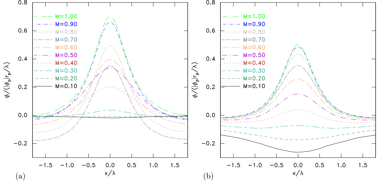
Figure 5: (Color Online) Wake transverse potential profile at y = 0 , z = 1 . (a) Collisionless plasma, (b) Collisional plasma. Non-linear regime: point charge \bar{Q} = -0.2 .
