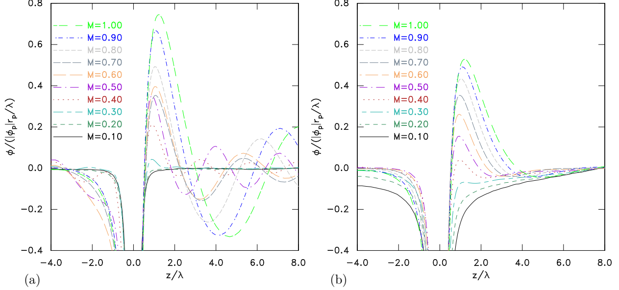
Figure 3: (Color Online) Wake axial potential profile for mach numbers M . Non-linear regime: point charge \bar{Q} = -0.2 . (a) Collisionless plasma, (b) Collisional plasma (collision time 1.3\lambda_{De}/c_s ).
