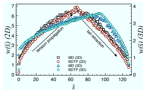
FIG. 2: (Color online) Comparison of waiting times w in both 2D and 3D for MD and the BDTP model. The agreement of the BDTP model with MD simulations is excellent, and reveals the two stages of translocation: the tension propagation stage of increasing w(\tilde{s}) and the tail retraction stage characterized by decreasing w(\tilde{s}) . The parameters used were the same for both MD and BDTP ( N_0 = 128 , f = 5 , k_B T = 1.2 , \eta = 0.7 ). The 3D MD results are from [33].
