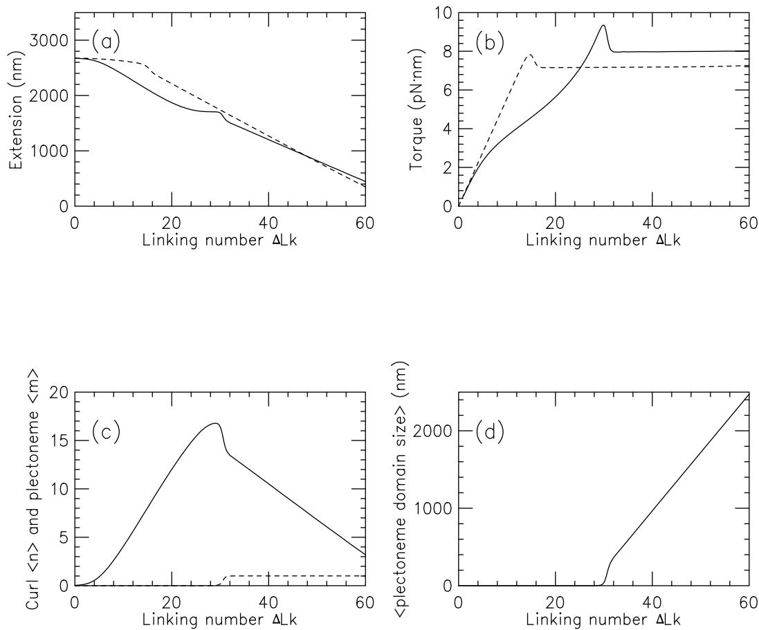
FIG. 8: Behavior of supercoiled DNA in the presence of curl-binding proteins. Calculations are shown for f = 0.5 pN, 150 mM salt, and \beta\mu = 10 . The presence of the curl-binding proteins stabilizes the curls and drives formation of many curls at the buckling transition. Extension as a function of \Delta Lk is shown as the solid curve in (a); torque is shown as the solid curve in (b); dashed curves indicate results without curl-binding proteins from Fig. 5. Curl ( \langle n \rangle , solid) and plectoneme ( \langle m \rangle , dashed) numbers are shown in (c) for the curl-binding protein case; the corresponding interwound length per plectoneme ( \langle L_p/m \rangle ) is shown in (d).
