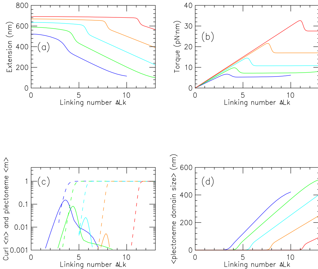
FIG. 3: (Color online) Properties of stretched twisted DNA as a function of linking number, for a 2.2 kb molecule in 150 mM Na + buffer, for forces of 0.25 (blue), 0.5 (green), 1 (cyan) 2 (orange) and 4 pN (red).
