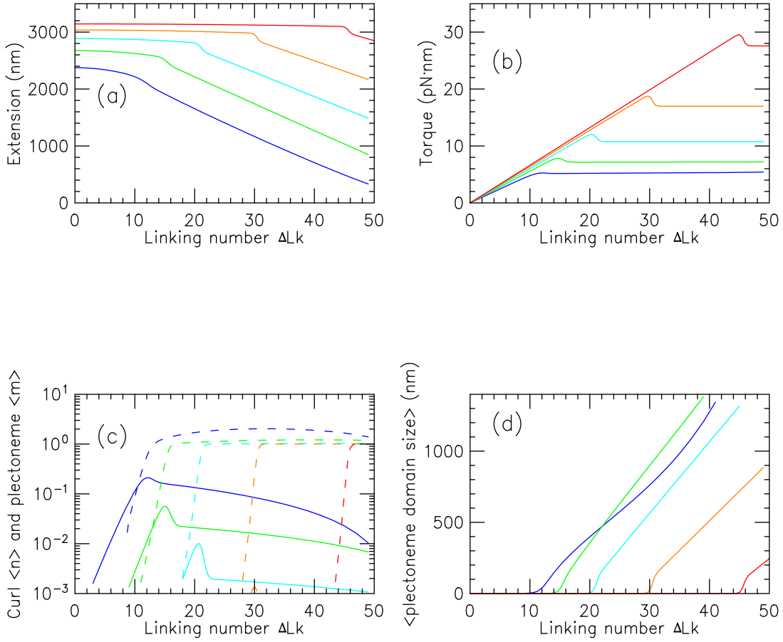
FIG. 5: (Color online) Properties of stretched twisted DNA as a function of linking number, for a 10 kb molecule in 150 mM Na + buffer, for forces of 0.25 (blue), 0.5 (green), 1 (cyan), 2 (orange) and 4 pN (red).
