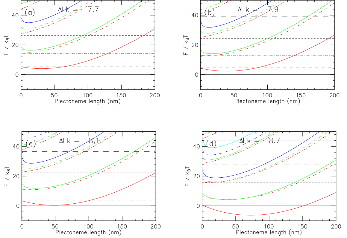
FIG. 2: (Color online) Free energies of states with different (n, m) and L_p near buckling transition for 2.2 kb molecule in 150 mM Na + buffer subject to 2 pN force. Free energies are measured relative to that of the n = 0, m = 0 state. Horizontal black lines indicate straight DNA with different numbers of chiral curls and no plectonemic domains ( m = 0 ): solid, n = 0 ; dashed, n = 1 ; dot-dashed, n = 2 ; short dashed, n = 3 ; long dashed, n = 4 . Curves indicate free energy as function of length of interwound plectonemic region for states with successively larger numbers of plectonemic regions: the line dash style indicates the number of curls in that state, following the same labeling as the straight-curl states. Plectonemic states with m = 1, 2, 3 and 4 for each value of n (each dash type) have free energies which increase with m for each value of plectoneme length ( m = 1, 2, 3 and 4 are shown in red, green, blue and cyan, respectively). Parts (a), (b), (c) and (d) show the free energies for successively larger linking numbers passing through the buckling transition. The uppermost solid line in (d) shows the (5, 0) state.
