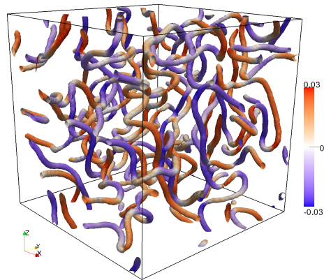
FIG. 1. Snapshot of a measure of the charge density vector field for a configuration of vortex filaments in 3D simulation of phase ordering. The figure shows the x-component \mathcal{D}_x of the Jacobian determinant defined in Sec. II. The system size in this simulation is 128^3 .
