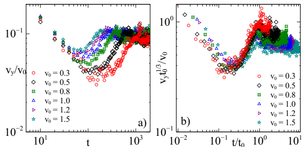
FIG. 7. (Color online) a) Evolution with time of the ensemble average of the velocity component v_y \equiv \langle |v_y(t)| \rangle for different values of the shear rate. b) Rescaled v_y plotted as a function of the rescaled time t/t_0 .
