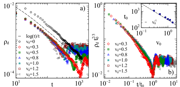
FIG. 5. (Color online) a) Density of defects \rho_d as a function of time t for different values of the imposed shear velocity v_0 . b) Data collapse of the rescaled density with the mean density in the statistical steady state \rho_0 \sim t_0^{-2/3} , where t_0 is the cross-over time to the steady state. Inset figure shows how t_0 scales with v_0 as t_0 \sim 1/v_0 .
