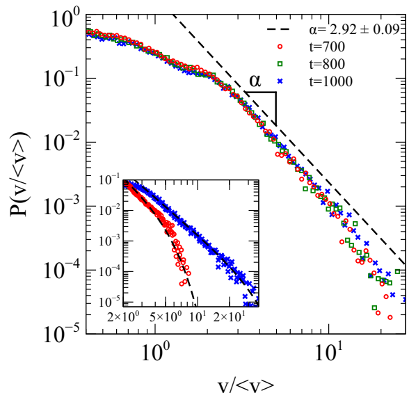
FIG. 3. (Color online) Collapsed probability distribution function (scaling function) of absolute velocity of point vortices in 2D during phase ordering. (Inset) PDF of the defect velocity for different core sizes (open circles correspond to larger core size and crosses correspond to smaller core size) to show that the Gaussian cut-off depends effectively on the vortex core size. The model parameters for the inset figure are A = 2.05 (open circles), A = 1.05 (crosses) and C = 3/20(1 + A) . In the main graph, A = 1.5 . Here v \equiv |\mathbf{v}| .
