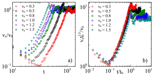
FIG. 6. (Color online) a) Evolution with time of the ensemble average of the velocity component v_x \equiv \langle |v_x(t)| \rangle for different values of the shear rate. b) Data collapse of the rescaled v_x as a function of the rescaled time t/t_0 .
