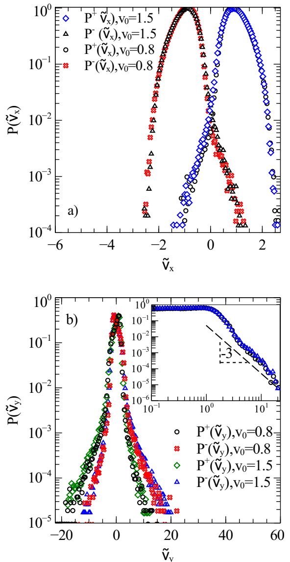
FIG. 9. (Color online) (a) PDF of the gliding velocity for positive (open diamonds and circles) and negative (open triangles and crosses) dislocations in the statistically stationary state at a different shear rates. (b) Probability distribution function of the climb velocity for positive (open circles and diamonds) and negative (open crosses and triangles) dislocations in the statistically stationary state. In both cases, the rescaled velocity variable is \tilde{v}_j \equiv v_j/\langle |v_j| \rangle for j = x, y . Inset figure shows the log-log plot of the tail PDF with logarithmic binning.
