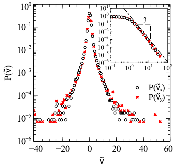
FIG. 8. (Color online) The time independent scaling function of the probability distribution corresponding to climb (crosses), respectively glide (open circles) velocities during the phase ordering in the absence of external field. The rescaled velocity variable is given as \tilde{v}_j \equiv v_j / \langle |v_j| \rangle for j = x, y . In the inset figure it is shown the log-log plot of the PDF calculated with logarithmic binning.
