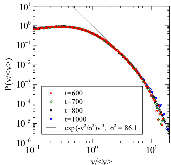
FIG. 4. (Color online) The scaling function of the probability distribution function of the absolute velocity of vortex filaments in 3D during phase ordering. Here v \equiv |\mathbf{v}| .
