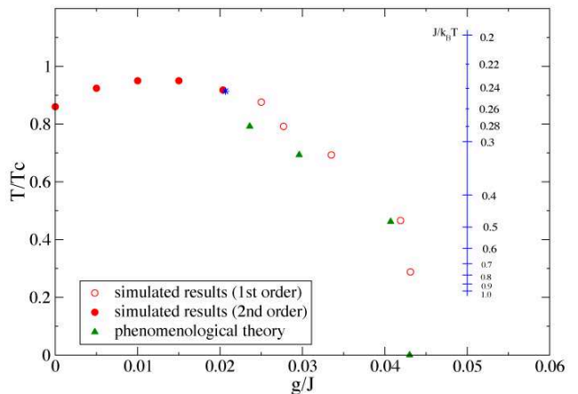
FIG. 8: Phase diagram of the Ising thin film ( D = 12 ) plotted in the plane of variables T/T_{cb} and g/J . Second-order transitions (from state (2) in Fig. 1 at low temperature to state (1) at higher temperature) are shown by full dots, first-order transitions (from state (2) to state (3)) are shown by open circles. The tricritical point is shown by a star. Triangles show estimates based on Eq. (6).
