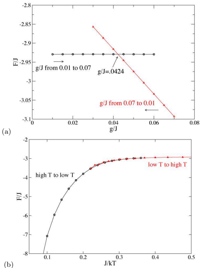
FIG. 3: (Color online) Free energy as obtained from thermodynamic integration varying g/J at constant temperature ( J/k_B T = 0.467 , L = 256 , case a) and varying inverse temperature J/k_B T at constant g/J = 0.025 (b). In (a), the estimated transition point (at g/J = 0.0424 ) is highlighted.
