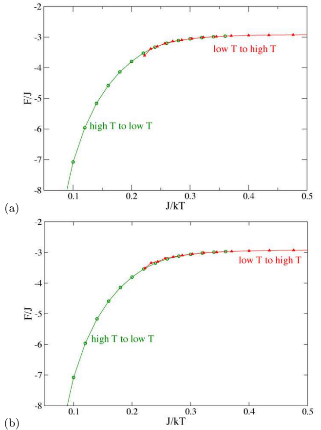
FIG. 4: (Color online) Free energy as obtained from thermodynamic integration varying J/k_B T at fixed g : (a) g/J = 0.01 ; and (b) g/J = 0.0 .
