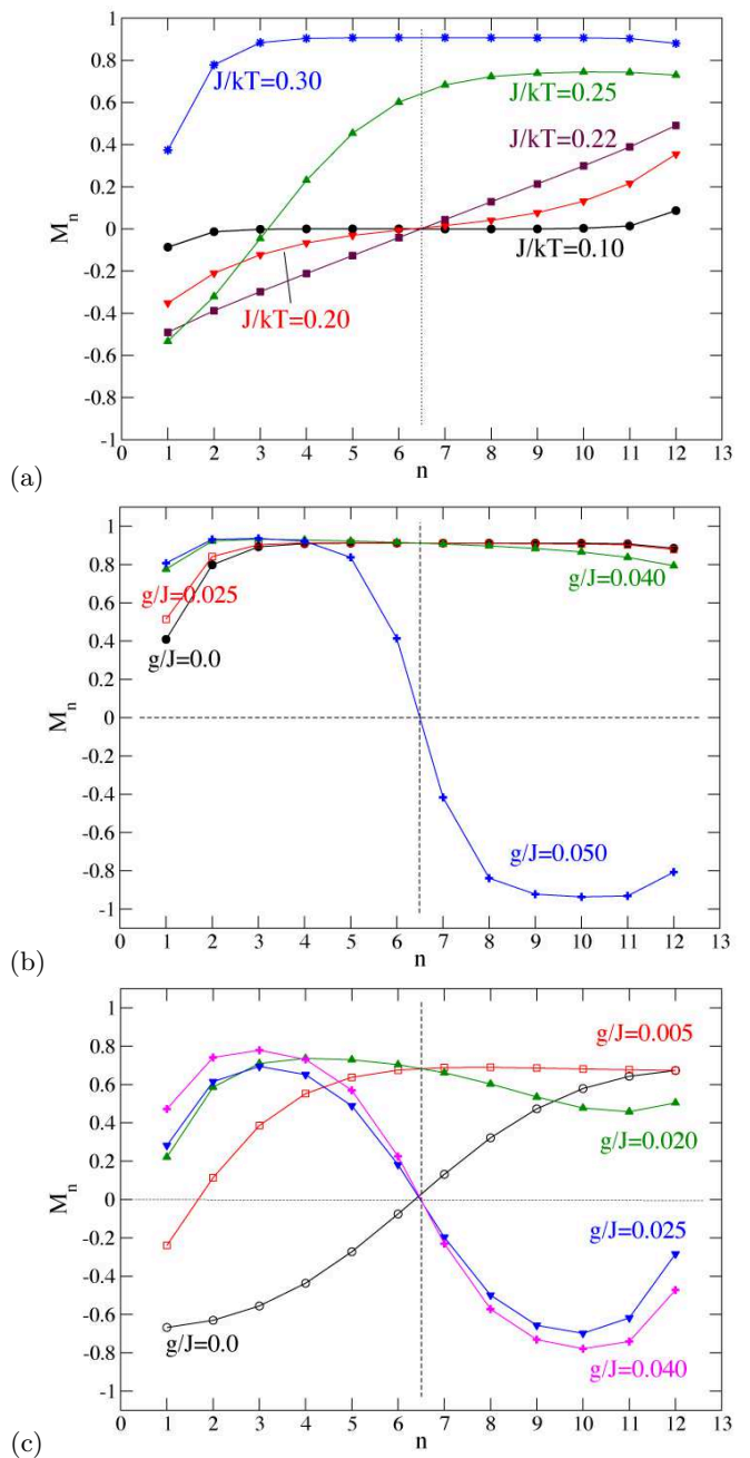
FIG. 2: (Color online) Layer magnetization m_n versus layer number n for the case L = 128 , D = 12 , H_1 = -H_D = -0.55J : (a) g/J = 0.01 and several choices of J/k_B T ; (b) J/k_B T = 0.303 and several choices of (g/J) ; (c) J/k_B T = 0.244 and several choices of g/J . Note that m_n is defined only for integer values of n , and data points are connected by straight lines to guide the eye. The mid-plane (which in the continuum limit where z runs from z = 0 to z = D has been denoted as z = D/2 in Sec. II) is located at z = (1 + D)/2 = 6.5 (vertical broken line), since for D = 12 there are 12 lattice planes from n = 1 to n = 12 . The horizontal broken straight line highlights zero magnetization.
