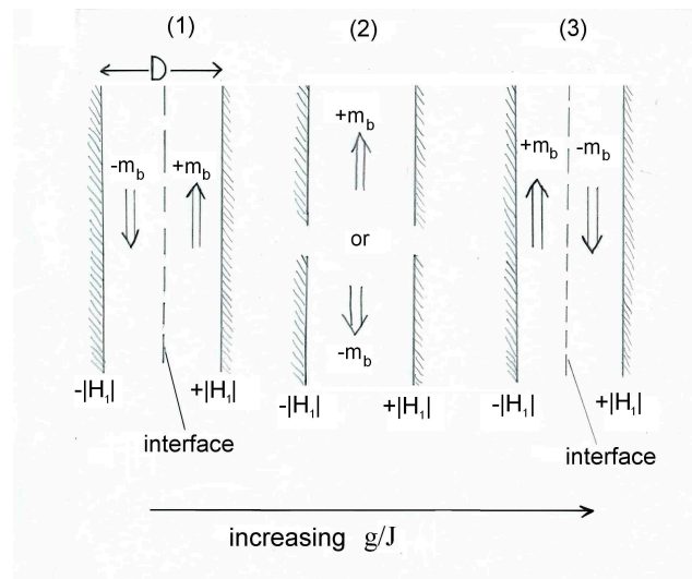
FIG. 1: Schematic description of the sequence of phases observed for D \rightarrow \infty in the temperature regime T_w < T < T_{cb} when the strength of the field gradient g/J increases. For small enough g/J the surface fields dominate, and there are two domains, separated by an interface parallel to the walls (state (1)). In this state the sign of the magnetization and of the surface field at the adjacent wall are the same and the magnitude of the magnetization equals the value in the bulk ( m_b ). In state (2) the gradient energy essentially compensates the surface effects yielding a degenerate state with the entire film being being predominantly positively ( +m_b ) or negatively magnetized ( -m_b ). In state (3) the gradient energy dominates: there are two domains of opposite magnetization but the signs are opposite to that of the surface field at the adjacent wall.
