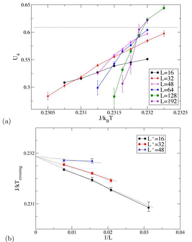
FIG. 5: (Color online) (a) 4th order cumulant U_L plotted vs. inverse temperature for the case D = 12, H_1 = -H_D = -0.55J, g/J = 0.015 , and several choices of L . The dotted horizontal straight line indicates the expected result [42–44] for the universality class of the d = 2 Ising model. (b) Extrapolation of the values of the inverse temperature J/k_B T of crossing points vs L^{-1} for different choices of the reference lattice size L' . The dashed lines are straight lines fitted to the data.
