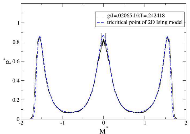
FIG. 7: (Color online) Normalized probability distribution P_L^*(M^*) = \langle M^2 \rangle^{-1/2} P_L(M) vs M^* = \langle M^2 \rangle^{-1/2} M generated at J/k_B T = 0.24167 , g/J = .0204 and reweighted to J/k_B T = 0.242418 , g/J = .02065 , as indicated, compared to the planar Ising model distribution at tricritical point [46].
