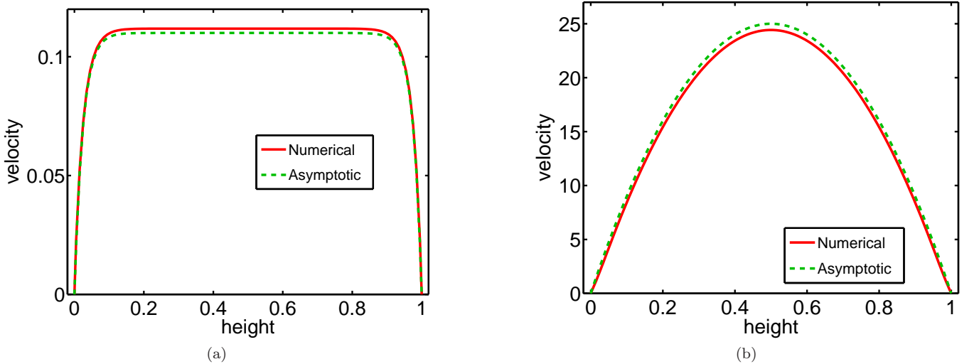
FIG. 13. (Color online) Comparison of the numerical solution to equation (12) and the asymptotic solution (a) on the lower branch in the plug flow regime and (b) on the upper branch in the parabolic flow regime for f = 0.1 and \epsilon = 5 \cdot 10^{-4} . The error in the asymptotic approximation is around 2% in both cases.
