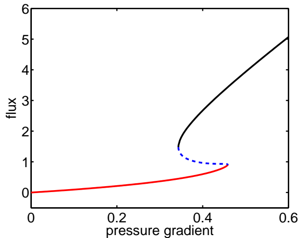
FIG. 8. (Color online) Flux as a function of applied pressure gradient, where the velocity profile satisfies equation (17) which includes the effect of pressure relief. The value of \epsilon is 5 \cdot 10^{-4} and the value of \delta is 0.1. The unstable solution is represented by a dashed line.
