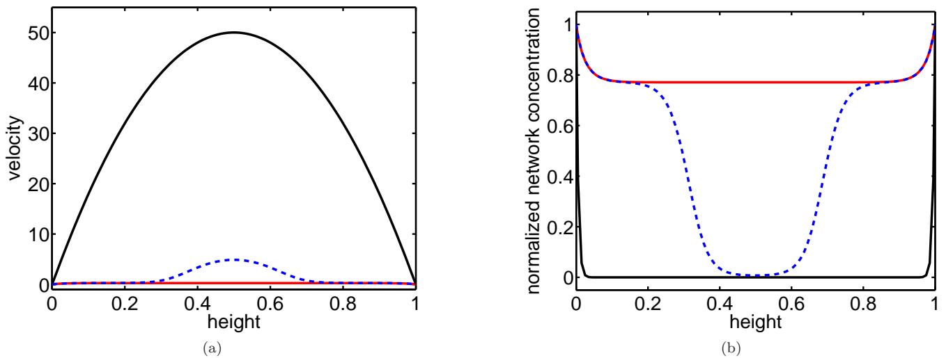
FIG. 6. (Color online) Solutions to equation (12) for \epsilon = 5 \cdot 10^{-4} at f = 0.20 . The unstable solution is represented by a dashed line. (a) Velocity profiles. (b) Normalized network concentration.
