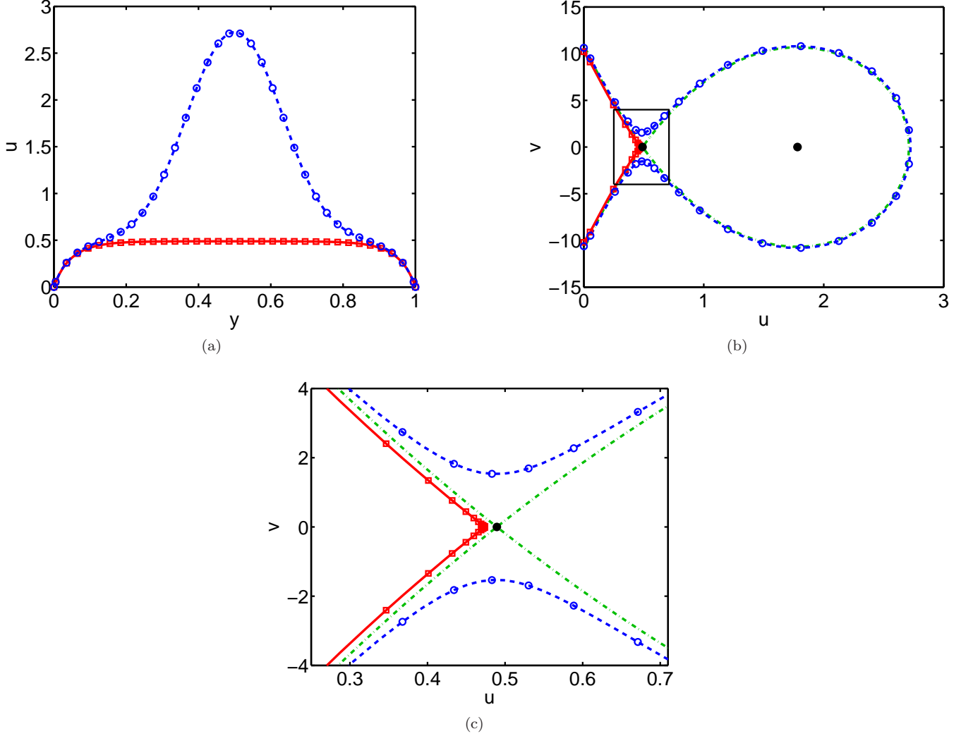
FIG. 15. (Color online) (a) Plug flow solution (red squares) and channeled solution (blue circles) for f = 0.30 and \epsilon = 10^{-3} . (b) Solutions plotted in the phase plane along with the equilibrium points and the stable and unstable manifolds of the saddle point (green dash-dot curve). (c) Close up of the solutions around the saddle point.
