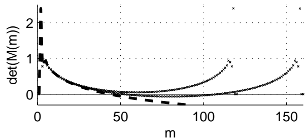
FIG. 4: Stability of discrete vs. continuous system for F(r) = \tanh(4(1-r)) - 0.5 . Top: \det(M(m)) . Dashed line corresponds to continuum eq. (10) and crosses to discrete eq. (9) with N = 120, 160 . Instability occurs iff \det(M(m)) < 0 . Bottom: steady states of discrete dynamics with N as indicated; inserts show the blowup of the ring structure.
