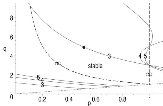
FIG. 2: Stability region for (2). The curves shown correspond to the boundaries of the stability \det(M(m)) = 0 , with m = 3, 4, 5 and m = \infty , as indicated. The line p = q is also drawn. Crossing any of the curves destabilizes the ring. The intersection of m = \infty and m = 3 boundaries is at p = 0.10779 , q = 9.277102 . Black dot is the position where we compute the pitchfork bifurcation in Figure 3.
