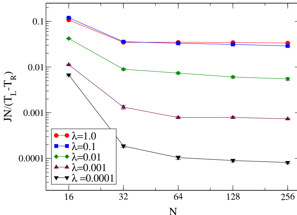
FIG. 1: (Color online) Plot of JN/(T_L - T_R) versus N for different values of \lambda . The parameter values were set at k_o = 4, k = 1, \Delta = 0.8 . All the data shown here were obtained from exact numerical computation.
