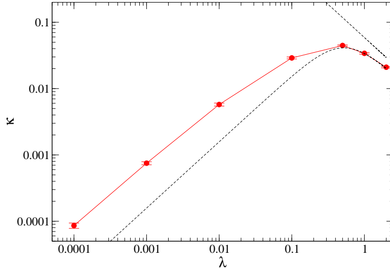
FIG. 2: (Color online) Plot of \kappa versus \lambda obtained from the numerical data in Fig. (1). The lower and upper bounds for \kappa_{GK} given by Eqs. (17,19) are shown by the dashed lines.
