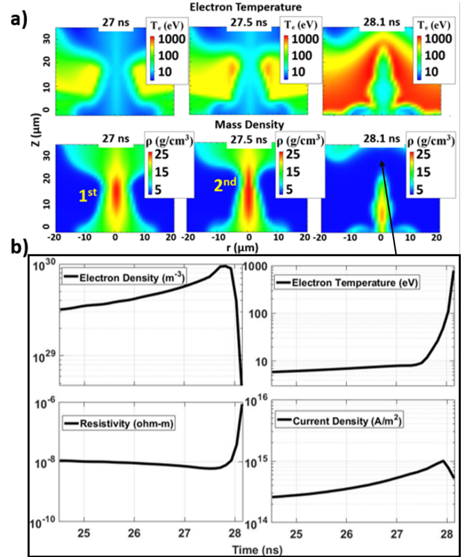
FIG. 3. a) Three temporal simulation snapshots displaying the electron temperature and the mass density at 27 ns, 27.5 ns, and 28.1 ns. The figure shows the cascading sausage instability as seen in the mass density renders, marked as 1st and 2nd. b) Electron density, electron temperature, plasma resistivity, and current density as a function of time in a 1 \mu\text{m} cell in the plasma neck at the location indicated by the black arrow.
