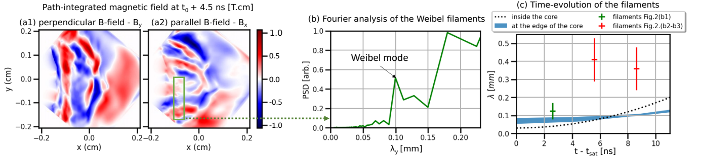
FIG. 3. (a1-a2) reconstructed path-integrated magnetic field from the 16-MeV proton image at t_0 + 4.5 ns (Fig. 2(b1)). (b) Power spectral density (PSD) analysis of Weibel-like filaments. The Fourier analysis was performed in the green rectangle of (a2). (c) Estimation of the filament size at 4.5 ns (green) and 7.5, 10.5 ns (red). The measurement is compared to the coalescence model of the ion-Weibel filaments in the plasma condition of the core center (dashed black line) and at the edge of the core (blue line). t_{sat} is the saturation time and we estimate t_{sat} = t_0 + 1.9 ns.
