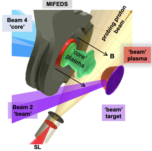
FIG. 1. Schematic of the experimental setup. The ‘beam’ plasma (red hemisphere) collides and propagates through the ‘core’ plasma (green blob) in the presence of an external magnetic field (generated by MIFEDS, grey box) aligned with the flow axis of the two plasmas.
