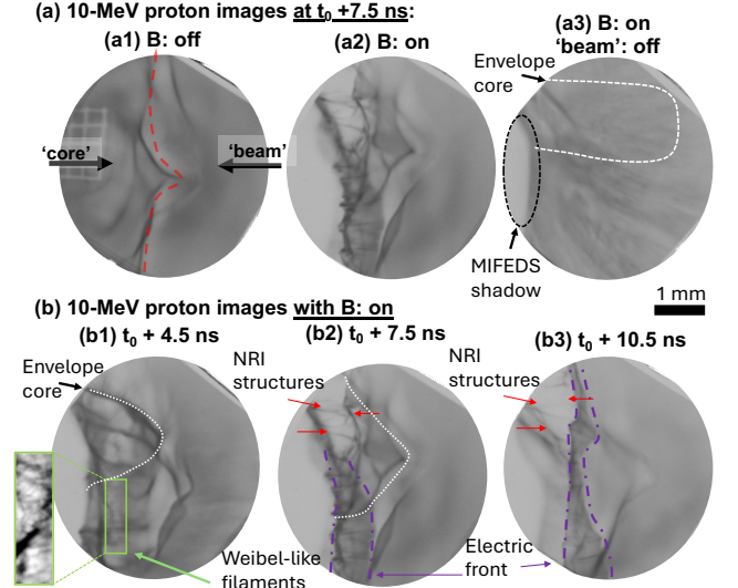
FIG. 2. 10-MeV proton images: (a) 7.5\text{ ns} after the initial asymmetric interaction ( t_0 ) without external B-field (a1), with the external B-field (a2), and core only with the external B-field (a3). Features are shifted up due to the external magnetic field. (b) 10-MeV proton images showing the temporal evolution of field structures at 4.5 , 7.5 , and 10.5\text{ ns} after t_0 . Light areas on the left-hand side in premagnetized shots are MIFEDS shadows. The white dotted lines in (a3), (b2), and (b3) are the approximate location of the core.
