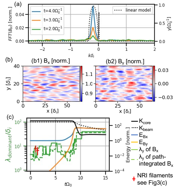
FIG. 4. (a) Calculated growth using the equation dispersion from Gary et al. [40] and the plasma parameters at t_0 (black dotted line). Solid lines are helicity-decomposed spectra of the perpendicular magnetic field at different times from simulation. (b1)-(b2) parallel and perpendicular components of the magnetic field calculated by the hybrid PIC code for plasma conditions taken at 4\Omega_0^{-1} . (c) Temporal evolution of plasma parameters: core kinetic energy (solid black line) and beam kinetic energy (dotted black line), parallel magnetic energy (blue line), perpendicular magnetic energy (orange line), and green lines are the wavelength ( \lambda_y ) of the dominant mode for B_x (solid) and B_x along the proton path as in the experiment (dashed). The red crosses are the NRI wavelength measured experimentally.
