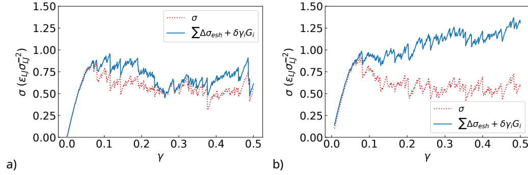
FIG. 4. Stress-strain curves from the simulation (dotted red line), and estimated from equation 5 with the parameters fitted from equation 4, a) example with good correspondence and b) poor correspondence.
