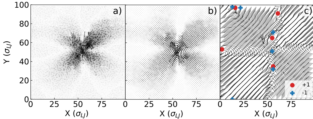
FIG. 1. Representation of the non-affine displacements during a plastic event: a) displacements mapped on atomic positions b) coarse-grained displacements c) normed coarsened-grained displacement vectors (black arrows) used to determine the topological defect positions (blue crosses for -1 defects and red circles for +1 defects)
