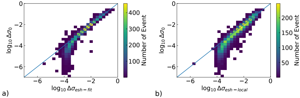
FIG. 3. 2D histogram of the stress drop of each event \Delta\sigma_0 : a) as a function of the stress drop computed from equation 5 using the parameters obtained with the Eshelby fit \Delta\sigma_{esh-fit} , b) compared to using the defect description parameters \Delta\sigma_{esh-loc} . The blue lines representing where the two are exactly equal.
