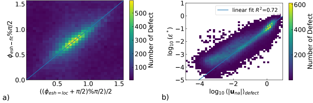
FIG. 2. a) Distribution of the angle \phi obtained from the fitting of the whole displacement field to equation 4 vis-à-vis \phi_{esh-loc} the angle of the local displacement field from equation 3. The diagonal blue line represents one-to-one correspondence. b) The eigenstrain of the Eshelby equation \varepsilon^* vis-à-vis the average displacement around the defect. The blue line represents the linear fit.
