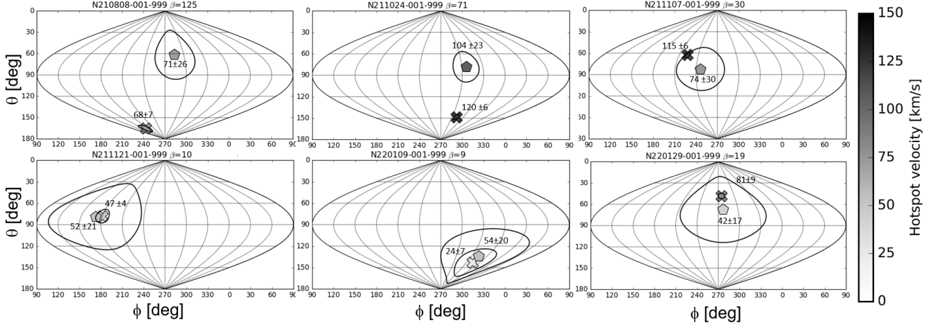
Figure 3: Analysis of the net asymmetry from all known seeds for N210808 and repeat experiments (including the yield dependence of v_{HS} from Eq 4) compared to the observed hot spot velocity ('X') (in grayscale in km/s).
