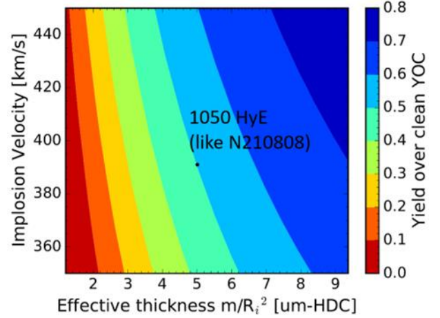
Figure 5: Contours of yield-over-clean (YOC) subject to a seed \ell=1 flux-asymmetry that induces YOC=0.5 at N210808-like initial conditions with a marginally igniting ( GLC=1 ) implosion plotted as function of effective shell thickness. Also shown is the operating point of N210808, which achieved 1.37 MJ and GLC \sim P R / (420 \times 50) = 1.4 [1]. The contours show the higher implosion velocity and/or with thicker effective shells are more robust to mode-1 asymmetry.
