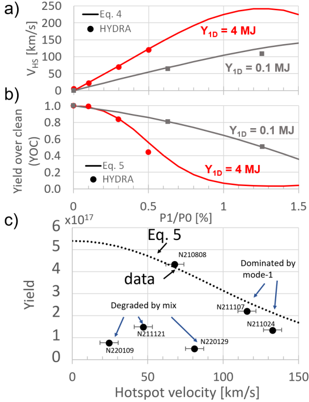
Figure 4: a) v_{HS} (a) and YOC (b) vs initial seed p_1/p_0 for the analytic model and 2D HYDRA simulations for an implosion with a 1D yield of 4 MJ (red) and an implosion with a 1D yield of 0.1 MJ (grey). c) Plot of nTOF measured v_{HS} vs yield for N210808 and repeat experiments compared to the \alpha -on piston model scaled to N210808. This analysis indicates that N211024 and N211107 were significantly degraded by \ell=1 asymmetry and suggest that even N210808 suffered some degradation from 1D.
