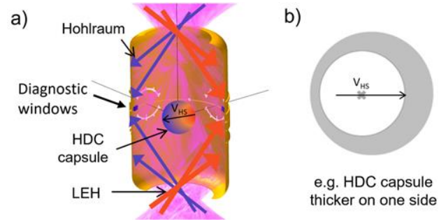
Figure 1: Two main classes of \ell=1 asymmetry seeds have been identified: a) drive (laser, and hohlraum penetrations, ie. windows) and b) capsule-ablator asymmetries.
