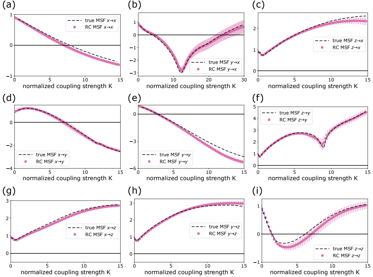
Figure 1. Master Stability Function of the true Lorenz system (black dashed line) and the coupled reservoir system (pink dots). A solid black line is shown at 0 to indicate the stability boundary.
