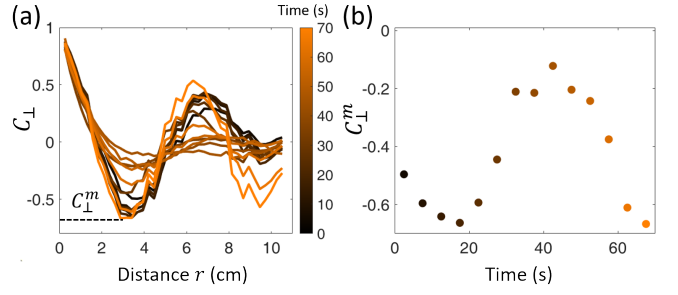
FIG. 4. Increase and decrease of coherence of long wavelength modes within a quasiperiod. (a) The equal time transverse spatial velocity correlation C_{\perp} averaged over time intervals of duration 5 s (100 frames) for the f_d = 88 Hz data shown in Fig. 1d. The color changes with time from 0 s - 5 s (black) to 65 s - 70 s (light orange). The strongly negative correlations are consistent with the predominantly transverse polarization of long wavelength oscillations. The more negative the minimum value C_{\perp}^m , the stronger are the correlations. (b) C_{\perp}^m as a function of time during the quasiperiod. Colors correspond to the data in (a).
