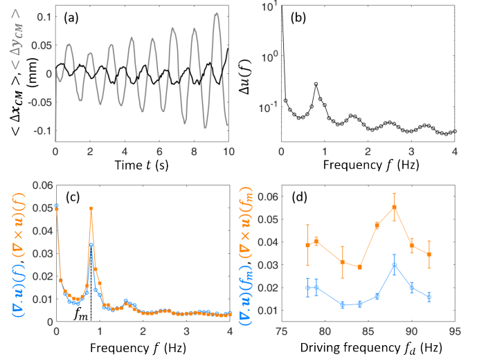
FIG. 3. Enhancement of transverse fluctuations due to resonant amplification of membrane modes. (a) Time series of the X (black) and Y (grey) coordinates of the center of mass prior to disordering of the lattice, for f_d = 88 Hz. (b) \Delta u(f) versus frequency f for the same data as shown in (a), showing a prominent peak at the oscillation frequency of the long wavelength mode. (c) Curl (\nabla \times \mathbf{u})(f) (filled orange squares) and divergence (\nabla \cdot \mathbf{u})(f) (open blue circles) of displacements of intensity maxima as a function of frequency f . The frequency corresponding to the peak, f_m , corresponds to the frequency of long wavelength oscillations shown in (b). (d) The peak values of curl ((\nabla \times \mathbf{u})(f_m)) , filled orange squares) and divergence ((\nabla \cdot \mathbf{u})(f_m)) , open blue circles) of displacements of intensity maxima as a function of driving frequency f_d . Error bars are standard errors of the mean across three distinct quasiperiods.
