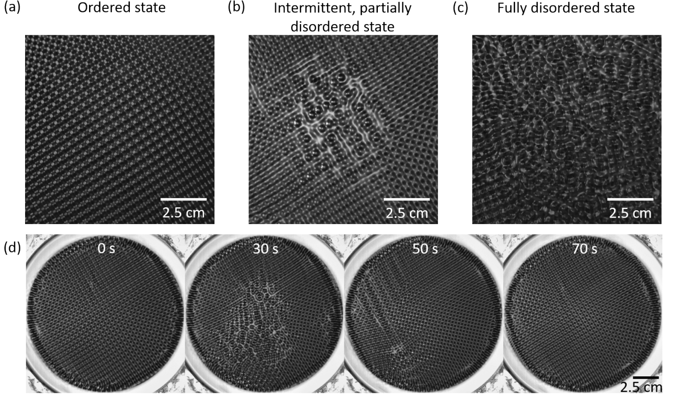
FIG. 1. Quasiperiodic transitions between order and disorder in Faraday waves. Snapshots of our system for a fixed driving frequency f_d = 88 Hz. (a) An ordered Faraday wave lattice at peak vibration acceleration \gamma = 5.4g , (b) an intermittent partially disordered state at \gamma = 5.95g , and (c) a fully disordered state at \gamma = 6.5g . (d) A time sequence of snapshots during a typical quasiperiod from the same data set as in (b), showing the onset of disorder followed by the clearing of defects and reordering of the lattice.
