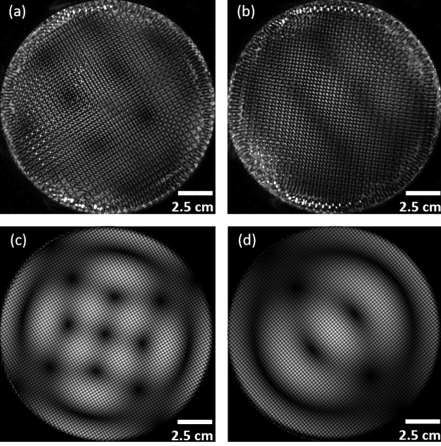
FIG. 2. Spatial structure of long wavelength modes. (a-b) Visualization of the spatial structure of long wavelength modes for f_d = 88 Hz (a), and f_d = 79 Hz (b). The images in (a) and (b) represent the pixel-wise standard deviation of image intensity over one oscillation time period ( \approx 1 s) leading up to disordering of the lattice. The image intensity has been uniformly multiplied by 3 to facilitate clearer visualization. (c-d) Visualization of the geometry of theoretically predicted normal modes of a circular elastic membrane, with mode numbers (2,2) (c), and (1,2) (d). The membrane diameter in (c-d) is chosen to be the same as for experiments shown (a-b).
