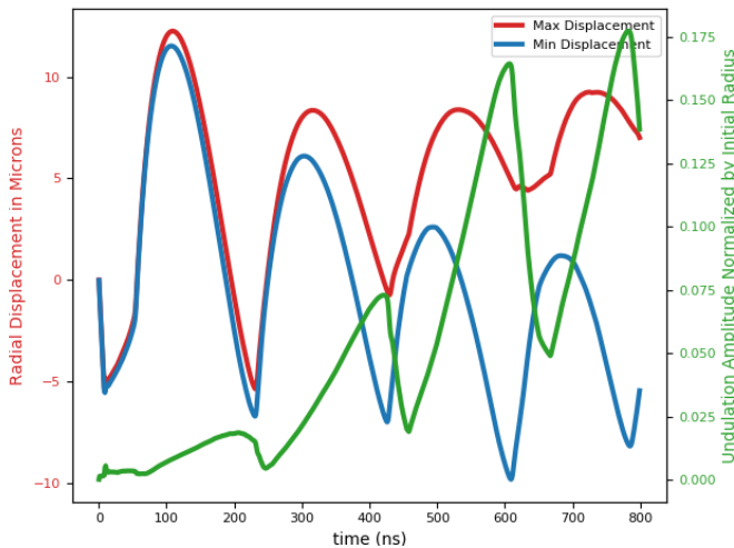
FIG. 3. Maximum (red) and minimum (blue) radial displacement along the boundary plotted over time. The difference between the two has been normalized by the initial radius of 90 \mu\text{m} and is shown in green.
