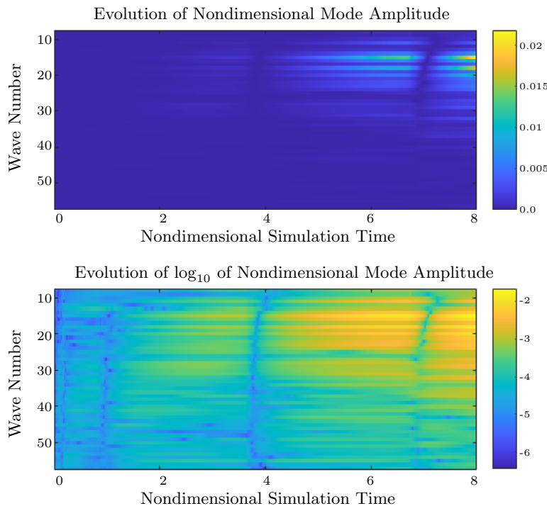
FIG. 7. Evolution of the Fourier modes of the surface undulation (normalized by the domain radius) plotted against nondimensional time \bar{t} = t/R_0\sqrt{\kappa/\rho} .
