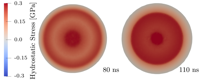
FIG. 4. Hydrostatic stress contours plotted at times 80, 110 ns. on a \pm 0.3 GPa scale. Observe the tensile wave traveling inward.
