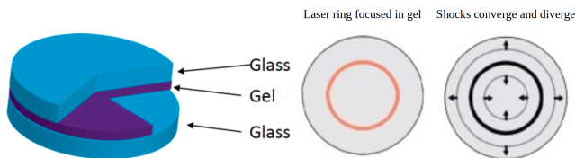
FIG. 1. Schematic of hydrogel specimen sandwiched between glass plates (left), detail of the initial circular 180\mu\text{m} -diameter laser ring (center) and waves emanated from laser-ablated ring (right).
