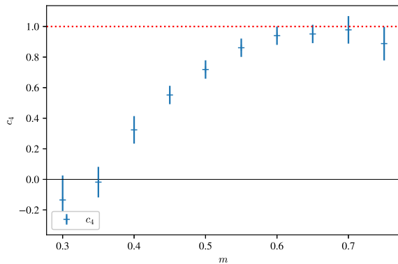
FIG. 19. Numerically estimated effective anharmonicity c_4 determined for anharmonic depinning using Eq. (B3). L = 64 and the initial condition is c_4 = 1 (red dotted line). The numerically estimated effective c_4 decreases as m decreases, vanishing within the precision of our simulation when m \approx 0.3 . There the error for c_4 increases, as the small system sees more system-spanning avalanches, crossing over to a single-particle behavior. Increasing L further increases this error, since c_4 is determined through a high-order harmonics of the driving signal, and scales \sim L^4 appearing in Eq. (B3). Still, qualitatively this confirms that c_4 can be dropped in the effective long-distance description of the model.
