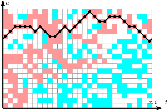
FIG. 4. Directed percolation from left to right. A site (i, u) is defined to be connected if it is occupied, and at least one of its left neighbors (i - 1, u) , (i - 1, u \pm 1) is connected. The index i takes the role of time t .
