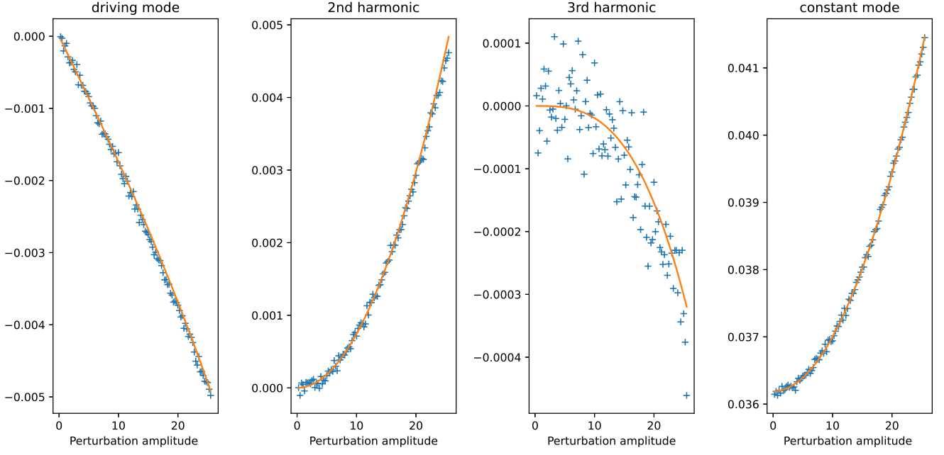
FIG. 16. Numerical estimation of the interface modes for different driving amplitude A . From the orange fits one obtains the coefficients {}^i u_j defined in Eqs. (77)-(80). For example, from the fit of the driving mode one obtains {}^1 u_1 and {}^3 u_1 . The polynomial behaviour predicted in Eq. (80) is verified. The shown plots are for anharmonic depinning, L = 1024 , and m = 0.06 . The perturbation amplitude is in lattice units.
