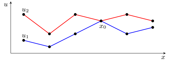
FIG. 2. Two configurations at depinning.
