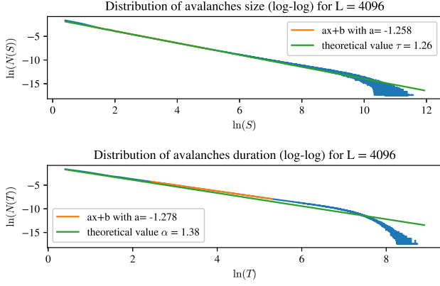
FIG. 9. Avalanches-size and duration distributions for TL92. \tau and \alpha are the associated exponents. We also computed S_m and T_m from these distributions at different m and verified the relations Eq. (52) and Eq. (56) (not shown).
