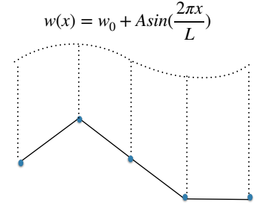
FIG. 14. We drive the interface with the spatially modulated driving given in Eq. (76), with f = 1 . The continuous black line and the blue dots represent the interface, while the grey dashed line represents w(x) .
