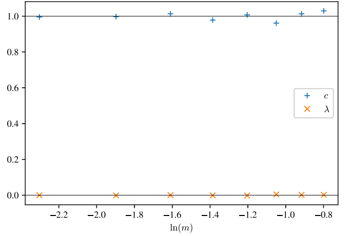
FIG. 13. The numerically estimated effective c and \lambda for the qEW equation. The effective elasticity c does not depend on m (with noticeable simulation errors at large m ), as predicted by the statistical tilt symmetry (STS). The numerically estimated non-linearity \lambda vanishes.
