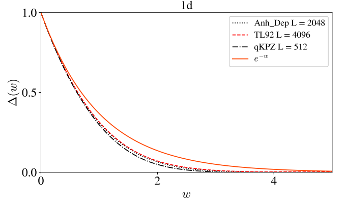
FIG. 11. Comparison of the shapes of the correlators in d = 1 and for anharmonic depinning, TL92 and qKPZ with the exponential behavior observed in a subspace in Ref. [49]. We clearly see (a): The correlators for TL92, aDep and qKPZ are very close. (b) The subspace found in [49] is not the one attained by the evolution of those models. The shapes have been normalized by setting |\Delta'(0^+)| = \Delta(0) = 1 .
