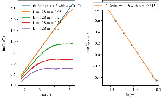
FIG. 7. Anharmonic depinning 2d (left) 2-point function C(x) alongside the diagonal of the system for different values of m (not all shown here) plotted against x' = \frac{4x\sqrt{2}(L\sqrt{2}-x\sqrt{2})}{\sqrt{2}L} . The exponent \zeta = 0.47 is extracted from the linear part of the curve. (right) Scaling of the plateau of the 2-point functions for different m . The fit gives \zeta_m = 0.61 .
