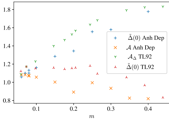
FIG. 17. \tilde{\Delta}(0) and \mathcal{A} for Anharmonic depinning and TL92 in d = 1 . They seem to converge to the same value, for this particular scaling choice.
