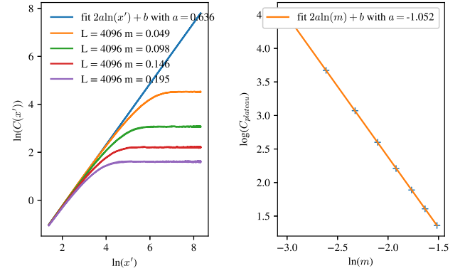
FIG. 5. TL92 1d (left) 2-point function C(x) for different values of m (not all shown here), plotted against x' = \frac{4x(L-x)}{L} to take advantage of the periodic boundary conditions. We read off the exponent \zeta = 0.636 in the linear part of the curve (the slope is 2\zeta ). (right) Scaling of the plateau of the 2-point functions for different m . The fit yields \zeta_m = 1.052 .
