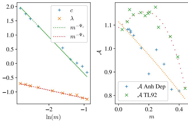
FIG. 15. Left: double-logarithmic plot for scaling of c and \lambda for anharmonic depinning in 1d as a function of m . Right: Measured amplitude ratios \mathcal{A} for TL92 and anharmonic depinning ( linear plot ). The dotted lines are guides for the eye. The second-order polynomial fits show convergence to \mathcal{A} \approx 1.10(2) for m \rightarrow 0 .
