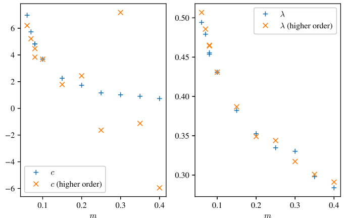
FIG. 18. Comparison of the different formulae (Eq. (87) and Eq. (B2) for a fit based on higher-order harmonics) for determining c and \lambda , for aDep in d = 1 . We see a good agreement for \lambda , while for c the higher-order harmonics are too noisy for m \geq 0.2 .
