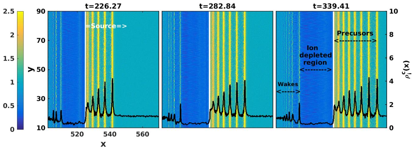
FIG. 2: Time evolution of the ion charge density \rho_i^c(x, y) due to passage of an infinite line source ( \delta x = 1.02, \delta y = L_y ). The source creates well developed trailing wake fields and precursor structures moving ahead of it. The line plots superposed on the snapshots are the profiles of the density \rho_i^c(x) as a function of x for y = 50.03 (its scale is given on right y axis).
