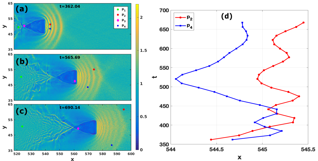
FIG. 7: (a)-(c) Tagging and tracking. p_1 (*), p_2 (•), p_3 (♦) and p_4 (■) are the four tagged particles. Initially p_2 and p_4 are the particles tagged between the two precursors and p_1 and p_3 are tagged at the back end of the bubble. Out of these four particles, one particle p_3 gets accelerated in the ion bubble/wake-field region and particle p_4 gets energized and eventually gets untrapped. (d) The bouncing motion of the trapped particles p_2 and p_4 is made evident from their trajectories in the x direction.
