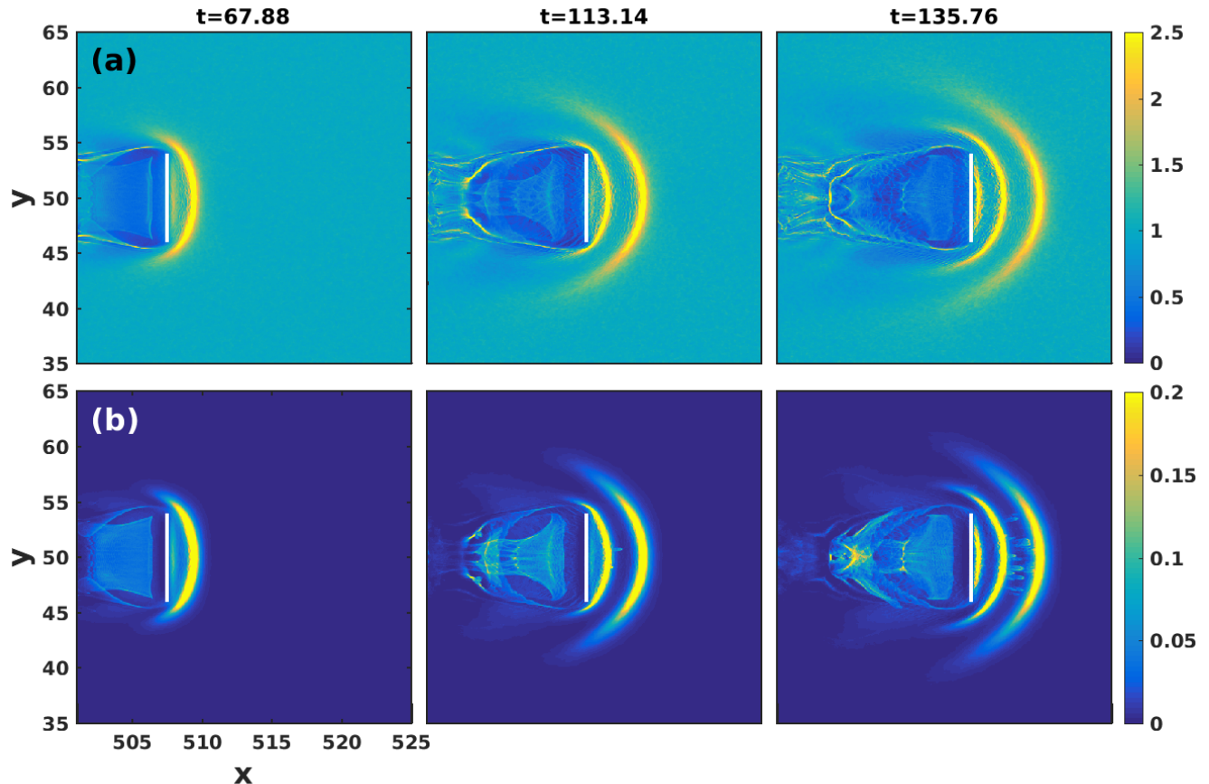
FIG. 6: The evolution of (a) the ion charge density \rho_i^e(x, y) at various times while (b) displays the corresponding ion kinetic energy K_i(x, y) . Some self-injection of ions is evident in the bubble regions in (a) as light blue regions showing ion accumulation in the otherwise dark blue ion evacuated region of the bubble. In (b) the yellow streaks between the two leading precursors indicate formation of energetic beam-lets.
