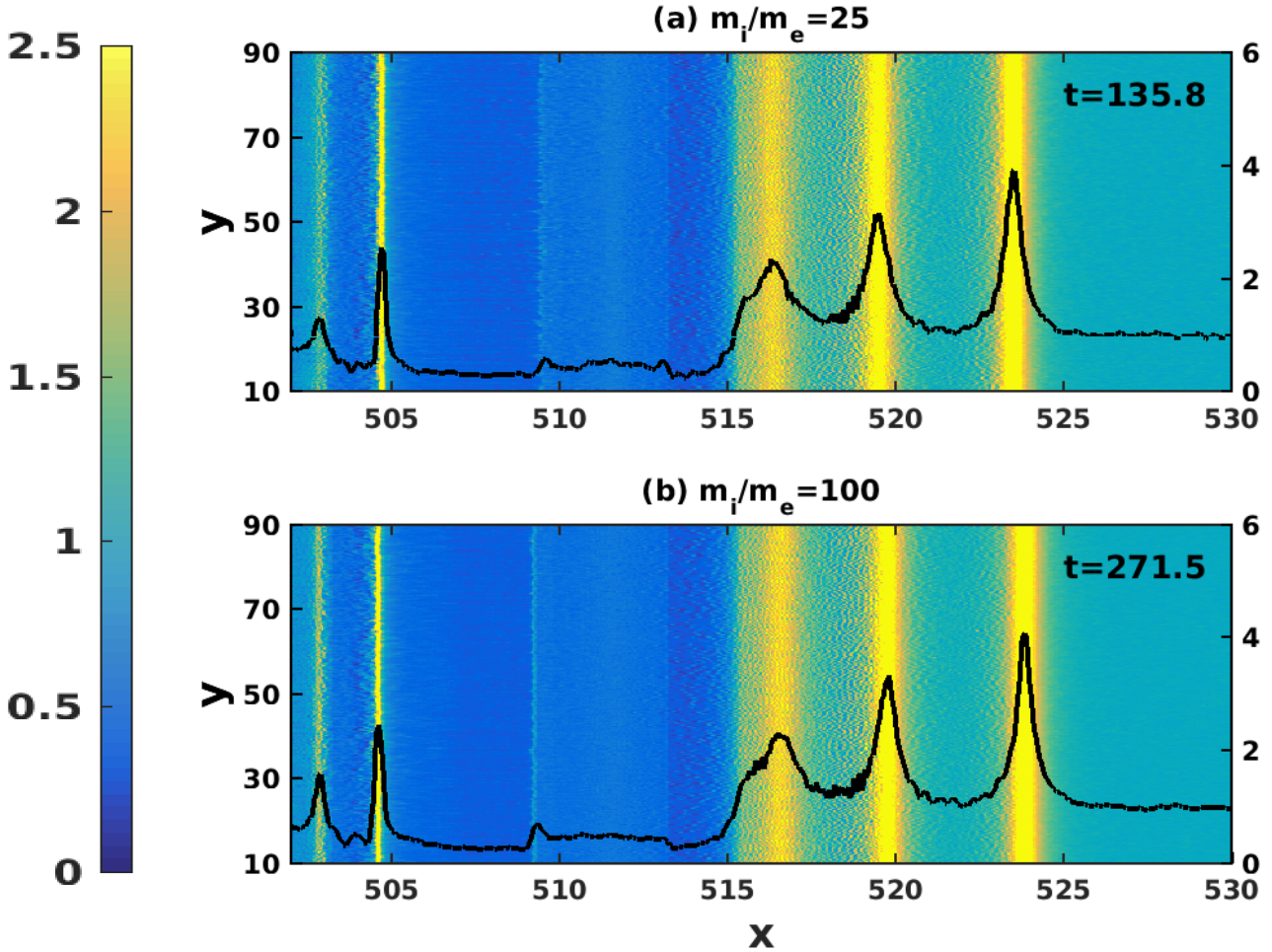
FIG. 9: A comparison of the precursor excitations by a line source for two different values of the mass ratio, namely 25 and 100 while maintaining the same Mach number of 1.1. As can be seen the basic phenomenon of precursor excitation and the nature of the precursor remains the same in both cases with a time delay that is linearly proportional to the ion acoustic speeds for the two cases. For the higher mass ratio of 100 the phenomenon occurs at twice the time period compared to that of 25.
