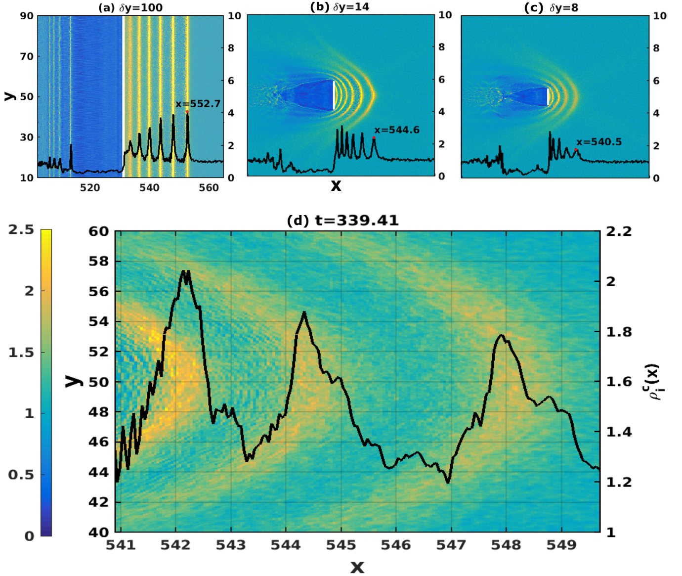
FIG. 5: Snapshots of the background ion charge density \rho_i^c(x, y = 50.03) at t = 282.84 , for charged sources of three different transverse lengths \delta y = 100, 14 and 8 at t = 282.84 to highlight the influence of the transverse dimension of the source on the shape of the precursor soliton. It is seen that with a decrease in the transverse size of the source the precursor soliton tips keep bending more and more backwards to form sharper crescent shapes. The vertical white line shows the location of the source. In (d) we present a zoomed view of (c). It is seen that the amplitudes of the precursors diminish with distance while their widths keep increasing. Numerical values of these quantities are given in Table I which shows that the product of their amplitudes a with the square of their widths L^2 remains constant. This is a characteristic property of a two dimensional soliton. Note: The colorbar is common for all the subplots (a)-(d).
