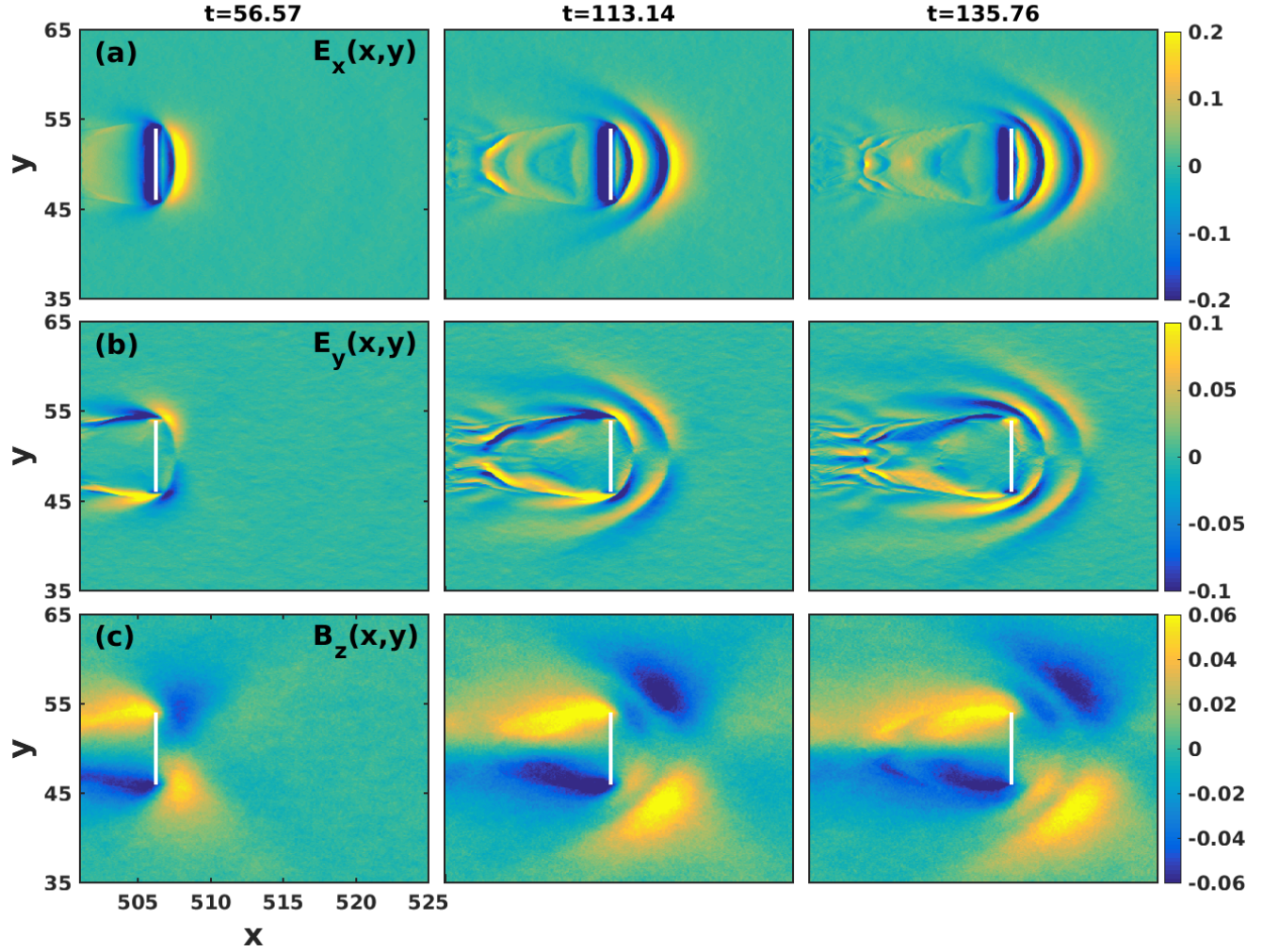
FIG. 8: The field components (normalised to m_e c \omega_{pe} / e ) of the excited waves: (a) E_x(x, y) , (b) E_y(x, y) and (c) B_z(x, y) . The presence of E_y and also a finite magnetic field component B_z show that these near-field wave components are no longer purely electrostatic, as was seen for the infinite planar charge source case, but have a non-negligible electro-magnetic component. This is another distinctive feature arising from the finite transverse dimension of the charged source.
