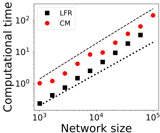
FIG. 3. Computational complexity of algorithms for multiplex reconstruction. We generate multiplex networks with variable size N . Tests are performed on synthetic multiplex networks with pre-imposed community structure constructed according to the LFR model with \gamma = 2.1 , \tau = 1.0 , k_{\max} = \sqrt{N} , \langle k \rangle = 5.0 , and \mu = 0.1 . Tests are also performed on networks without community structure that were generated using the configuration model (CM) with \gamma = 2.1 , k_{\min} = 3 and k_{\max} = \sqrt{N} . No correlation at the level of degree sequence and/or community structure is present between the layers of the multiplex. Given a network, we provide 50% of partial information to the degree- and community-based (DC) classifier and measure the time required by the algorithm to reconstruct the multiplex. Computational time is measured in seconds. Simulations were run on a Intel(R) Xeon(R) CPU E5-2690 v4 @ 2.60GHz. As guidelines, we display lines denoting the scalings N (dotted) and N \log N (dashed).
