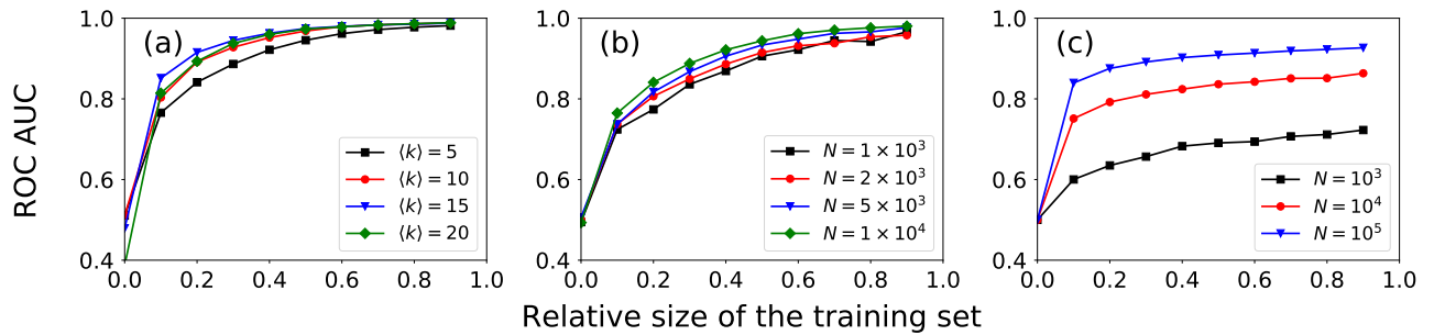
FIG. 6. Reconstruction of synthetic multiplex networks (a) We display the ROC AUC of the degree- and community-based (DC) classifier as a function of the the relative size of the training set. We consider multiplex networks with pre-imposed community structure with size N = 10,000 and power-law degree distribution P(k) \sim k^{-\gamma} , with \gamma = 2.1 . The strength of the community structure is determined by the mixing parameter \mu = 0.1 . Communities have size obeying a power-law distribution with exponent \tau = 1.0 . Different curves represent different values of average degree \langle k \rangle . Maximum degree is k_{\max} = \sqrt{N} . (b) Same as in panel (a), but for networks with average degree \langle k \rangle = 5 . Different curves are obtained for different N values. (c) We display the ROC AUC of the degree-based (D) classifier as a function of the the relative size of the training set. Networks generated according to the configuration model with \gamma = 2.1 , k_{\min} = 3 , and k_{\max} = \sqrt{N} . Different curves are obtained for different N values.
