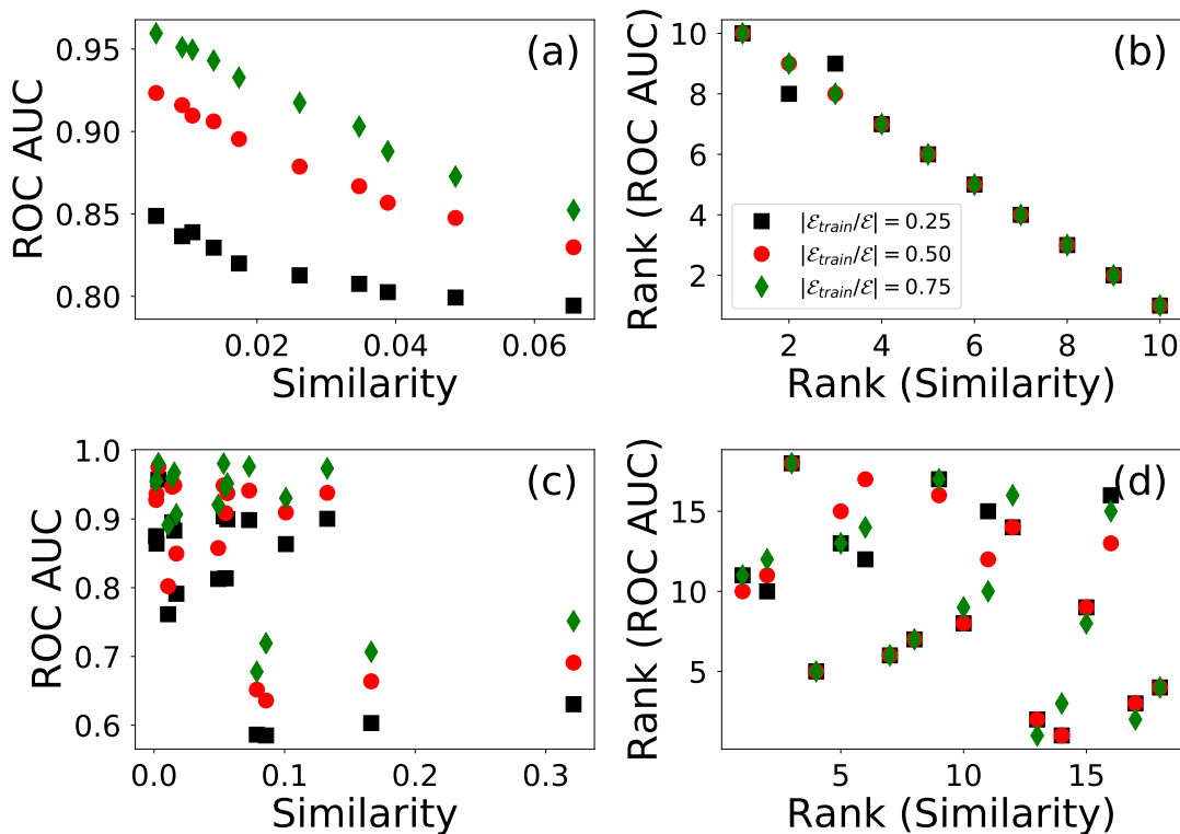
FIG. 9. Sensitivity analysis in the reconstruction of multiplex networks with edge overlap. (a) We consider Lancichinetti-Fortunato-Radicchi (LFR) multiplex networks with N = 10,000 nodes, average degree \langle k \rangle = 10 , degree exponent \gamma = 2.1 , maximum degree k_{\max} = \sqrt{N} = 100 , community distribution exponent \tau = 1 , mixing parameter \mu = 0.1 , and minimum size of the communities c_{\min} = 10 . The two layers are initially identical, then nodes of one of the layers are relabeled with probability q to control for the amount of shared edges. For q = 0 , the two layers share all edges; for q = 1 , the fraction of edges shared become minimal. We consider various values of the relabeling probability q . We report the values of the ROC AUC obtained by using our DC classifier as a function of the Jaccard similarity index of the set of edges of the two layers, i.e., J = |\mathcal{E}^{(\alpha, \beta)}| / (|\mathcal{E}^{(\alpha)}| + |\mathcal{E}^{(\beta)}| + |\mathcal{E}^{(\alpha, \beta)}|) . The different curves correspond to different choices of the relative size of the training set |\mathcal{E}_{\text{train}}|/|\mathcal{E}| , namely (i) |\mathcal{E}_{\text{train}}|/|\mathcal{E}| = 0.25 , (ii) |\mathcal{E}_{\text{train}}|/|\mathcal{E}| = 0.50 , and (iii) |\mathcal{E}_{\text{train}}|/|\mathcal{E}| = 0.75 , where \mathcal{E} = \mathcal{E}^{(\alpha)} \cup \mathcal{E}^{(\beta)} . We perform linear regression of the data points, and obtain the following values of the Pearson's correlation coefficient ( p -value): (i) \rho = -0.93(0.00) , (ii) \rho = -0.99(0.00) , (iii) \rho = -0.99(0.00) . (b) Same as in panel (a), but we plot the rank position of the data according to the two metrics. We obtain the following values of the Spearman's correlation coefficient ( p -value): (i) \sigma = -0.99(0.00) , (ii) \sigma = -1.00(0.00) , (iii) \sigma = -1.00(0.00) . (c) Same as in panel (a), but for the real-world multiplex networks of Fig. 8. We measure: (i) \rho = -0.54(0.02) , (ii) \rho = -0.55(0.02) , (iii) \rho = -0.56(0.02) . (d) Same as in panel (b), but for the real-world multiplex networks of Fig. 8. We measure: (i) \sigma = -0.34(0.17) , (ii) \sigma = -0.44(0.07) , (iii) \sigma = -0.42(0.08) .
