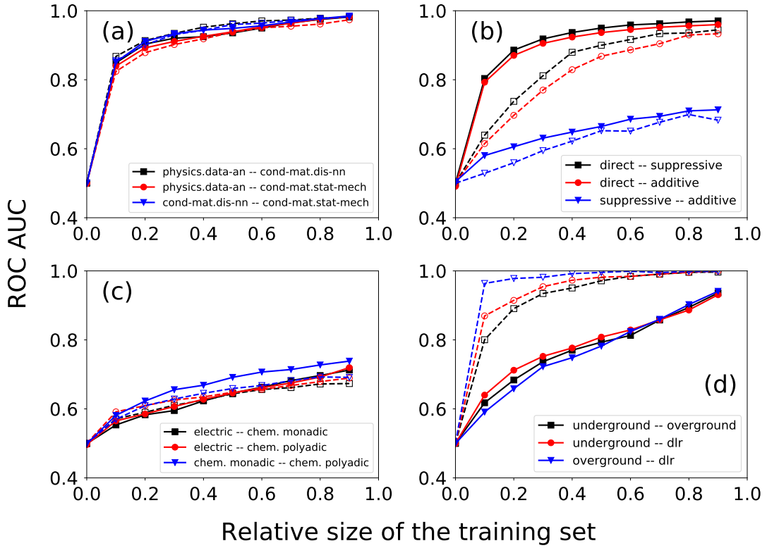
FIG. 4. Reconstruction of real-world multiplex networks. (a) ROC AUC as a function of the relative size of the training set. We report results for the arXiv multiplex collaboration network [39]. We compare the results achieved with the degree- and community-based (DC, filled symbols / full curves) classifier with those of the Wu et al. 's classifier (empty symbols / dashed curves) [30]. Results are averaged over 10 realizations. (b) Same as in panel (a), but for the genetic interactions multiplex network of the Drosophila Melanogaster [40]. Results are averaged over 100 realizations. (c) Same as in panel (a), but for the Caenorhabditis Elegans multiplex connectome [41]. (d) Same as in panel (a), but for the London multiplex transportation network [42]. Results are averaged over 100 realizations.
