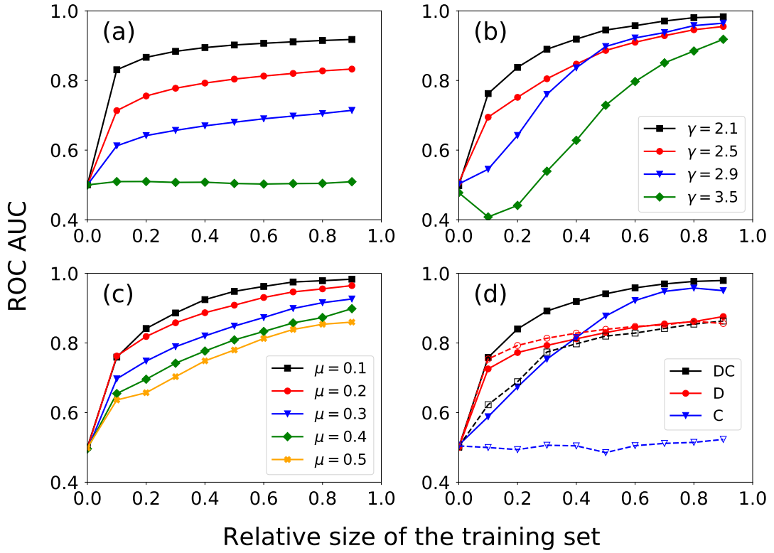
FIG. 2. Reconstruction of synthetic multiplex networks with partial edge information. (a) We plot the performance metric ROC AUC of the degree-based (D) classifier as a function of the relative size of the training set. Multiplex networks have size N = 100,000 and power-law degree distribution P(k) \sim k^{-\gamma} . We display results for different \gamma values. We impose minimum degree k_{\min} = 3 for all \gamma values, while the maximum degree is k_{\max} = \sqrt{N} for \gamma \leq 3 and k_{\max} = N^{1/(\gamma-1)} for \gamma > 3 . The degree sequences of the layers are uncorrelated. (b) We plot the ROC AUC of the degree- and community-based (DC) classifier as a function of the relative size of the training set. Tests are performed on synthetic multiplex networks with pre-imposed community structure constructed according to the LFR model with N = 10,000 , \langle k \rangle = 5.0 , and k_{\max} = \sqrt{N} for \gamma \leq 3 and k_{\max} = N^{1/(\gamma-1)} for \gamma > 3 . Community power-law exponent is \tau = 1.0 , and mixing parameter is \mu = 0.1 . The degree sequences and community structures of the layers are uncorrelated. (c) Same as in (b), but for fixed degree exponent \gamma = 2.1 and different \mu values. (d) We compare the performance of the different classifiers on synthetic graph with built-in community structure (filled symbols / full curves) and without community structure (empty symbols / dashed curves). We plot the performance metric of the DC classifier, the D classifier and the community-based (C) classifier. Graphs with community structure are constructed using the LFR multiplex model with N = 10,000 , \gamma = 2.1 , k_{\max} = \sqrt{N} , \langle k \rangle = 5.0 , \tau = 1.0 , and \mu = 0.1 . We use the configuration model with N = 10,000 , \gamma = 2.1 , k_{\min} = 3 , k_{\max} = \sqrt{N} for the graphs with no community structure. The degree sequences and community structures of the layers are uncorrelated.
