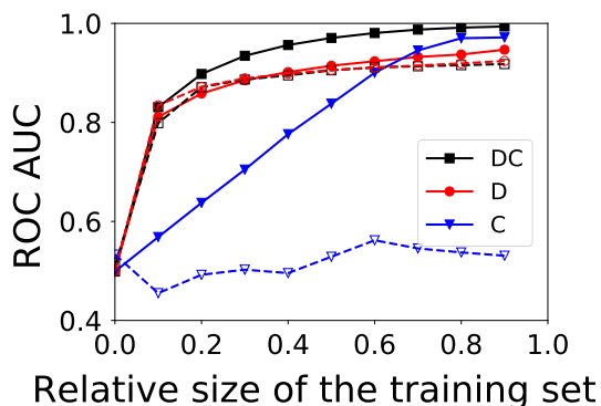
FIG. 5. Reconstruction of synthetic multiplex networks with partial edge information. The figure is the analogue of Fig. 4d, but for networks of larger size. We compare the performance of the different classifiers on synthetic graph with built-in community structure (filled symbols / full curves) and without community structure (empty symbols / dashed curves). We plot the performance metric of the degree- and community-based (DC) classifier, the degree-based (D) classifier and the community-based (C) classifier. Graphs with community structure are constructed using the LFR multiplex model with N = 100,000 , \gamma = 2.1 , k_{\max} = \sqrt{N} , \langle k \rangle = 6 , \tau = 1.0 , and \mu = 0.1 . We use the configuration model with N = 100,000 , \gamma = 2.1 , k_{\min} = 3 , k_{\max} = \sqrt{N} for the graphs with no community structure. The degree sequences and community structures of the layers are uncorrelated.
