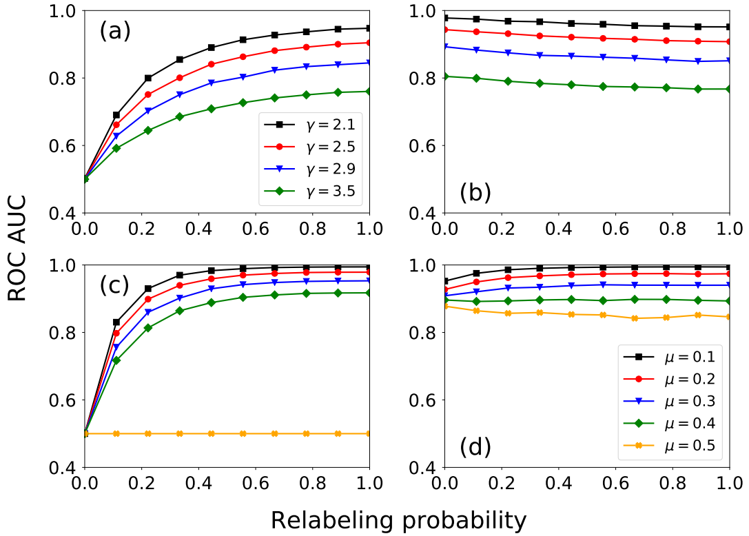
FIG. 1. Reconstruction of synthetic multiplex networks. (a) We consider random multiplex networks with power-law degree distribution P(k) \sim k^{-\gamma} composed of N = 100,000 nodes. Minimum degree is k_{\min} = 3 ; maximum degree is k_{\max} = \sqrt{N} if \gamma \leq 3 , and k_{\max} = N^{1/(\gamma-1)} if \gamma \geq 3 . Different curves are obtained for different \gamma values. We plot the classification metric ROC AUC of the degree-based (D) classifier as a function of the probability relabeling nodes; we relabel nodes to control for degree-degree correlation (see Methods). Degrees are positively correlated when the relabeling probability is zero; they become progressively uncorrelated as the relabeling probability increases. Results are obtained over a single realization of the model. We do not observe substantial fluctuations from run to run. (b) Same as in panel (a), but for multiplex networks with anti-correlated degree sequences. The sequences are maximally anti-correlated for a null relabeling probability, and they become uncorrelated as the relabeling probability increases. (c) We consider the multiplex networks with pre-imposed community structure and power-law degree distribution P(k) \sim k^{-\gamma} . Graphs with N = 10,000 nodes are generated according to the Lancichinetti-Fortunato-Radicchi (LFR) model, see Methods for details. We set degree exponent \gamma = 2.1 , maximum degree k_{\max} = \sqrt{N} , and average degree \langle k \rangle = 20 . Communities have size obeying a power-law distribution with exponent \tau = 1.0 . The strength of the community structure is determined by the mixing parameter \mu . We plot the ROC AUC of the community-based (C) classifier as a function of the probability relabeling the nodes of the multiplex. The classifier is unaware of the ground-truth degree sequences of the network layers. Different curves are obtained for different values of the mixing parameter \mu controlling for the strength of the community structure of the network layers. The community structure of the two layers is correlated when no nodes are relabeled; correlation decreases as the relabeling probability increases. (d) We plot the ROC AUC of the degree- and community-based (DC) classifier as a function of the relabeling probability for synthetic multiplex networks with pre-imposed community structure. The networks are the same networks as in panel (c). In this case, however, the classifier takes also advantage of the knowledge of the ground-truth degree sequence of the network layers.
