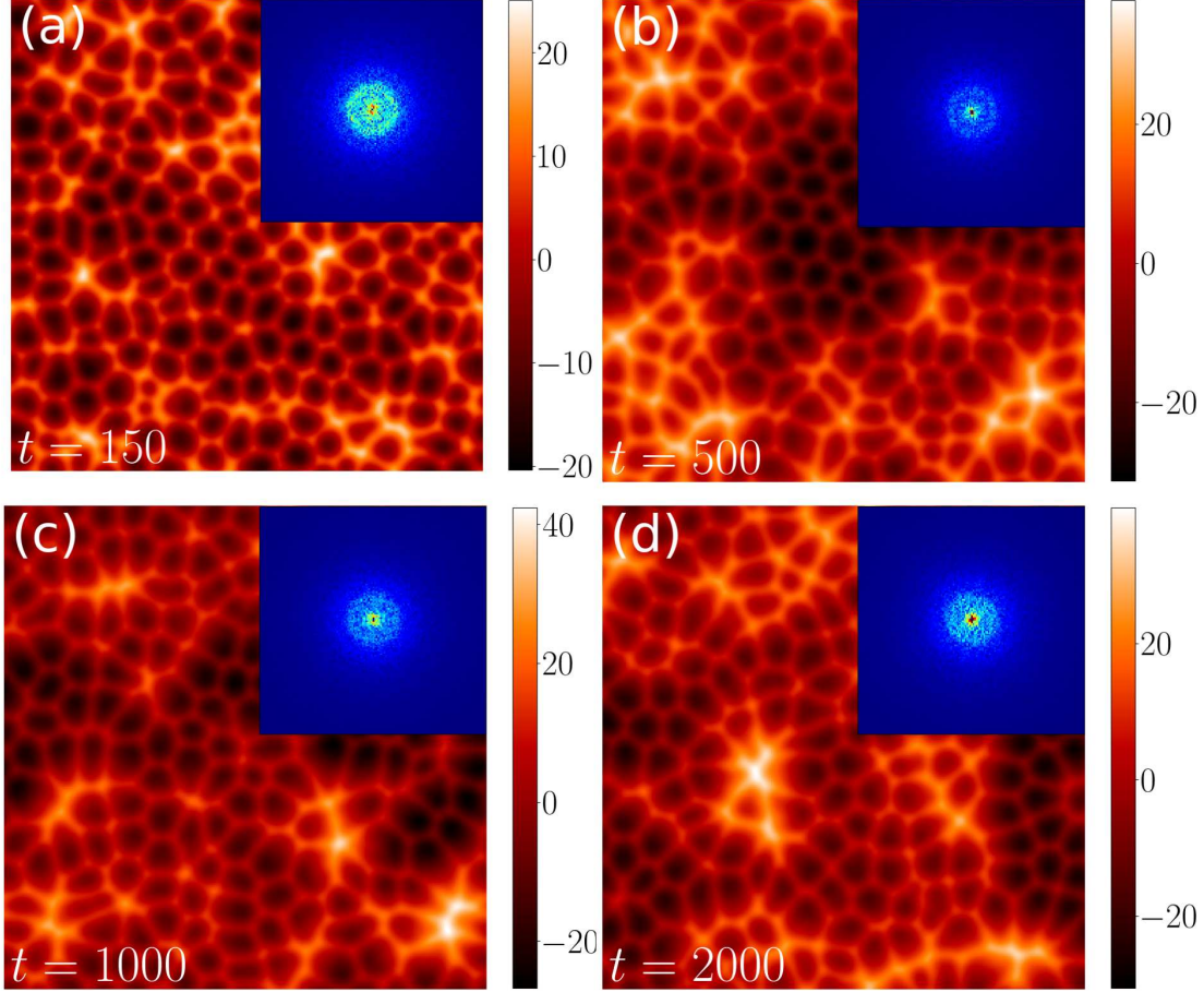
FIG. 11. Results from a simulation of Eq. (51) with \lambda = -0.2 , r = 0 and \nu = 0.05 starting from a low amplitude spatial white noise initial condition. The surface height with the PSD in the insets is shown at times (a) t = 150 , (b) t = 500 , (c) t = 1000 and (d) t = 2000 .
