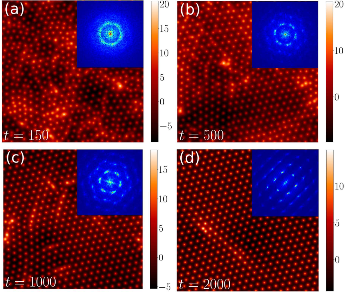
FIG. 7. Results from a simulation of Eq. (50) with \lambda = -0.2 , r = 0 and \nu = 0.05 starting from a low amplitude spatial white noise initial condition. The surface height with the PSD in the insets is shown at times (a) t = 150 , (b) t = 500 , (c) t = 1000 and (d) t = 2000 .
