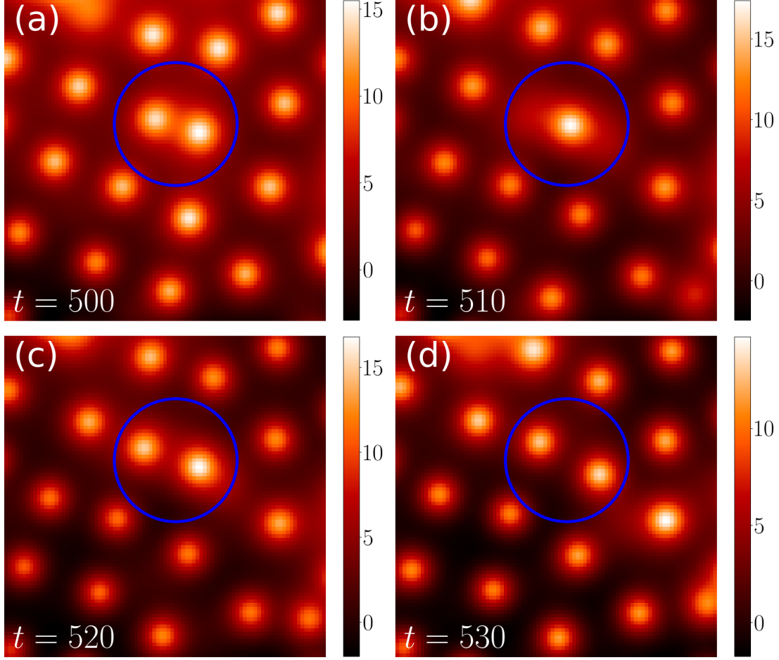
FIG. 10. A zoomed in view of a simulation with the same parameters used in Fig. 7. The plotted domain has a side length of 32.8. The surface height is shown at times (a) t = 500 , (b) t = 510 , (c) t = 520 and (d) t = 530 . Blue circles are included to indicate the region of interest. Two nanodots merge into one between (a) and (b). This nanodot then splits into two between (b) and (c).
