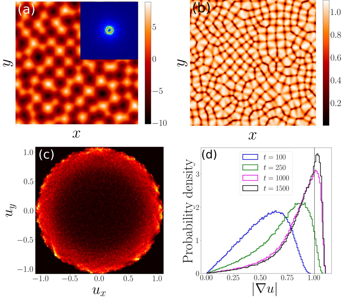
FIG. 1. Results from a simulation of Eq. (51) with \lambda = r = 0 and \nu = 1 starting with a low amplitude spatial white noise initial condition. The surface height at time t = 1000 is shown in (a), along with its power spectral density in the inset. Panel (b) shows the magnitude of the gradient of the surface shown in (a). In (c), the 2D gradient distribution is plotted for the surface shown in (a). Figure (d) shows the probability distribution of the gradient's magnitude at three different times: t = 100 in blue, t = 250 in green, t = 1000 in magenta and t = 1500 in black. The simulation parameters were N = 512 and L = 30\pi .
