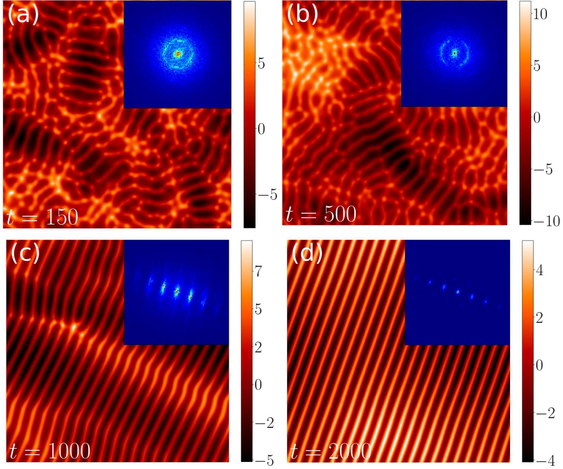
FIG. 15. Results from a simulation of Eq. (50) with \lambda = -0.55 , r = 0 and \nu = 0.05 starting from a low amplitude spatial white noise initial condition. The surface height with the PSD in the insets is shown at times (a) t = 150 , (b) t = 500 , (c) t = 1000 and (d) t = 2000 .
