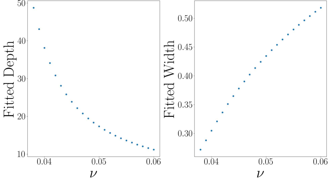
FIG. 4. Values of the (a) depth and (b) width of the Gaussian fits to the u_{xx} profile along a line passing through a spike for small values of \nu . These results were obtained from simulations of Eq. (50) starting with a low amplitude noise initial condition for the parameter values \lambda = r = 0 , the same values used in Fig. 3. The data displayed are for time t = 2000 . For these simulations, N = 256 and L = 5\pi .
