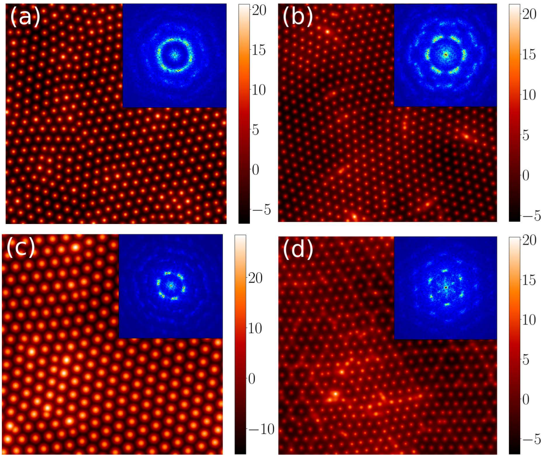
FIG. 13. Results from four simulations of Eq. (50) with different values of \lambda , r and \nu at time t = 2000 . The parameter values used were (a) \lambda = -0.1 , r = 0 and \nu = 0.05 ; (b) \lambda = -0.2 , r = 0 and \nu = 0.04 ; (c) \lambda = -0.2 , r = 0.3 and \nu = 0.04 ; and (d) \lambda = -0.2 , r = -0.05 and \nu = 0.04 .
