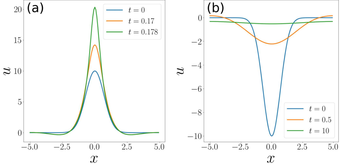
FIG. 2. u(x, 0, t) versus x for two simulations of Eq. (61) at three different times. In (a), the initial condition was an upright Gaussian of height 10 and width \sigma = 1 . Blue is time t = 0 ; orange is t = 0.17 ; and green is t = 0.178 . In (b), the initial condition was an inverted Gaussian of depth 10 and width \sigma = 1 . Blue is time t = 0 ; orange is t = 0.5 ; and green is t = 10 . The simulation parameters were L = 5 , N = 128 and \Delta t = 0.0001 .
