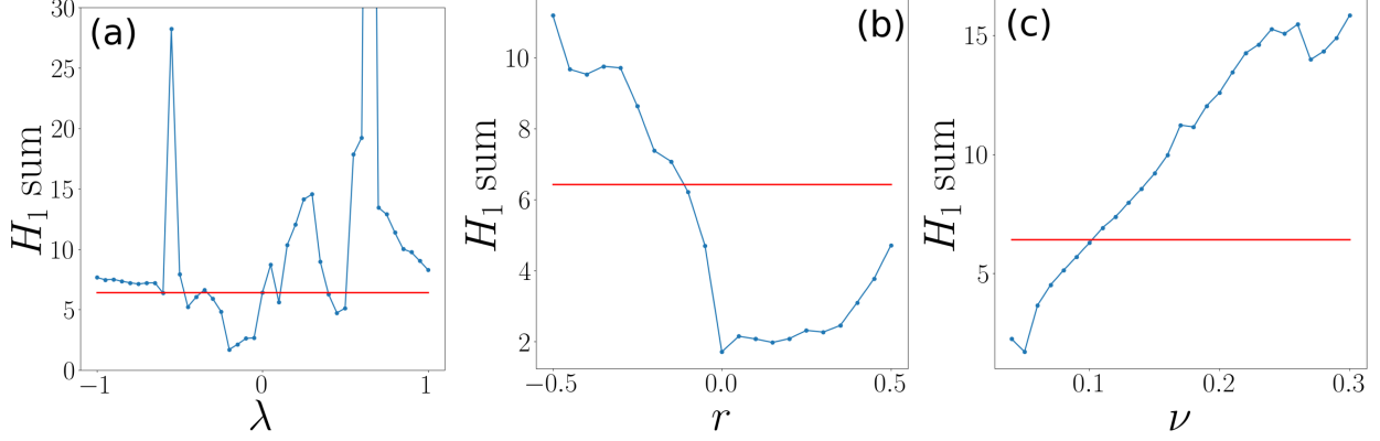
FIG. 14. Normalized H_1 values averaged over times t = 1900 to t = 2000 for simulations of Eq. (50) in which the three parameters were varied separately. In (a), the values r = 0 and \nu = 0.05 were fixed while \lambda ranged from -1 to 1. In (b), the values \lambda = -0.2 and \nu = 0.05 were fixed while r ranged from -0.5 to 0.5. In (c), the values \lambda = -0.2 and r = 0 were fixed while \nu ranged from 0.04 to 0.3. The red horizontal lines correspond to the normalized H_1 sum for simulations with r = \lambda = 0 and \nu = 0.05 .
