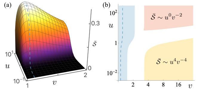
FIG. 4. (a) 3D plot of the universal scaling function for the correlation function \bar{\mathcal{S}}(u, v) , for undamped fluids near RP. The blue dashed line corresponds to the rescaled frequency v^* (the boson peak) at which \bar{\mathcal{S}}(u, v) is maximum for fixed rescaled wavevector u . (b) u \times v diagram showing the boson peak (blue dashed line) and power law regions for which \mathcal{S}(u, v) \propto u^\alpha v^\beta , with (\alpha, \beta) close to their asymptotic values (0, -2) (red) and (4, -4) (yellow). In the blue region the condition \bar{\mathcal{S}}(u, v) > \bar{\mathcal{S}}(u, v^*)/2 is satisfied.
