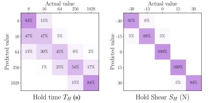
FIG. 4. Experimentally controlled parameters can be extracted from the contact distribution. The percentage of actual and predicted S_H and T_H for block #2. Other blocks show qualitatively similar results.
