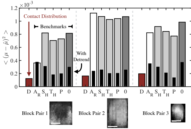
FIG. 3. Contact Distribution Encodes Frictional Strength Test-set mean squared prediction error for three distinct block pairs. Our linear regression method using the spatial distribution of contact ( D ) is compared with four methods using global variables. Prediction error for a linear fit to the total area of contact ( A_R , Eq 3) is shown in white. The errors of optimal experimental predictors (Eq. (4)) using hold time T_H , hold shear S_H , and both parameters ( P ) are shown in light gray. Error from predicting the mean value ( 0 , Eq 5) is shown in dark gray. Thin black bars indicate error when using these benchmark methods on \mu with the slow trend from wear removed as described in text. 10 \times 10 max-pooled example images from each block pair are shown below prediction errors, to scale with one another. Scale bars are 5mm.
