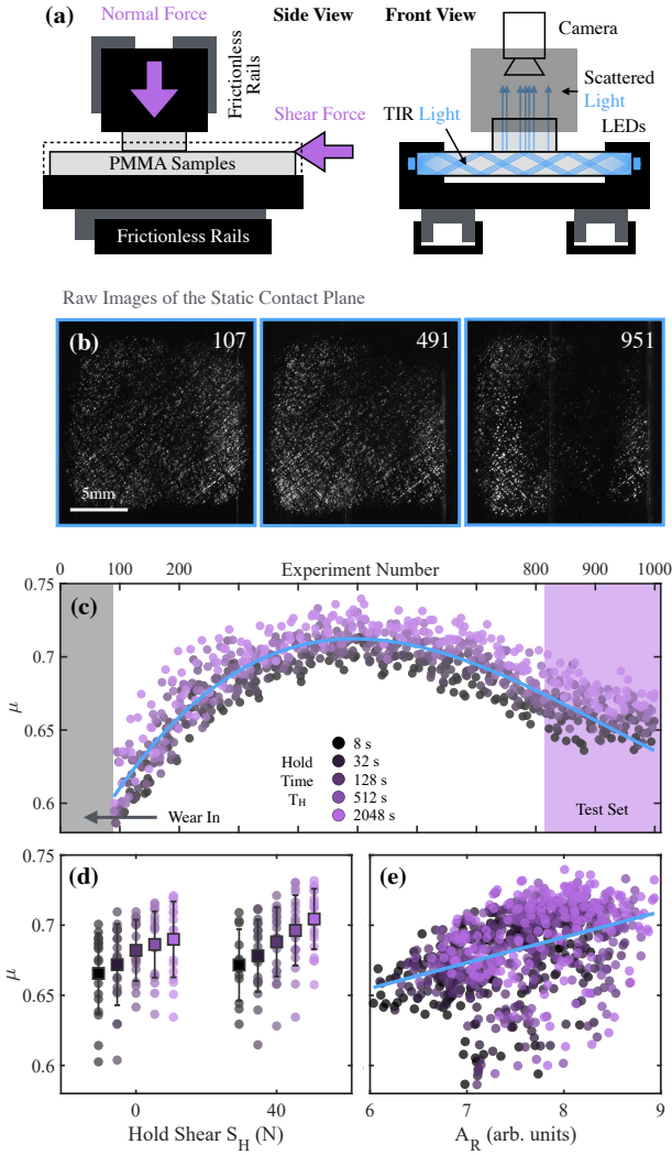
FIG. 1. Experimental Setup and Benchmark Parameters a) Left: Schematic of the biaxial compression/translation stage. Right: Embedded optical setup to image the contact ensemble. b) Three typical images of interfacial contact for after a few dozen, a few hundred, and nearly one thousand experiments, respectively. All data in (b-e) is for block pair 1. c) \mu vs experiment number. Colors (shading) in (c-e) indicate experimental parameter hold time T_H . The final 18% of data, indicated with shading on the right, is to be used as the test set for predictions. d) \mu for the highest (40N) and lowest (0N) hold shears S_H for block pair 1, separated and color (shade) once again represents hold time. Circles are individual experiments, squares are means and error bars are standard deviations for unique (S_H, T_H) pairs. e) \mu as a function of real area of contact A_R (sum of image intensities). Solid line is a linear fit to all data, cf. (3)
