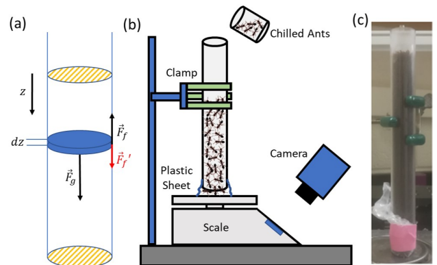
FIG. 1. (a) One of the horizontal slices used to obtain m_{app} in Janssen's model; \vec{F}_f is a supportive friction force, \vec{F}_g is the gravitational force, and \vec{F}_f' is the random force used in our simulations. (b) Schematic of the experimental set up. (c) Image of a fully loaded cylinder at the end of an incremental experiment.
