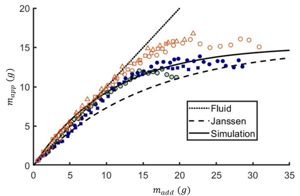
FIG. 2. Apparent mass m_{app} vs added mass m_{add} increases. Differently shaded points are results from trials with ants from different colonies.
