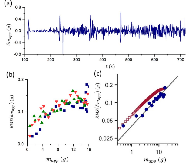
FIG. 4. (a) Fluctuations in the apparent mass as a function of time in a representative experiment. (b) Root-mean-square (RMS) fluctuations as a function of apparent mass for 3 experiments using ants from the same colony. (c) Binned average of the experimental RMS fluctuations of m_{app} (closed circles) and simulated RMS fluctuations of m_{app} (open squares) as a function of m_{app} . The black line corresponds to \sim m_{app}^{1/2} .
