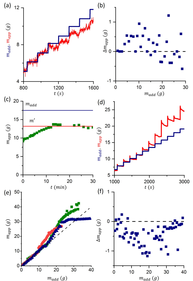
FIG. 3. (a) Added (stepping line) and apparent (fluctuating line) masses of the ants during a portion of a representative experiment in the region where departure from fluid-like behavior begins. (b) The change in the apparent mass over the first 60s after a new addition of mass. (c) Time dependence of the apparent mass in an experiment in which 17.5g of ants were added at once at t = 0 . The horizontal line labeled m' shows the apparent mass measured in the incremental experiment for the same m_{add} . The upper horizontal line corresponds to m_{add} . (d) Added (stepping line) and apparent (fluctuating line) masses of passive spherical grains in a representative experiment. (e) m_{app} vs m_{add} for the grains in various experimental realizations. Note the strong overshoot in m_{app} . The dashed line represents fluid behavior. (f) Change in the apparent mass of the passive spheres over the first 60s after a new addition of mass.
