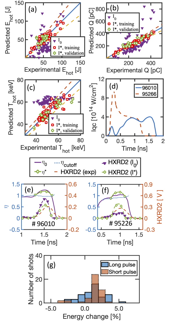
FIG. 2. (Color Online) (a) Predicted E_{hot} versus the experimental data. (b) Predicted Q versus the experimental data. (c) Predicted T_{hot} versus the experimental data. Dashed lines in Fig.(a)-(c) represent the experimental error bars of 22% for E_{hot} , 10% for Q and 9.4% for T_{hot} . In (a)-(c), " I_0 " refers to the predictions based on the original LILAC laser intensity and " I^* " refers to the predictions based on the modified laser intensities, with "training" ("validation") refers to the group of shots that were (were not) used in deriving the laser intensity modification. (d) Laser intensity for shot 96010 and 95266. (e) and (f) Predicted and measured time-resolved HXR2 signals and \eta from LILAC ( \eta_0 ) and the modified intensity ( \eta^* ) for Shot 96010 (long pulse) and 95226 (short pulse). We notice I^*/I_0 = \eta^*/\eta_0 . (g) Histogram of laser energy change after modification.
