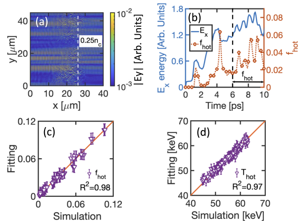
FIG. 1. (Color Online) (a) E_y component for both the laser speckles and TPD plasma waves at 8.0 ps. (b) Typical temporal evolution of hot electron fraction f_{hot} and plasma wave ( E_x ) energy. Plasma conditions for (a) and (b) are L_n = 150\mu\text{m} , I = 2.5 \times 10^{14} \text{ W/cm}^2 , T_e = 2.0 \text{ keV} and T_i = 1.0 \text{ keV} . (c) The fitting quality for the hot electron scaling f_{hot} , Eq.(1). (d) The fitting quality for the hot electron scaling T_{hot} , Eq.(2). Error bars in (c) and (d) show the 95% confidence interval for the fitting. We used nlparci from MATLAB to calculate the 95% confidence interval [33].
