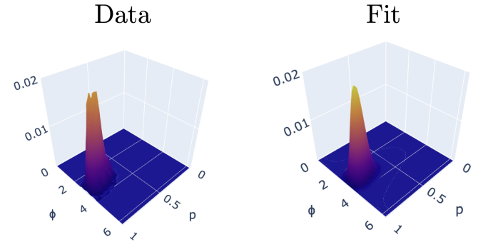
Figure 2. Comparing time-aggregated data of a single trajectory generated by Eq. (15)'s stochastic model (left) to the fit to a geometric canonical ensemble with functional form as in Eq. (9) (right). Here, h(Z) = E(p, \phi) = \delta \langle \sigma_x \rangle + \epsilon \langle \sigma_z \rangle = \delta 2\sqrt{p(1-p)} \cos \phi + \epsilon(1-2p) , with \delta = \epsilon = 1 . The excellent agreement is visually clear, and it is quantified by a total variation distance between the two distributions of f \approx 5.6 \times 10^{-4} .
