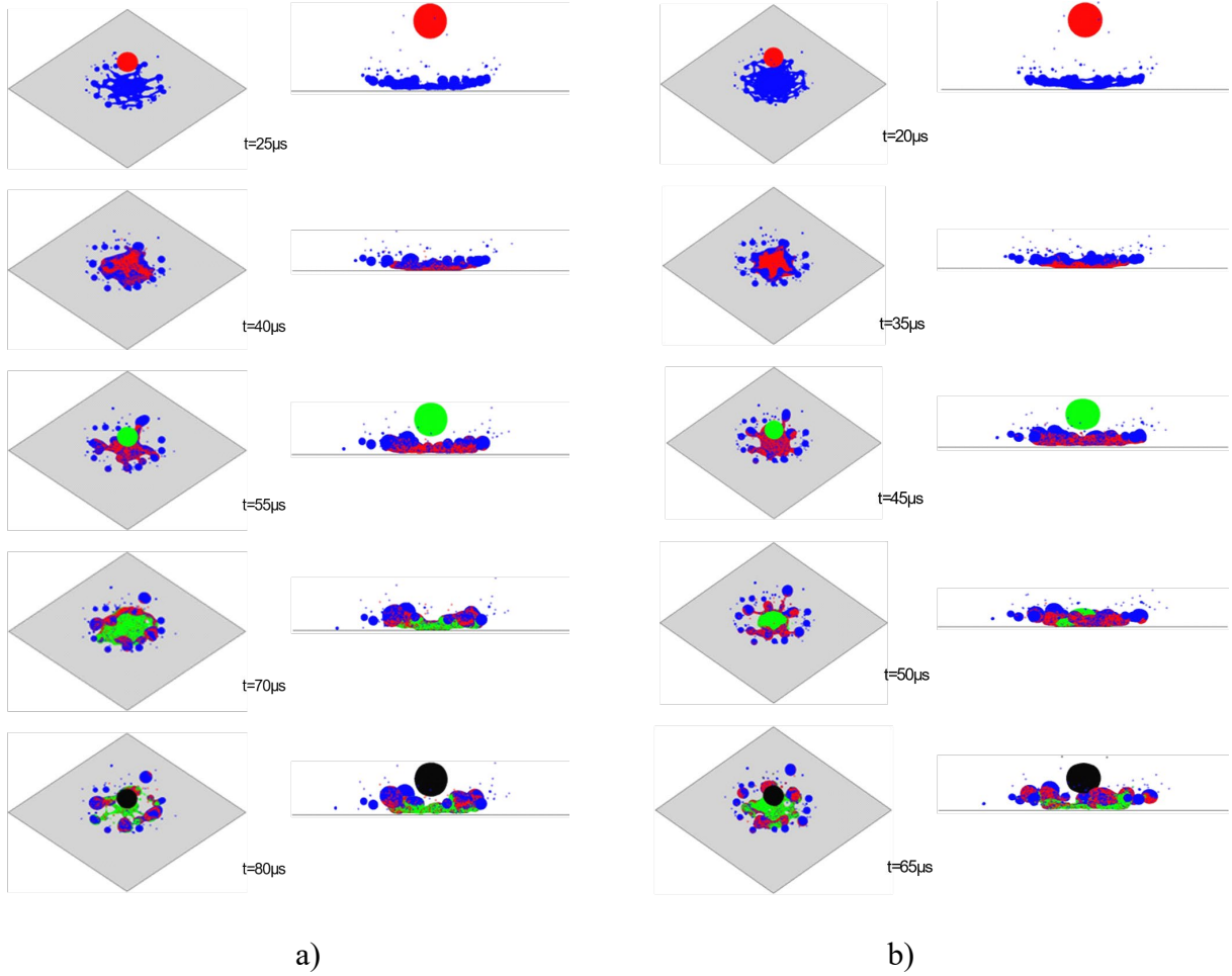
FIG. 5. Post-impingement outcomes at T_w = 600\text{ K} a) f = 40\text{ kHz} b) f = 50\text{ kHz} .
