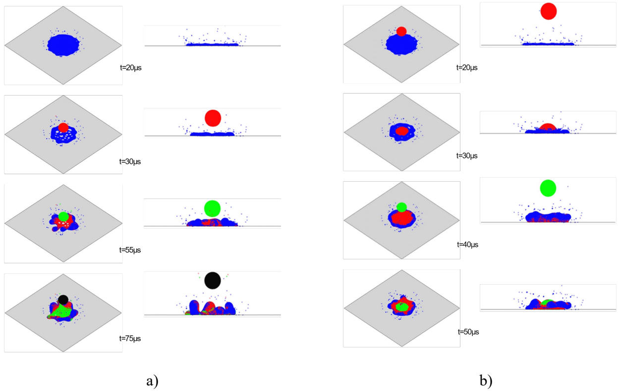
FIG. 3. Post-impingement outcomes at T_w = 420 K a) f = 40 kHz b) f = 50 kHz .
