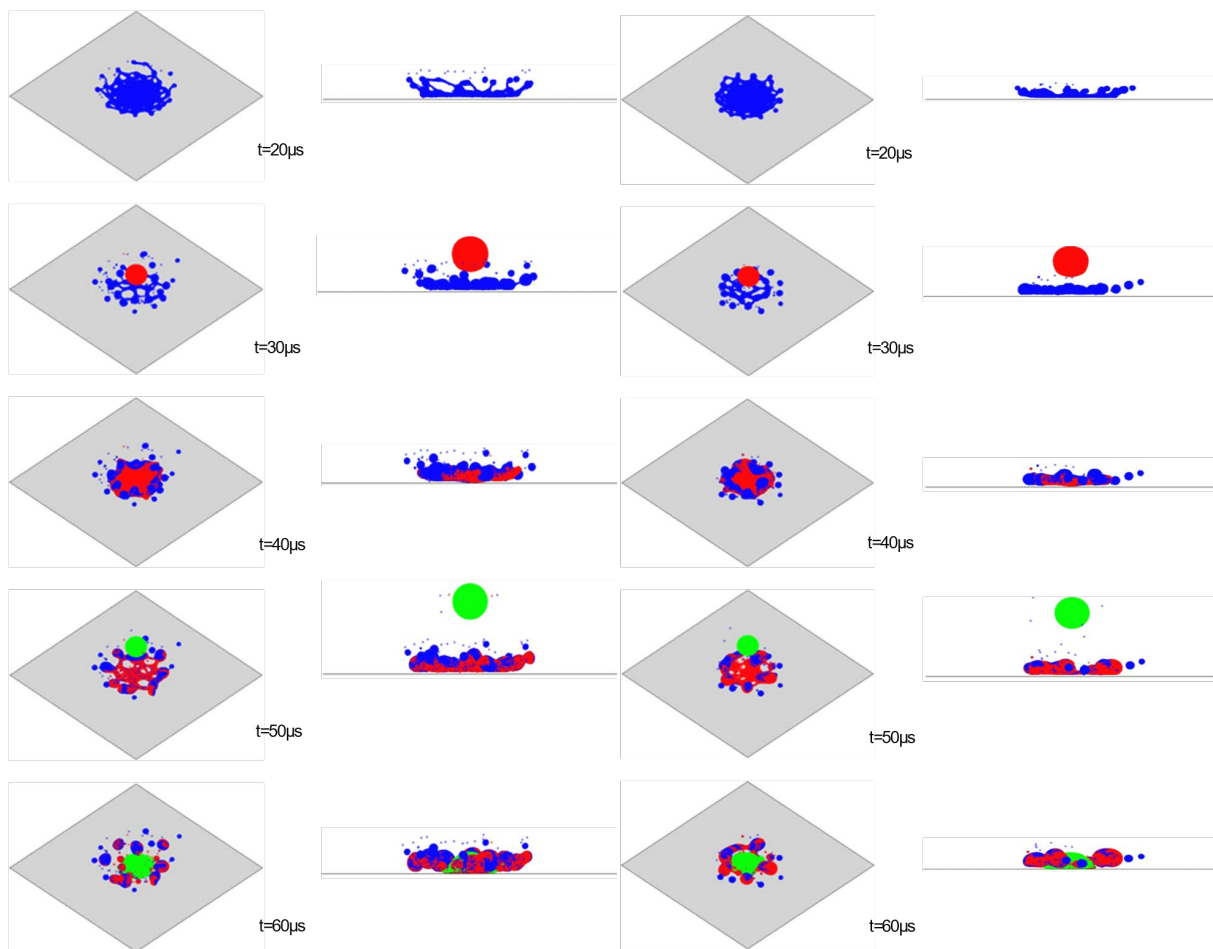
FIG. 7. Post-impingement outcomes at T_w = 600 K and f = 40 kHz a) P = 5 bar b) P = 20 bar .
