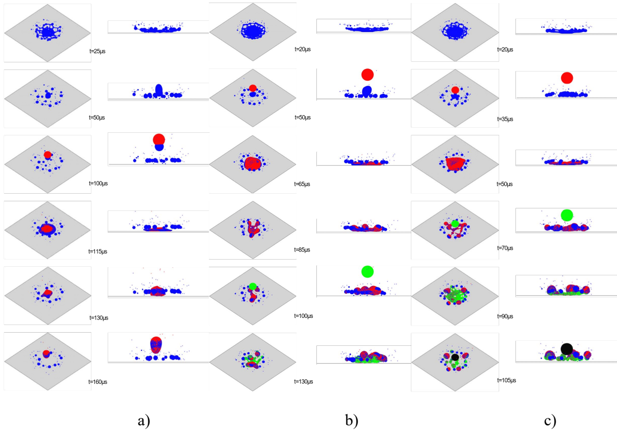
FIG. 4. Post-impingement outcomes at T_w = 600 K a) f = 10 kHz b) f = 20 kHz c) f = 30 kHz .
