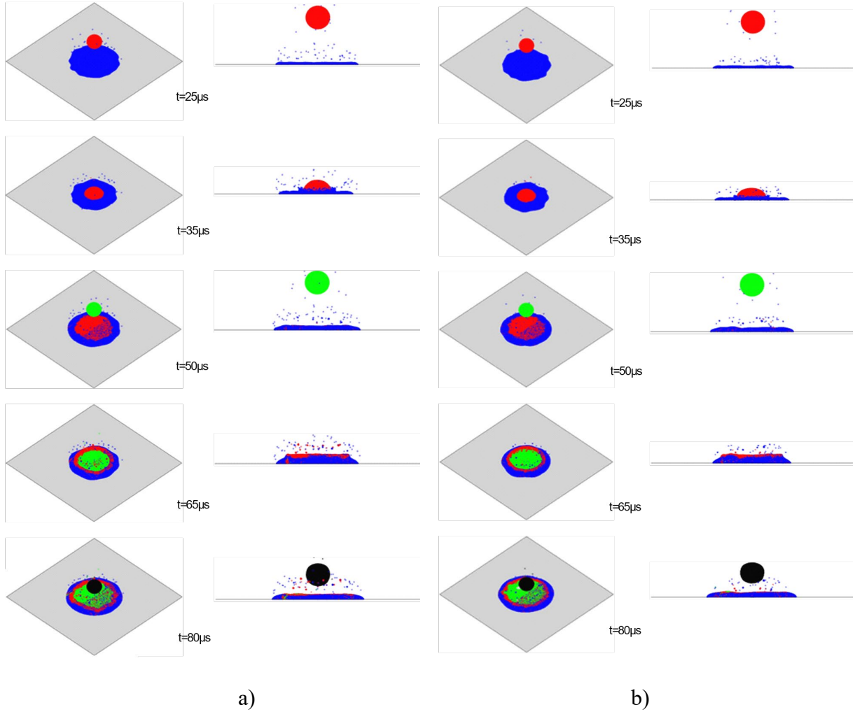
FIG. 6. Post-impingement outcomes at T_w = 420 K and f = 40 kHz a) P = 5 bar b) P = 20 bar .
