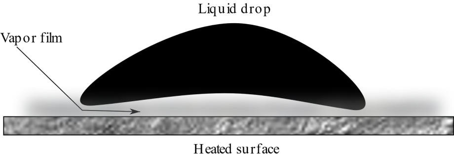
FIG. 1. Schematic of the Leidenfrost phenomenon during drop-wall impact
