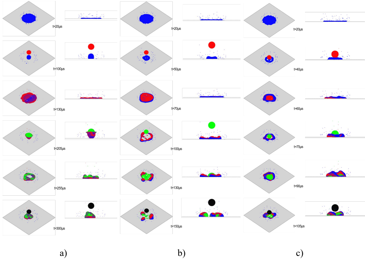
FIG. 2. Post-impingement outcomes at T_w = 420 K a) f = 10 kHz b) f = 20 kHz c) f = 30 kHz .
