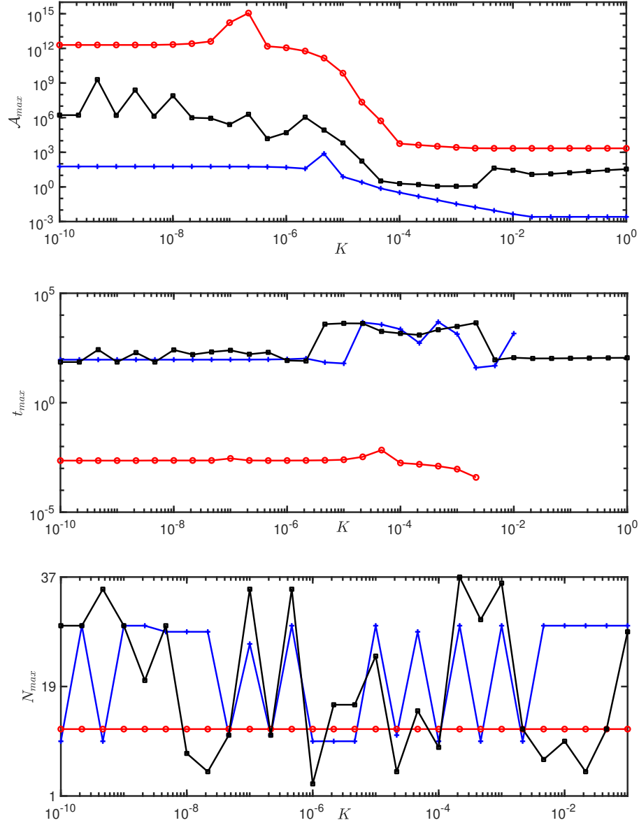
FIG. 11: Same as Fig. 6 but for the amplitude-dependent coupling (8). Red lines with circle markers show results for the single peak initial condition while blue lines with + markers are the results for the sine wave initial condition. The top panel shows the variation in the maximum amplitude of observed excitations (on log scale) as a function of the coupling coefficient K_0 . The middle panel shows the variation in the time taken to reach the maximal excitation t_{max} on log scale, also as a function of K_0 . Finally, the bottom panel shows the variation of the location N_{max} of the maximal amplitude among the individual oscillators as a function of K_0 . Note that the single peak initial conditions were initialised at N = 12 .
