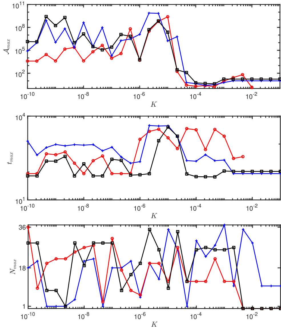
FIG. 6: Red lines with circles show the results for the single peak initial condition, blue lines with crosses show the results for the sine wave initial condition while black lines with square markers show results for the random initial condition. The top panel shows the variation in the maximum amplitude \mathcal{A}_{max} (on log scale) as a function of the diffusion coefficient K . The middle panel shows the time t_{max} taken to reach the maximal excitation, also on log scale, while the bottom panel shows the variation of the location i = N_{max} of that maximal event among the individual oscillators.
