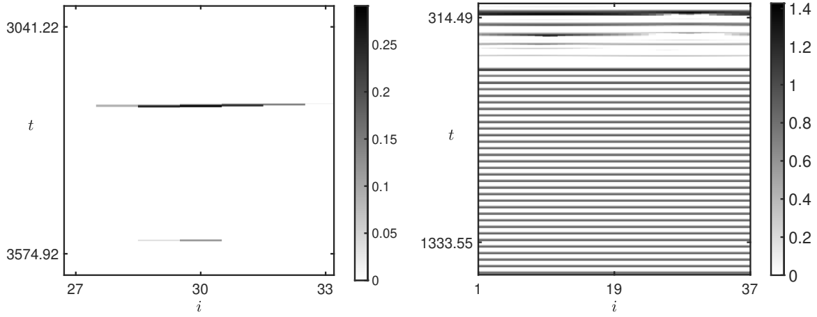
FIG. 4: Space-time plot showing the evolution of \log_{10}(\mathcal{A}_i) starting from a sine initial condition in a system of N = 37 coupled oscillators with K = 1 \times 10^{-4} (left panel), with maximum amplitude occurring at the i = 30 , and K = 2.2 \times 10^{-3} (right panel) with maximum amplitude occurring at i = 10 . The left panel shows that the large amplitude feature is not localized at a single oscillator and that neighboring oscillators respond coherently. In the right panel, all oscillators are synchronized and so oscillate in spatial coherence.
