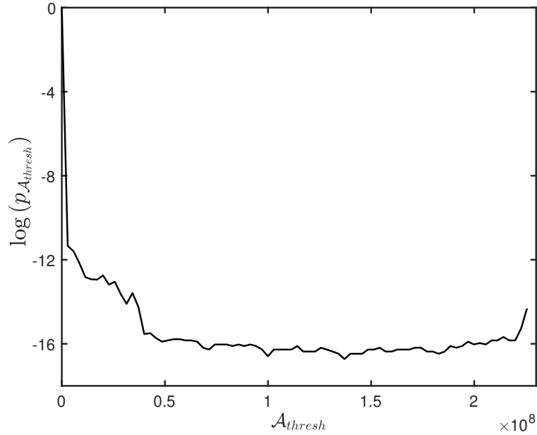
FIG. 5: Logarithm of the probability density function p_{\mathcal{A}_{thresh}} for different amplitude thresholds \mathcal{A}_{thresh} from the time evolution shown in Fig. 2. We observe an increase in the probability of extremely large amplitudes, indicating that the occurrence of extreme events is more probable than what is expected from an exponential distribution of amplitudes.
