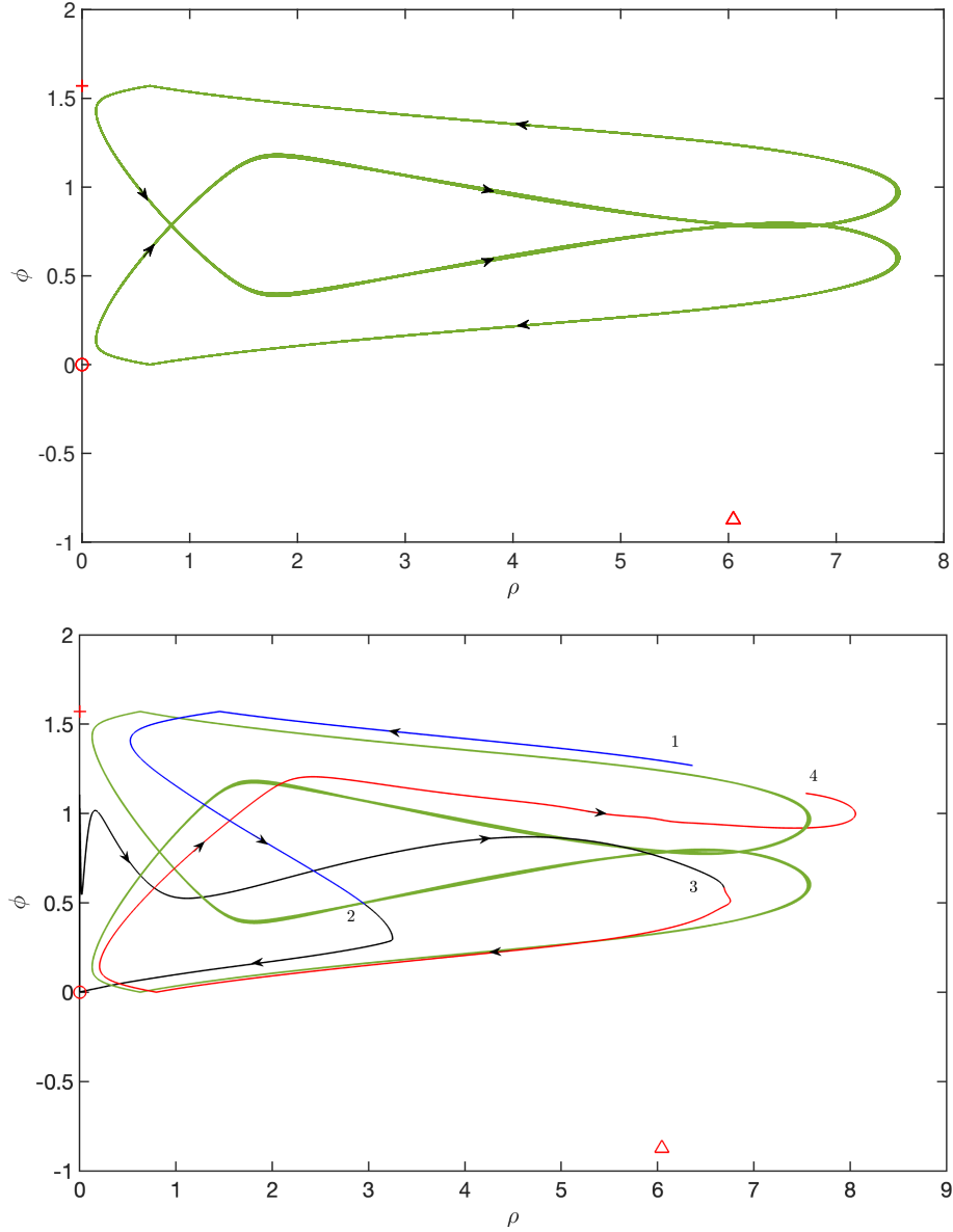
FIG. 10: Top panel: Phase portrait along the (\rho, \phi) plane during regular periodic spiking at a single node in the network with no coupling (green line). Bottom panel: Same view in the (\rho, \phi) plane with superposed evolution close to a large amplitude event at N = N_{max} (black line) in the coupled network with K = 2.1544 \times 10^{-6} , for comparison with Fig. 9.
