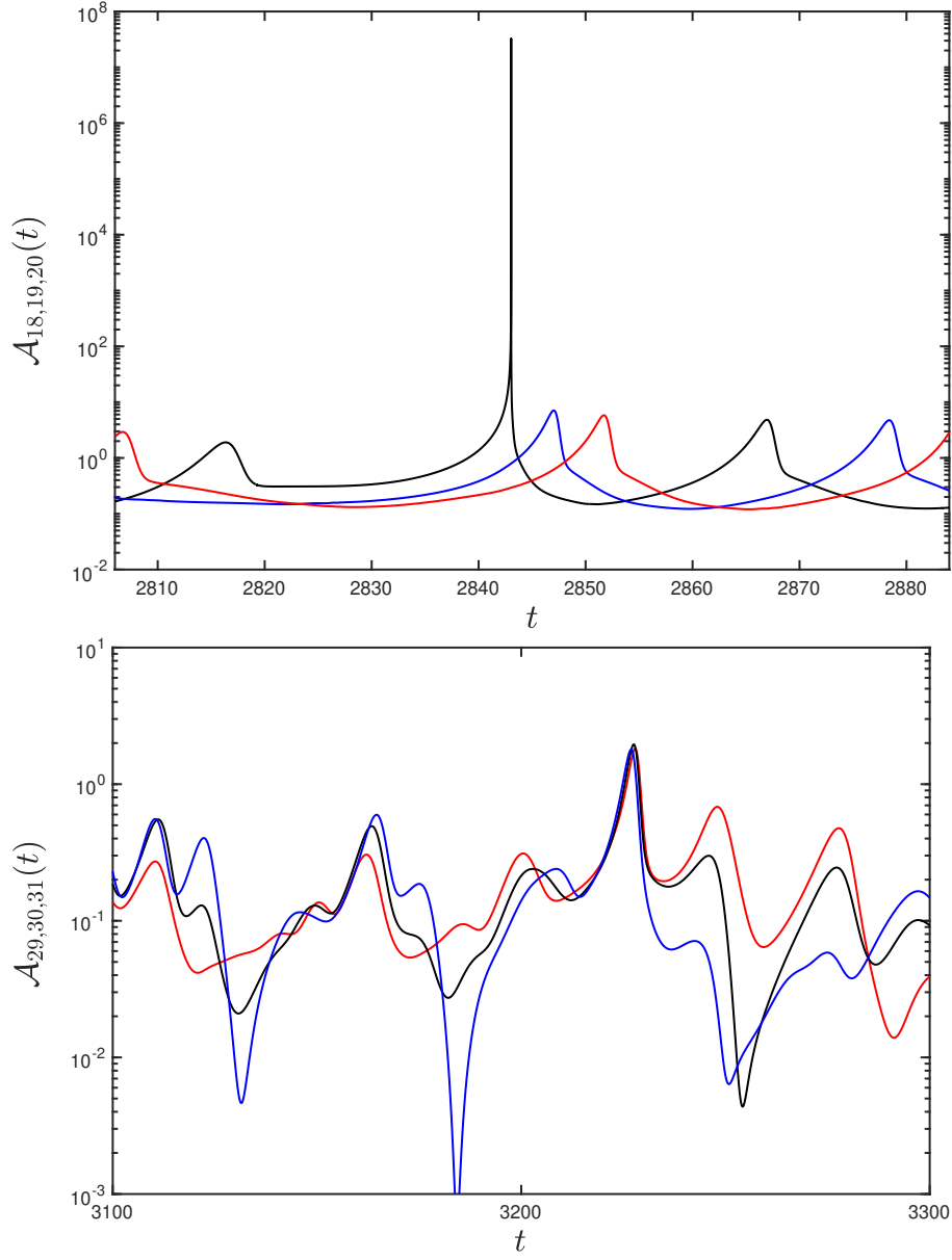
FIG. 3: Top panel: Evolution of large amplitude event at i = 19 (shown as black line) as seen in the right panel of Fig. 2 along with the amplitude evolution of its immediate neighbors at i = 18 (red line) and i = 20 (blue line). Bottom panel: Evolution of large amplitude event at i = 30 (shown as black line) as seen in the left panel of Fig. 4 along with the amplitude evolution of its immediate neighbors at i = 29 (red line) and i = 31 (blue line).
