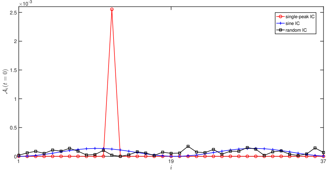
FIG. 1: Three types of initial conditions showing the distribution of initial amplitudes \mathcal{A}_i(t = 0) in a system of N = 37 coupled oscillators. The red line with circle markers shows a single peak initial condition, the blue line with crosses shows a sine wave initial condition and the black line with square markers shows a uniformly distributed random initial condition. In all three cases the Riemann sums pertaining to the 3 curves are equal.
