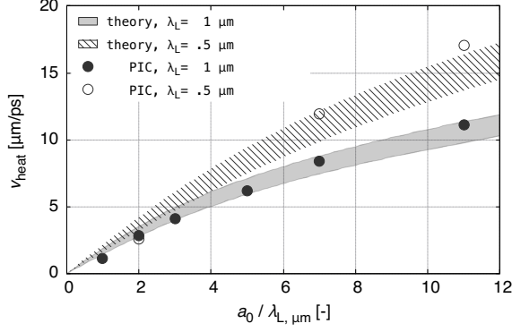
FIG. 4. Fast thermal diffusion speed v_{\text{heat}} versus a_0/\lambda_{L,\mu\text{m}} ( \propto I^{1/2} ). The target parameters were fixed ( n_i = 50 , Z = 10 ). Black dots and white circles represent the simulation results for \lambda_L = 1.0 and 0.5 \mu\text{m} , respectively. The gray shaded area and striped area are v_{\text{heat}} obtained from Eq. (5) with the factor f = 0.065 and the absorption rate \chi_{\text{ab}} = 0.1 – 0.17 for \lambda_L = 1.0 \mu\text{m} and \chi_{\text{ab}} = 0.13 – 0.22 for \lambda_L = 0.5 \mu\text{m} , respectively.
