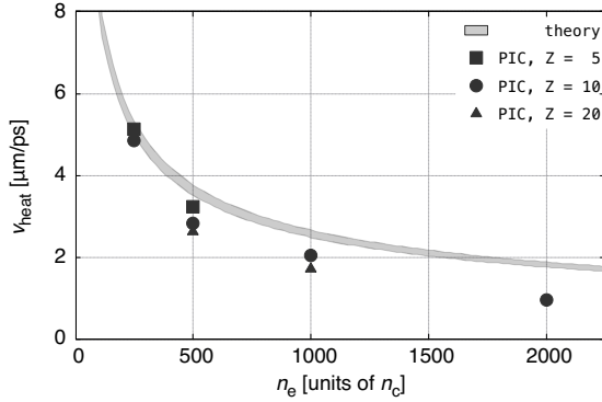
FIG. 5. Fast thermal diffusion speed v_{\text{heat}} versus target electron density n_e when the laser normalized amplitude and the laser wave length are fixed ( a_0 = 2 and \lambda_L = 1.0 ). The black square, circle, and triangle dots represent the simulation results of Z = 5 , 10 , and 20 , respectively. The gray shaded area is the result of the theoretical model with the absorption rate \chi_{\text{ab}} = 0.17 – 0.2 .
