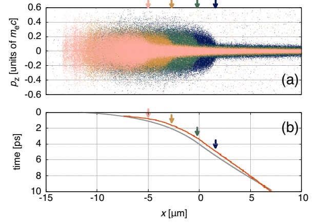
FIG. 3. (a) Temporal evolution of electron phase plot x - p_z for a_0 = 1 , n_i = 50 , Z = 10 , and the pre-plasma scale length 2.56 \mu\text{m} . The arrows indicate the positions of the diffusion front at times t = 0.83 ps (pink), 1.67 ps (yellow), 3.33 ps (green), and 5.0 ps (blue). (b) Trajectory of the fast thermal diffusion front in the time-space diagram. The orange line represents the result of the PIC simulation shown in Fig. 3 (a). It is as same as the orange circles in Fig. 1(b) and the orange line in Fig. 2(b). The gray line represents the numerical solution of Eq. (2) with the factor f = 0.1 . The arrows indicate the observation times in (a).
