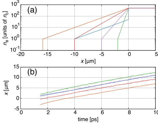
FIG. 2. (a) Initial electron density profile for each case. The scale lengths are 0.32, 0.80, 1.60, and 2.56 \mu\text{m} . The maximum densities of the pre-plasma for the cases with the scale length of 2.56 \mu\text{m} are 50 and 500 n_c . (b) Trajectory of thermal diffusion front in each case. The color of each line corresponds to that shown in Fig. 2(a).
