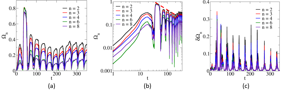
FIG. 9: \Omega_n metrics for the evolving surface patterns during the film growth with contact angle \theta = 51^\circ in both linear scale (a) and log scale (b) with least square linear fitting shown as dashed line. \delta\Omega_n(t) for the system is shown in (c).
