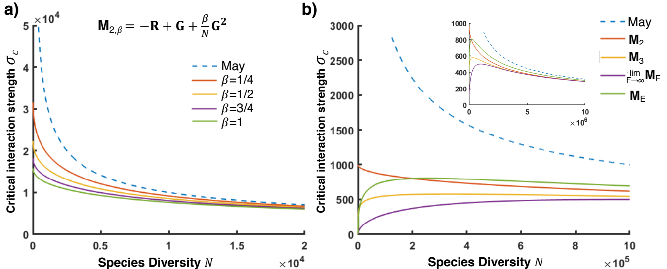
FIG. 2. Non-monotonic stability relationships arise from beyond 3-species correlations
