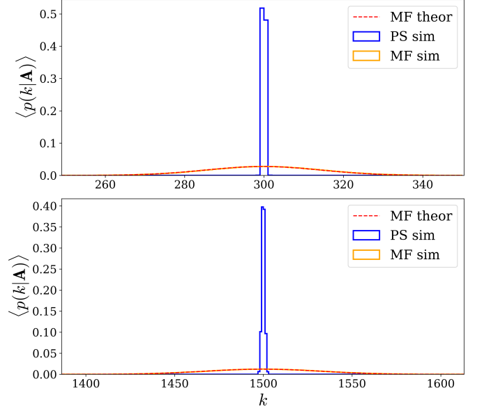
FIG. 7: (Color online). Degree distributions of 3-star and MF models with 1000 ( top panel ) and 5000 ( bottom panel ) nodes for t_1 = 3284.58 , t_2 = -7500 , t_3 = 4500 . The degree distribution of the 3-star model is almost degenerate around dominant degrees. Degree distribution for the MF model follows instead the expression (66).
