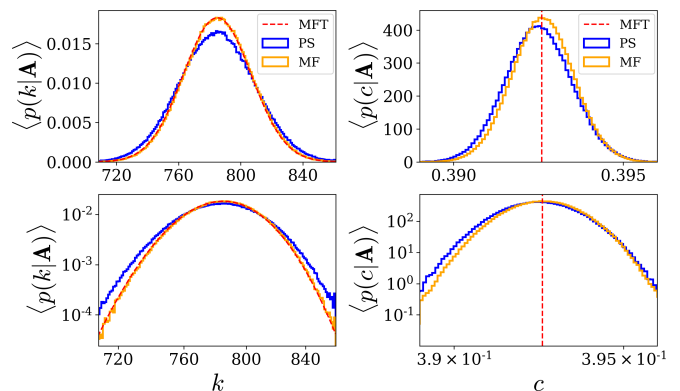
FIG. 9: (Color online). Degree and local clustering coefficient distributions for 3-star and MF models at t_1 = -0.5 , t_2 = 0.3 , t_3 = 0.1 ( top row ) and corresponding log-log plots ( bottom row ). The degree distribution of the MF model is described well by the Gaussian (66) (dashed curve on degree distribution plots). The vertical dashed lines on LCC plots show the position of the average LCC found from (62). Both degree and LCC distributions of the 3-star model in this case are wider than the degree distribution of the corresponding MF model, but the averages match well. Decay is exponential in both cases as shown in log-log plots.
