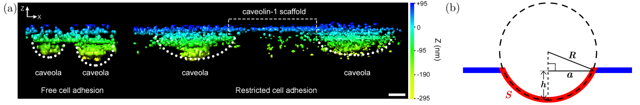
FIG. 1: Cup-shaped caveolae. (a) Two-dimensional z - x rendering of caveolae obtained from three-dimensional superresolution fluorescence imaging of caveolin-1 at the plasma membrane for mouse embryonic fibroblast cells freely adhering to fibronectin substrates (left) and with adhesion constrained to 210 \times 10 \mu\text{m}^2 fibronectin islands (right). Changes in the cell adhesion geometry are expected to modify the cell adhesion forces [22, 23], and the shape and organization of caveolae [14]. The white dotted curves indicate the approximate position of the plasma membrane for the observed caveolae. Scale bar: 100 nm. (Adapted with permission from Ref. [14].) (b) Schematic of the spherical cap model of caveola shape, with the caveola domain indicated in red and the surrounding membrane indicated in blue. We denote the caveola surface area by S = \pi L^2 , the caveola radius of curvature by R , the caveola base radius by a , and the caveola invagination depth by h [24].
