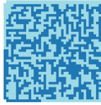
Figure 7: A typical supercritical sample.
