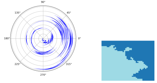
Figure 9: Boundary Slope Plots for \lambda = 1/\mu (critical regime), with population constraints 10%, along with the final state on a 40 \times 40 grid graph. Run for 25,000,000 compressed steps, amounting to 354,337,192,915 proposals, over the course of approximately one month of computing time. The metastable region that was apparent in the subcritical case is not an obstruction here.
