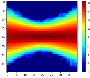
Figure 6: \log(\text{flips} + 1) , after 254 hours (equivalently, 64,054,464,437,342 proposals) on a 40 \times 40 grid graph. pop bounds 5 percent. This is stuck in a bottleneck set; it has not reached the equally probable region around the vertical partition. Loosening either the population constraint or bringing the fugacity closer to the critical value can help mixing.
