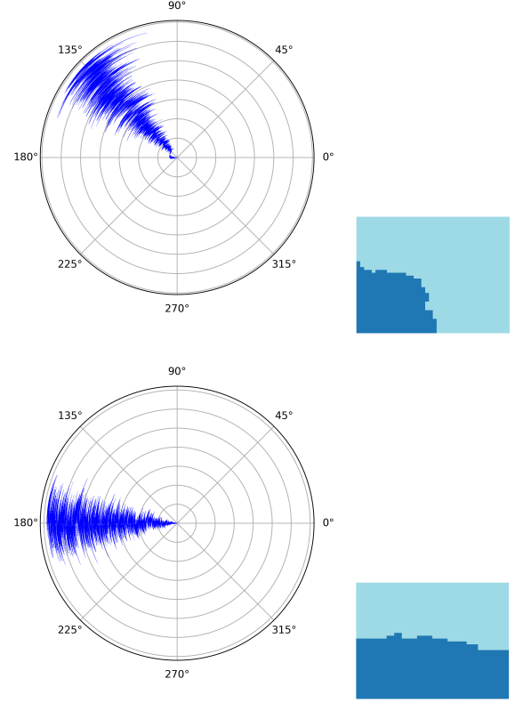
Figure 5: (left) Boundary slope plot and (right) the end state, from a subcritical ( \lambda = \frac{1}{2\mu} = .189\dots ) flip walk constrained to population balance 10 percent (bottom) and 50 percent (top). The top plot was run for 21,000,000 compressed steps, which amounted to 703,328,732,936 proposals, over roughly one month of computing time. The bottom plot was run for 23,000,000 compressed steps, 712,097,053,677 proposals, over the same time period.
