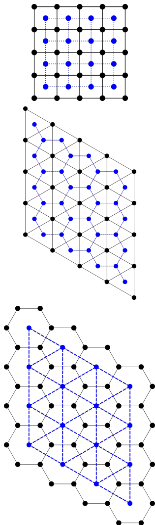
Figure 3: From top to bottom, the 4 \times 4 versions of Squarelandia, Trilandia and Hexlandia in black, displayed with their supernode-deleted duals in blue.
