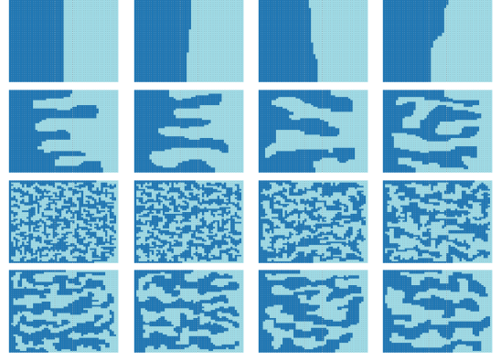
Figure 14: Samples from distributions with energy function e^{-(\gamma_{\text{pop dev}} + \delta \text{boundary length})} with \delta = 1 as \gamma varies from .11 to .81 (top two rows, read left to right) and \gamma = 1 as \delta varies from .11 to .81 (bottom two rows, read left to right). The images in each experiment are snapshots of a single run of the Markov chain.
