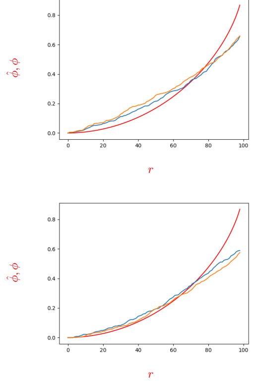
Figure 12: With variable endpoints on a 30 \times 30 (top) and 40 \times 40 (bottom), with N = 501 independent runs starting from the horizontal partition for 1,000,000 steps each. Notation as in fig. 11.
