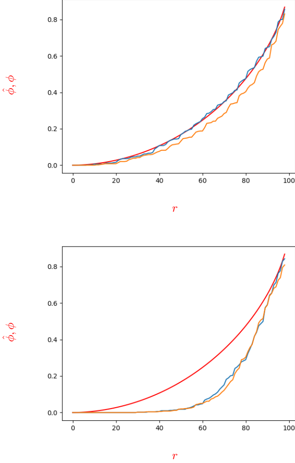
Figure 11: Taking n = 20 (Top) and n = 30 (Bottom), with \gamma_i obtained after 100,000 steps each with N = 500 . Comparing \hat{\phi}(r, x) with \phi(r, x) for x = \pm 1 and r \in \{i/101 : 0 \leq i \leq 99\} . The solid red line is \phi(r, 1) = \phi(r, -1) , and the other two lines are \hat{\phi}(r, 1) and \hat{\phi}(r, -1) . The x -axis is r , and the y -axis is the value of the function. Apparently 100,000 is sufficient for mixing when n = 20 , at least for this statistic, but not when n = 30 .
