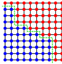
Figure 2: The relationship between connected partitions and self-avoiding walks.
