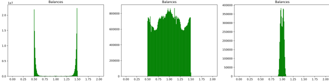
Figure 13: The population balance histogram after running with balance constraints for steps starting from a vertical partition of a 40 \times 40 grid graph. Here, the x -axis represents the balancedness of a block, measured in terms of |A|/h where |A| is the size of a block, and h is exactly half the total population. The y -axis counts the number of times a partition containing a block with that balance was encountered during the run. After normalization, this provides an approximation of the marginal distribution of population balance of the stationary distribution. Since we start with a perfectly balanced partition, we do not include the first 1,000,000 partitions in the histogram, and these figures were obtained after a month of computation. Left is subcritical ( \lambda = 1/2\mu ), middle is critical ( \lambda = 1/\mu ), right is supercritical ( \lambda = 1 ). The balance constraints for the subcritical and supercritical runs are 50 percent, which explains the sharp cutoffs, and the balance constraint for the supercritical run is 100 percent. For the subcritical run, most of the mass is on partitions which are nearly as unbalanced as allowed by the constraints; experiments evaluating softer thresholds on population balance or using simulated tempering could provide additional insight in future work.
