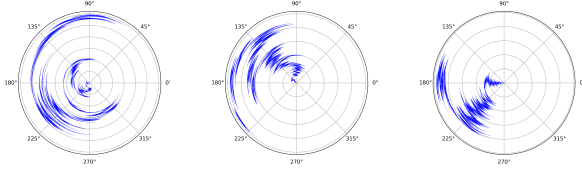
Figure 10: (Left) Setting \lambda = 1/\mu - .3 = .35\dots , population bound at 50% and using a 40 \times 40 grid graph results in a run that looks more like the critical case than the subcritical case. (Middle) The same but \lambda = .32 , (Right) same but \lambda = .29 . Each of these was run for about a week of computing time, which amounted to the order of 250,000,000,000 proposals each.
