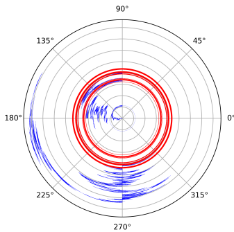
Figure 8: Boundary slope plots (left) for a super critical ( \lambda = 1 ) run with population constraint 100%. The apparent rapid rotation in the beginning of the run was due to the boundary end points ending up near the two corners of one edge. This was run for 11,000,000 compressed steps, or 20,302,926,563 proposals, over the course of one month of computing time.
