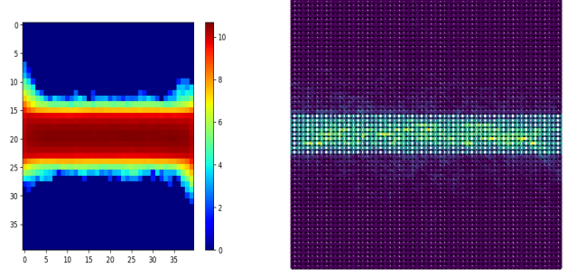
Figure 20: (Left) Log flips plot of running the flip walk with \lambda = 1/\mu_{\text{square}} on G' for 10,000,000 steps. (Right) Edge cut heat map of splitting 1000 uniform spanning trees. In both cases a preference for the horizontal divide is apparent.
