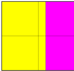
Figure 22: Take \omega to be the number of seats won by party one. Arrange the voters so that every voter with x -coordinate \leq .6 is party one (yellow), and every other voter is party two (purple). In this set up, every roughly vertical partition gives one block to each party and every roughly horizontal partition gives both blocks to party one. The horizontal and vertical partitions are represented by dashed lines.
