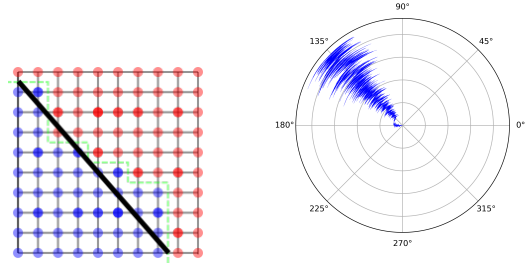
Figure 4: (Left) The boundary line segment. (Right) An example boundary slope plot.
