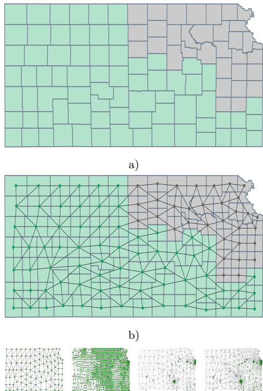
Figure 1: a) Kansas with county units [8], along with a connected 2-partition. b) The corresponding state dual graph overlaid. Much more granular subdivisions of a state such as the census units shown in the bottom row are often used instead of counties.
