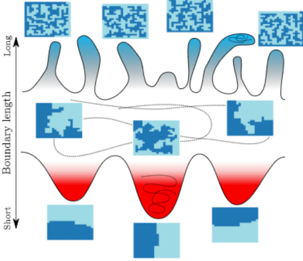
Figure 15: A schematic showing the local geometry of connected graph partitions. The y-axis represents ‘compactness’ (boundary length) as a measure of niceness of the partition.
