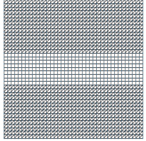
Figure 16: The graph G' .
