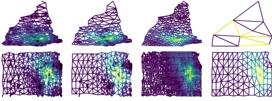
Figure 21: Heat map of boundary edge frequency for the states of New Hampshire and Kansas as computed over four different levels of resolution derived from census data. For each state, we draw 10,000 districting plans, with a 2% population deviation tolerance and compute how often each edge in the dual graph is cut in a partition.
