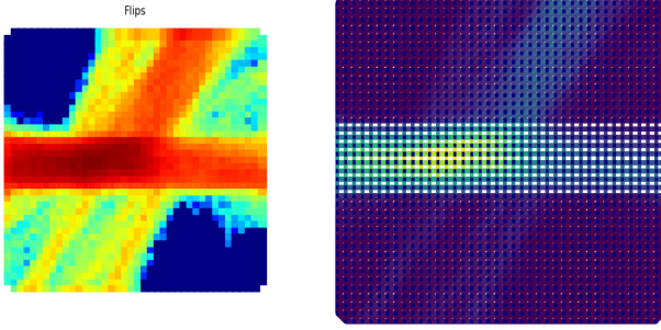
Figure 19: Even if we start with the vertical partition, we rotate into the horizontal partition and then remain there. 1000000 steps. Logflips on the left and edge cuts heat map on the right.
