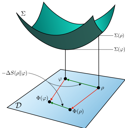
Figure 1. Information-theoretic form of mismatch cost. The top surface represents the entropy production (EP) \Sigma as a function of the initial state \rho , for a physical process whose dynamics is described by the quantum channel \Phi (red arrows). The bottom surface represents the set of states \mathcal{D} . Eq. (3) says that the extra EP incurred by some initial state \rho , additional to the EP incurred by the optimal initial state \varphi which minimizes EP, is equal to the decrease of relative entropy between \rho and \varphi over time (contraction of green arrows).
