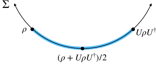
Figure 3. As an example, we consider a physical process in which the EP is invariant under some unitary involution, \Sigma(\rho) = \Sigma(U\rho U^\dagger) and UU = I . For any \rho , the uniform mixture (\rho + U\rho U^\dagger)/2 achieves minimum EP within the set of convex combinations of \rho and U\rho U^\dagger , \mathcal{S} = \{\lambda\rho + (1 - \lambda)U\rho U^\dagger : \lambda \in [0, 1]\} (thick blue line). This leads to the lower bound on EP incurred by state \rho , Eq. (25).
