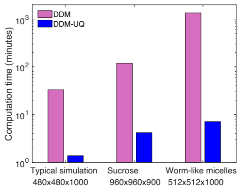
FIG. 8. Pair bar graphs demonstrating the computation efficiency of DDM-UQ scheme (blue) over current DDM approaches (pink). The size of each image stack is labeled underneath the dataset, in terms of frame size \times time points ( L_x \times L_y \times T ).
