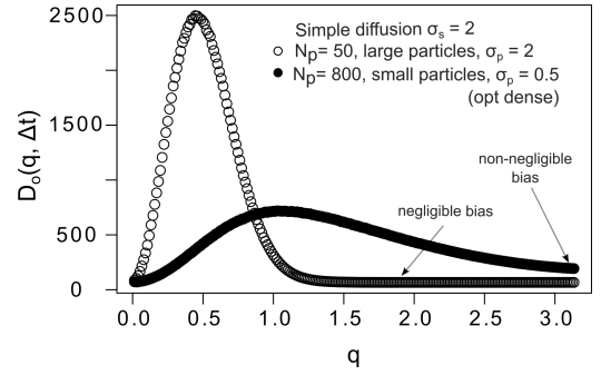
FIG. A2. A close look at the estimators of noise B_{est} in the first and second scenarios of simple diffusion with identical underlying dynamics \sigma_s = 2 , above. The difference lies in that the second case includes 16\times as many particles while particle radius decreases by 4\times (filled circles). For the range of q probed, D_o(q, \Delta t) does not decay to zero at q_{max} .
