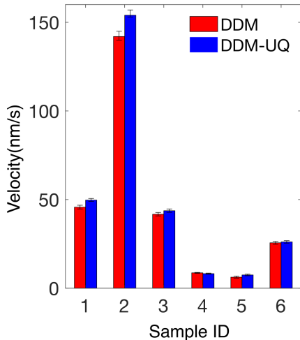
FIG. 10. Velocity estimates and confidence intervals extracted from fitting the stretched exponential model to either the full observations (DDM) or to reconstructed D(q, \Delta t) from selected design points (DDM-UQ). The error bars denote 95% confidence intervals.
