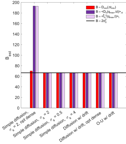
FIG. A1. Comparison of different estimators (denoted by different color bars) for all simulation scenarios. Note that the true noise 2\sigma_0^2 is kept constant in all simulations and denoted by the thick black line.
