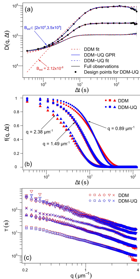
FIG. 9. Example of analysis of an actively-driven system. Experimental data extracted from a fluorescently-labeled actin-myosin-microtubule composite network system reported in [20], processed using DDM (red symbols) or DDM-UQ (blue symbols), and fit to a stretched exponential model to describe the system dynamics (Equ. (28)). (a) Comparing DDM, and DDM DQ fits to the original D_o(q, \Delta t) matrix, where the uncertainty is denoted by the grey shaded area, which is very small as the uncertainty is low. The solid line denotes full D_o(q, \Delta t) data, while the solid dots denotes D_o(q, \Delta t) selected to obtain the predictive distribution. (b) Fits to f(q, \Delta t) shown at several different q 's. (c) Parameter \tau , which describes the system relaxation time, plotted as a function of q . Different symbols represent \tau extracted from 6 different data sets. From this, the system velocity is obtained (Fig. 10).
