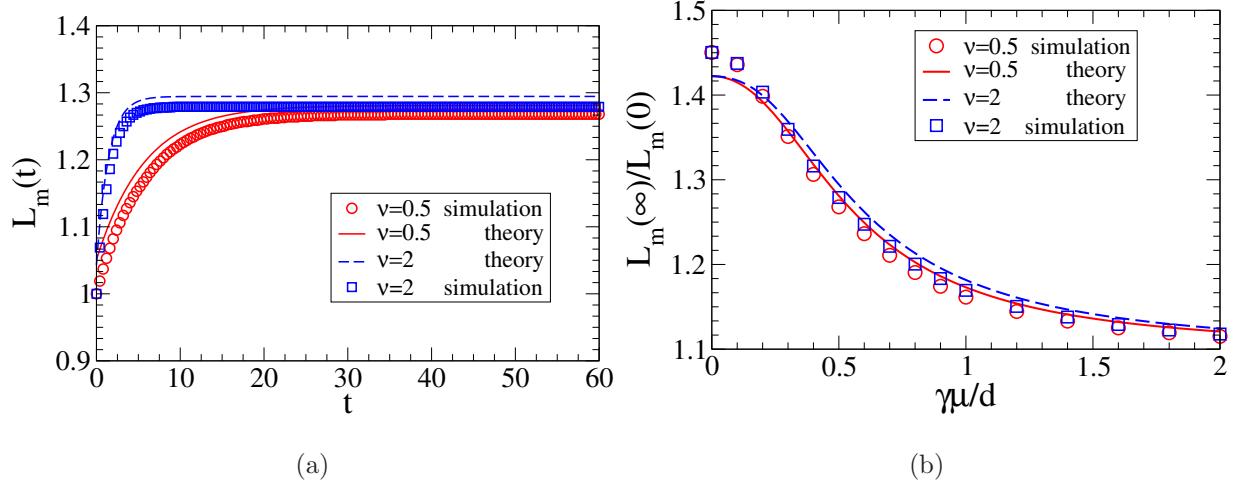
FIG. 13: (a) Tissue size time evolution to the final-state from numerical solutions for \tilde{\nu} = 0.5 and 2 (symbols) with c_0(0) = 0.1 and p = 0.4 . The theoretical approximations from (27) (with f = 0.5 ) for \tilde{\nu} = 0.5 (solid curve) \tilde{\nu} = 2 (dashed curve) are also shown. Time and L_m are in units of 1/d and \sqrt{D/d} respectively. (b) Normalized L_m(\infty) as a function of \tilde{\mu} measured from the numerical solutions at long times. The theoretical results from (28) are also shown.
