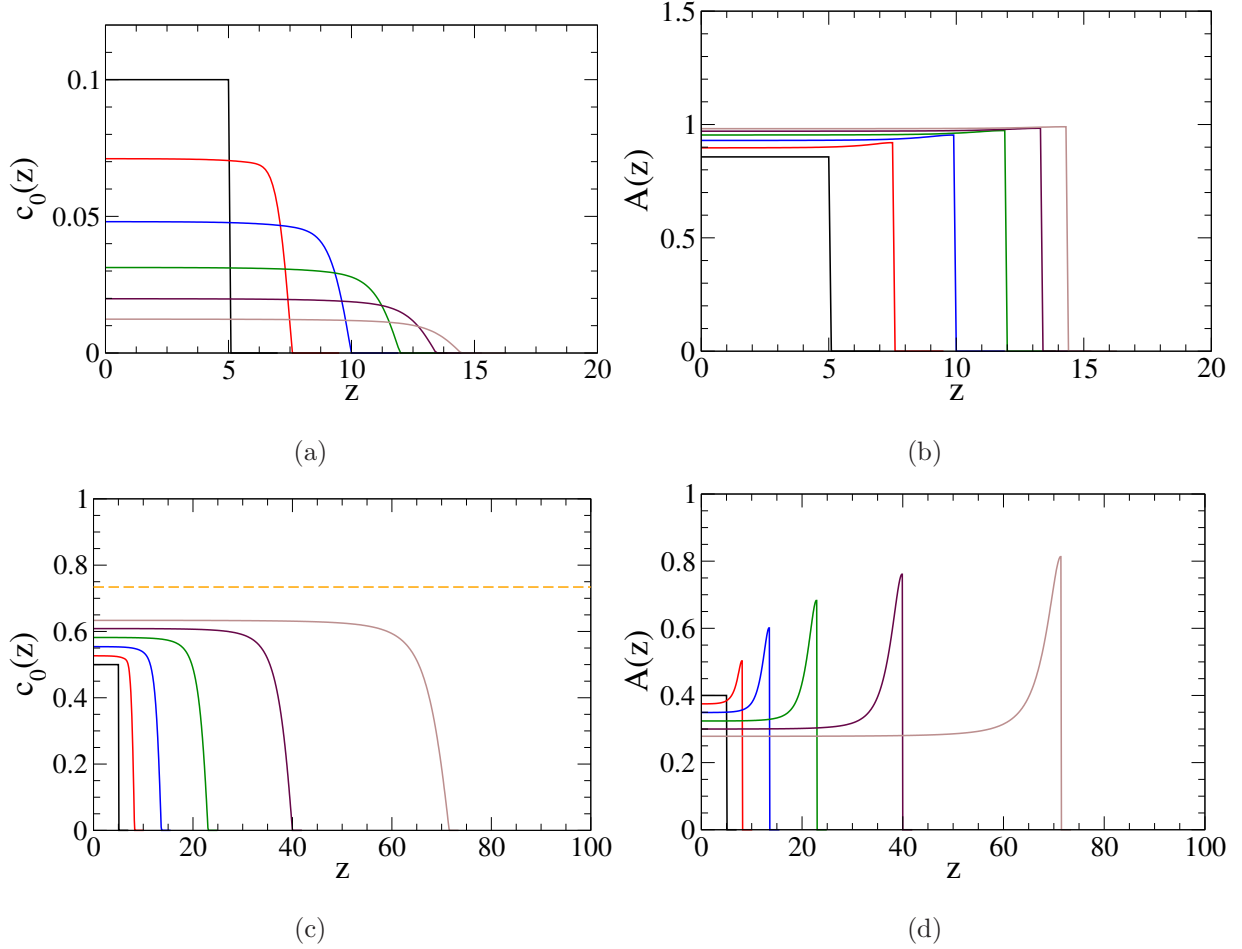
FIG. 7: Numerical solution of the lineage model with m = 2 , \tilde{\nu} = 0.5 and p = 0.9 for \tilde{\mu} = 1 inside the bistable region of the phase diagram in Fig. 3a. Time evolution of the (a) SC distributions c_0(z) , (b) feedback molecule concentrations A(z) , for initial concentration of c_0 = 0.1 . (c) and (d) are similar to (a) -(b) but for initial concentration of c_0 = 0.5 . Distribution curves in (a),(b) and (c),(d) are separated by time intervals of 10 and 2 respectively. Time and space are in units of 1/d and \sqrt{D/d} respectively.
