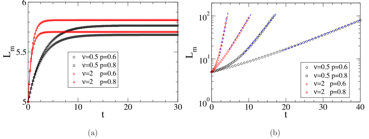
FIG. 9: Numerical results on the tissue size dynamics of the lineage model with m = 2 for (a) \tilde{\mu} = 2 corresponding to the case of the tissue size is governed by the final-state for \tilde{\nu} = 0.5 and 2. The solid curves are fitting of results of the form L_m(t) = a_0 + a_1 e^{-\frac{t}{\tau_s}} . (b) Semi-log plot of the tissue size as a function of time for \mu = 0.2 corresponds to the case of the blow-up growth. The straight lines in the large time regimes are fitting using an exponential form from which the exponential growth time-scales \tau are obtained. Time and L_m are in units of 1/d and \sqrt{D/d} respectively.
