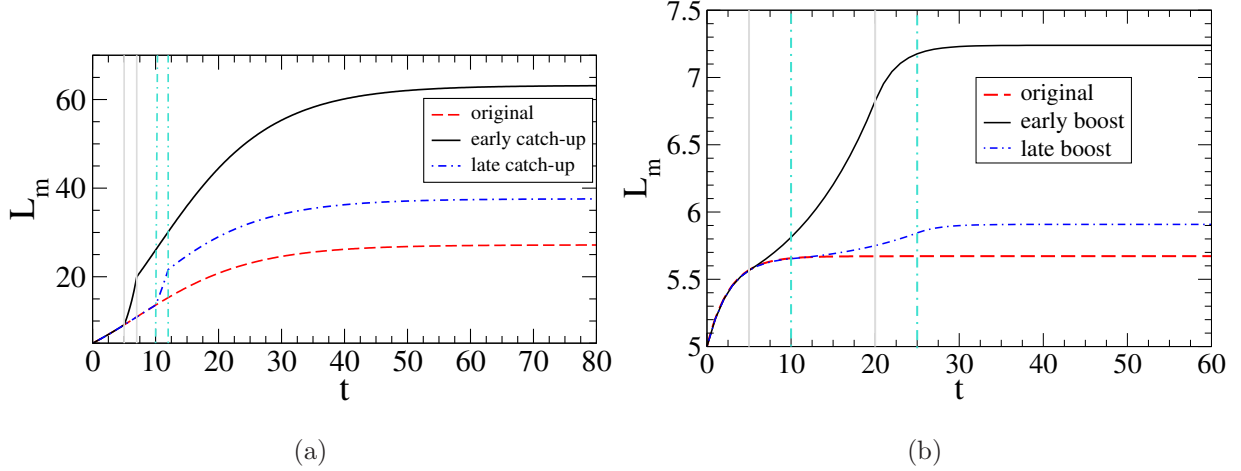
FIG. 16: (a) Catch-up growth modeled by a short duration of increase in the progenitor cell proliferation rate parameter \tilde{\nu} . The original final-state grows with p = 0.8 , \tilde{\mu} = 1 , c_0 = 0.3 and \tilde{\nu} = 0.5 (dashed curve). A catch-up growth occurs at an early stage (solid curve) in 5 \leq t \leq 7 (between two vertical solid lines) during which \tilde{\nu} = 2 . Another similar catch-up growth occurs at a later stage (dot-dashed curve) in 10 \leq t \leq 12 (between two vertical dot-dashed lines) during which \tilde{\nu} = 2 . (b) Boosted growth modeled by a pulse control of the secretion rate parameter of the regulatory molecules, \tilde{\mu} . The original growth of the tissue is with parameters m = 2 , \tilde{\nu} = 0.5 , \tilde{\mu} = 2 and p = 0.6 . The tissue size growth curves are shown for the original (dashed curve), early boosted (solid curve), and late boosted (dot-dashed curve) growths. An early pulse control of \tilde{\mu} is applied for 5 \leq t \leq 15 with the change \tilde{\mu} = 0.1 in this period. Another similar boosted pulse control is also applied but at a later time in 10 \leq t \leq 20 . The vertical lines show the corresponding boosted periods during which \tilde{\mu} is changed. Time and L_m are in units of 1/d and \sqrt{D/d} respectively.
