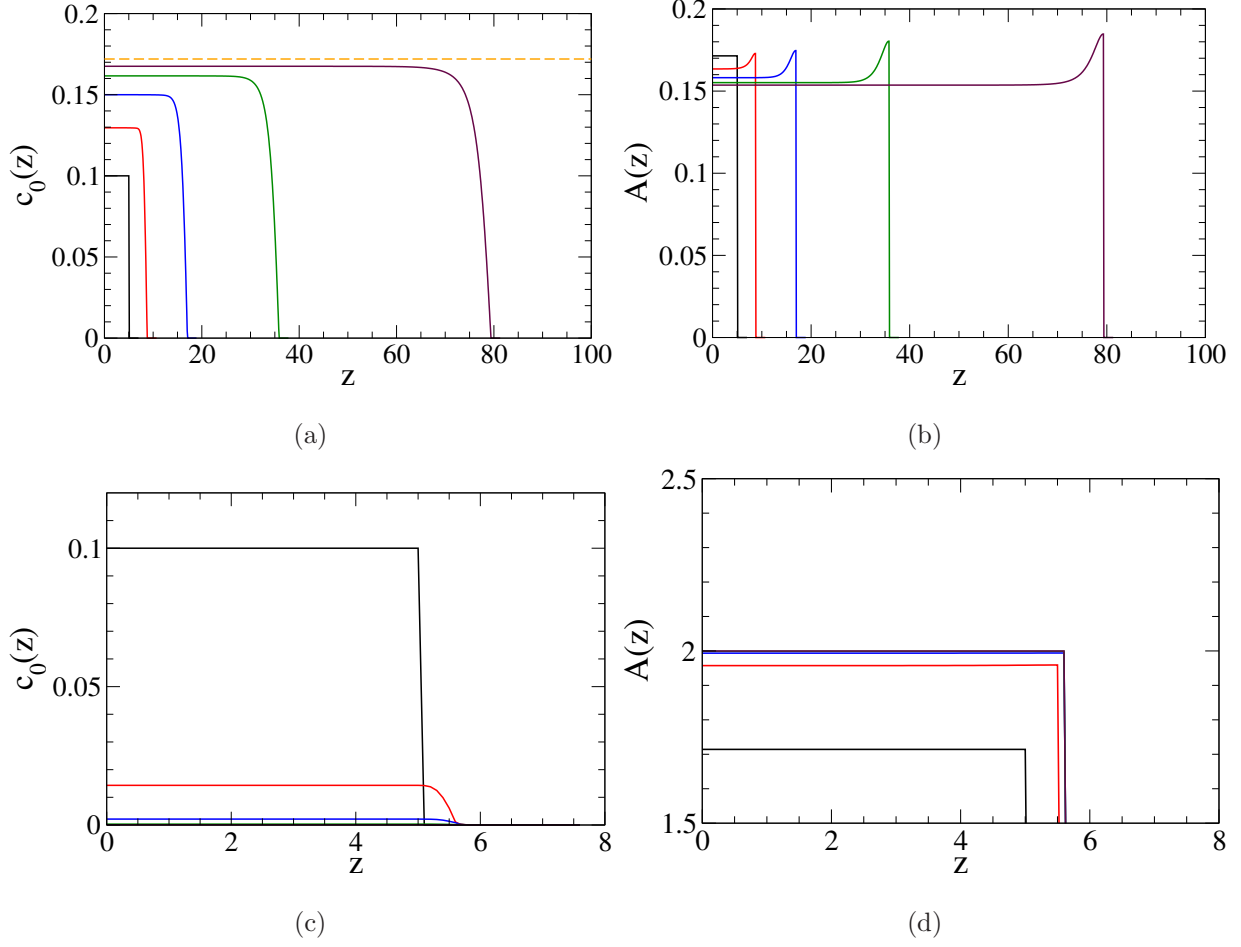
FIG. 5: Numerical solution of the lineage model with m = 2 , \tilde{\nu} = 0.5 and p = 0.6 for \tilde{\mu} = 0.2 inside region I of the phase diagram in Fig. 3a corresponding to the case of blow-up tissue growth. Time evolution of the (a) SC distributions c_0(z) , (b) feedback molecule concentrations A(z) . The non-trivial USS value c_0^* is marked by the horizontal dashed line in (a). (c) and (d) are similar to (a) and (b) for \tilde{\mu} = 2 inside region II of the phase diagram in Fig. 3a corresponding to the case of saturated tissue growth to the final-state. Time and space are in units of 1/d and \sqrt{D/d} respectively. Distribution curves in (a), (b) and (c), (d) are separated by a time of 10 and 5 units respectively.
