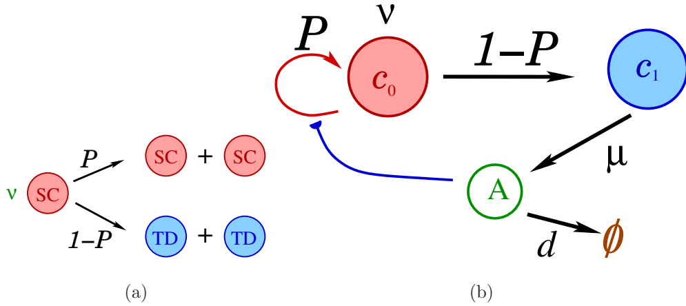
FIG. 1: Schematic picture showing a two-stage cell lineage model with negative feedback. c_0 and c_1 are the concentration of stem cell (SC) and terminally differentiated (TD) cell respectively. (a) SC replicates with a rate of \nu and has a probability \mathcal{P} of duplicating itself and 1 - \mathcal{P} of differentiating into two TD cells. (b) The molecule A , which negative regulates \mathcal{P} , is produced by the TD cells at a rate \mu , and decays with a rate d .
