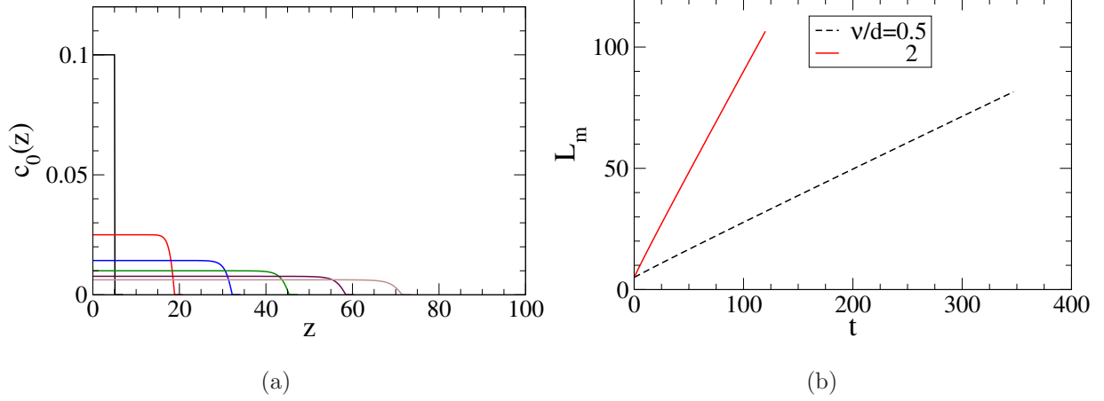
FIG. 15: Tissue designed to grow linearly by feedback control of the concentration of the regulatory molecules. m = 2 . (a) Time evolution of the c_0(z) profiles for \tilde{\nu} = 0.5 , each curve is separated by time intervals of 60 units. Time and space are in units of 1/d and \sqrt{D/d} respectively. (b) Tissue size as a function of time showing the linear growth behavior for \tilde{\nu} = 0.5 and 2. Time and L_m are in units of 1/d and \sqrt{D/d} respectively.
