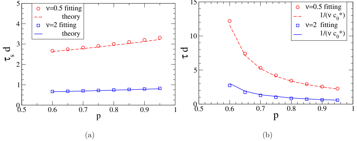
FIG. 11: Characteristic time-scales (in unit of 1/d ) for the controlled growth and blow-up growth, for m = 2 . Symbols are time-scales obtained from fitting of the tissue-size from the numerical solutions. Curves are the corresponding theoretical predictions. (a) \mu = 2 for the case of controlled growth to the final-state. Theoretical predictions are from (29). (b) \mu = 0.2 for the case of blow-up growth. Theoretical predictions are from (22).
