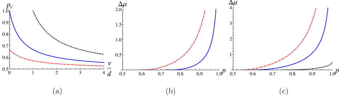
FIG. 4: (a) The critical value at which the coexistence regime vanishes, p_c (given by (13)) as a function of \tilde{v} for different values of the Hill coefficient, m = 1 (dashed black), m = 2 (solid blue) and m = 4 (dot-dashed red). (b) The size of the co-existence regime \Delta\tilde{\mu} \equiv \tilde{\mu}_t^- - \tilde{\mu}_0 (given by (11) and (9)) as a function of p for different values of m for \tilde{v} = 0.5 and (c) for \tilde{v} = 2 .
