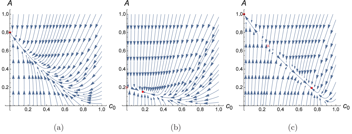
FIG. 8: The A vs. c_0 phase plane portrait obtained from (7) and (8) showing (a) the case of final-state with p = 0.6 , \tilde{\mu} = 0.8 , (b) the case of blow-up state with p = 0.6 , \tilde{\mu} = 0.2 , (c) in the bistable regime with p = 0.9 , \tilde{\mu} = 1 . In all cases, \tilde{\nu} = 0.5 and \gamma = 1 . The stable and unstable fixed points are denoted by a filled and open circles respectively.
