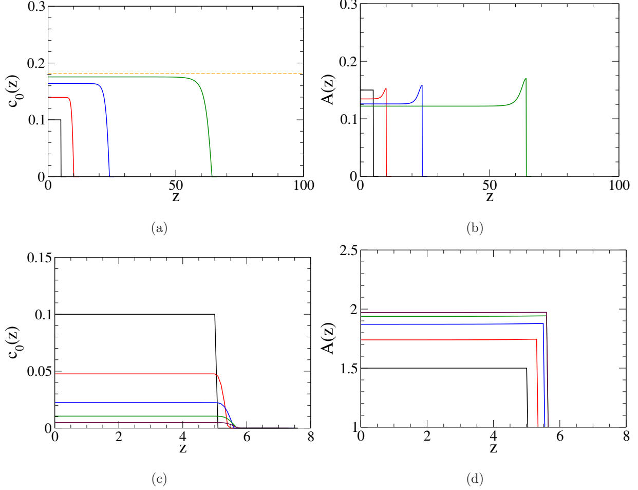
FIG. 6: Numerical solution of the lineage model with m = 2 , \tilde{\nu} = 2 and p = 0.6 for \tilde{\mu} = 0.2 inside region I of the phase diagram in Fig. 3b corresponding to the case of blow-up tissue growth. Time evolution of the (a) SC distributions c_0(z) , (b) feedback molecule concentrations A(z) . (c) and (d) are similar to (a) and (b) for \tilde{\mu} = 2 inside region II of the phase diagram in Fig. 3a corresponding to the case of saturated tissue growth to the final-state. Time and space are in units of 1/d and \sqrt{D/d} respectively. Distribution curves in (a), (b) and (c), (d) are separated by a time of 3 and 0.5 units respectively.
