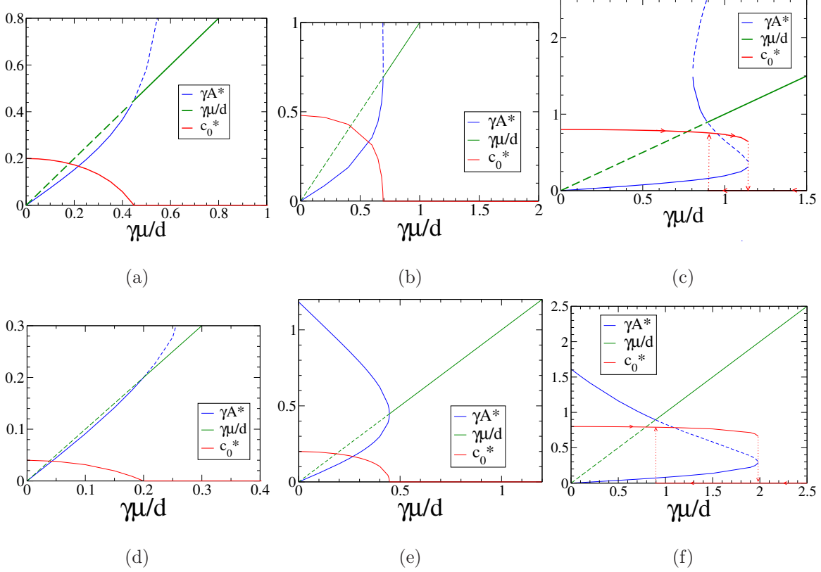
FIG. 2: The trivial (green curve) and non-trivial (blue curve) fixed points \gamma A as a function of \tilde{\mu} \equiv \frac{\gamma \mu}{d} for m = 2 . The solid lines show the stable states and the dashed lines show the unstable states. The corresponding physical ( c_0 \geq 0 ) and stable c_0 states are also shown by the red curve. (a) \tilde{\nu} \equiv \frac{\nu}{d} = 0.5 . p = 0.6 (b) \tilde{\nu} = 0.5 . p = 0.74 . (c) \tilde{\nu} = 0.5 . p = 0.9 . The red vertical dotted lines shows the hysteresis behavior and the bistable phase region lies inbetween them. (d) \tilde{\nu} = 2 . p = 0.52 . (e) \tilde{\nu} = 2 . p = 0.6 . (f) \tilde{\nu} = 2 . p = 0.9 .
