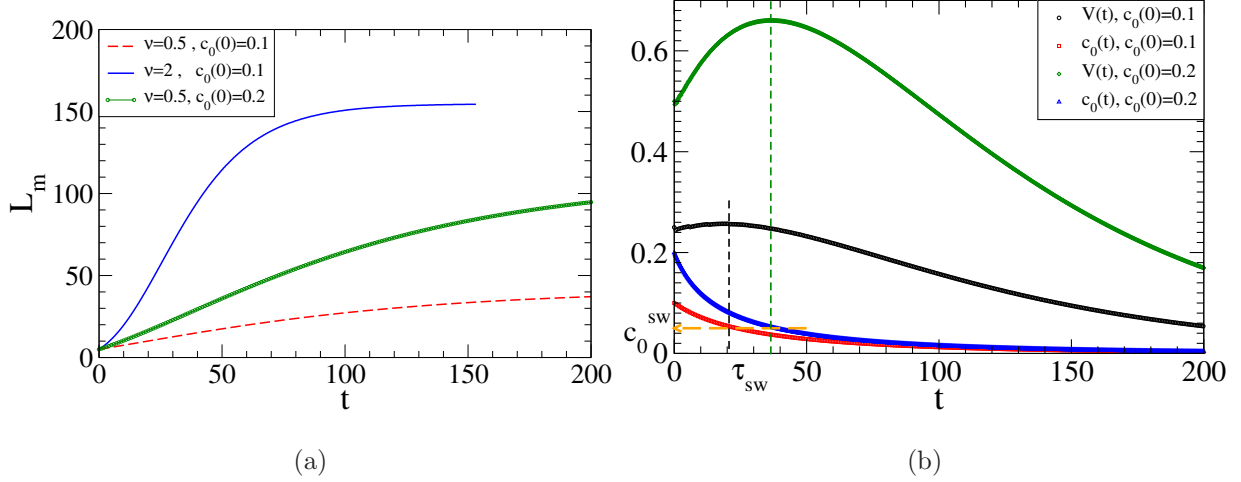
FIG. 12: Numerical results on the tissue size dynamics of the lineage model showing the S-shape growth curve, with m = 2 for (a) Leading edge tissue size as a function of t for \tilde{\mu} = 0.48 , p = 0.6 and \tilde{\nu} = 0.5 and 2. (b) The instantaneous growth speed of the leading edge of the tissue in (a) for \tilde{\nu} = 0.5 and initial SC cell density c_0(0) = 0.1 and 0.2. The maximum of the speed is marked by a vertical dashed line, which occurs at t = \tau_{sw} with the corresponding SC cell density decay to c_0^{sw} \simeq 0.05 (marked by dashed horizontal arrow), which agree reasonably well with the theoretical prediction (from (30)) of 0.047 and is independent of the values of \tilde{\nu} . Time and L_m are in units of 1/d and \sqrt{D/d} respectively.
