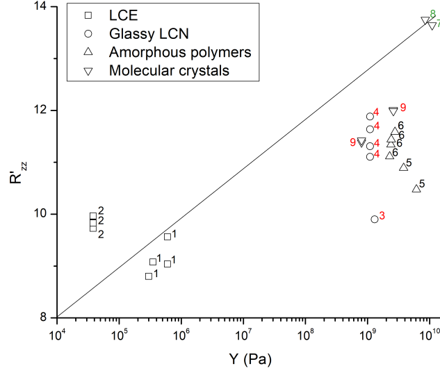
Figure 2: Graph of R'_{zz} vs. Young's modulus Y . The numbers on the graph indicate that R'_{zz} is calculated from data published in papers corresponding to the reference number next to each point in the graph. The line indicates proportionality; deviations are ascribed to differences in values of \phi_{ld} , \varepsilon^d and I_0 .
