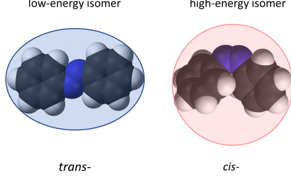
Figure 1: A schematic shows the shape change of a dye isomer under illumination and is excited from the low energy ‘trans’ (left) to the high energy ‘cis’ (right) conformation. The bare strain tensor can be calculated based on the change of semiaxes of the ellipsoid.
