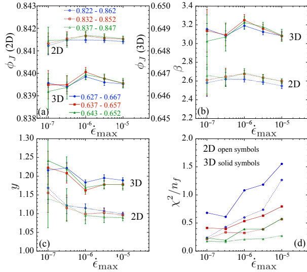
FIG. 2. Critical scaling parameters (a) \phi_J , (b) \beta , (c) y , and (d) the \chi^2/n_f of the fits, vs the upper limit of compression rate \epsilon_{\max} used in the fit, for three different ranges of \phi \in [\phi_{\min}, \phi_{\max}] . Each panel shows results for both 2D and 3D systems. We use the jackknife method to compute the estimated errors and bias-corrected averages of the fit parameters. The data symbols in all panels follow the legend shown in (a); open symbols and dotted lines are for 2D, solid symbols and solid lines are for 3D. Note in (a) that the scale for \phi_J in 2D is on the left, while the scale for \phi_J in 3D is on the right.
