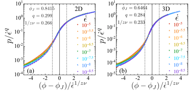
FIG. 3. Scaling collapses showing p/\epsilon vs (\phi - \phi_J)/\epsilon^{1/zv} for (a) our 2D system, and (b) our 3D system. The values of \phi_J , q , and 1/zv used in making these plots come from our fits for \epsilon_{\max} = 10^{-6.5} and the narrowest range of [\phi_{\min}, \phi_{\max}] . The points within this data window, that are used to make the fit, are shown as solid symbols; the points that are not used in the fit are shown as open symbols. We see a good collapse even for data that lies well outside the data window used in the fit. The vertical solid line locates the jamming \delta\phi = 0 ; the vertical dashed lines denote the additional constraint |x| \leq 1 for data used in the fit.
