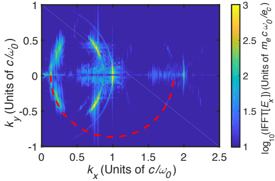
FIG. 4. Wave number spectrum of E_x for peak laser intensity I_0 = 1 \times 10^{17} \text{ Wcm}^{-2} and electron density n_e = 1.6\% n_c at time t = 2.4 ps, showing the angular dependence of the near-forward SRS and the spectrum present for other laser plasma instabilities. The red semi-circle shows wave numbers in the lower half plane for which an electron plasma wave would satisfy k-matching conditions with an incident and scattered light wave.
