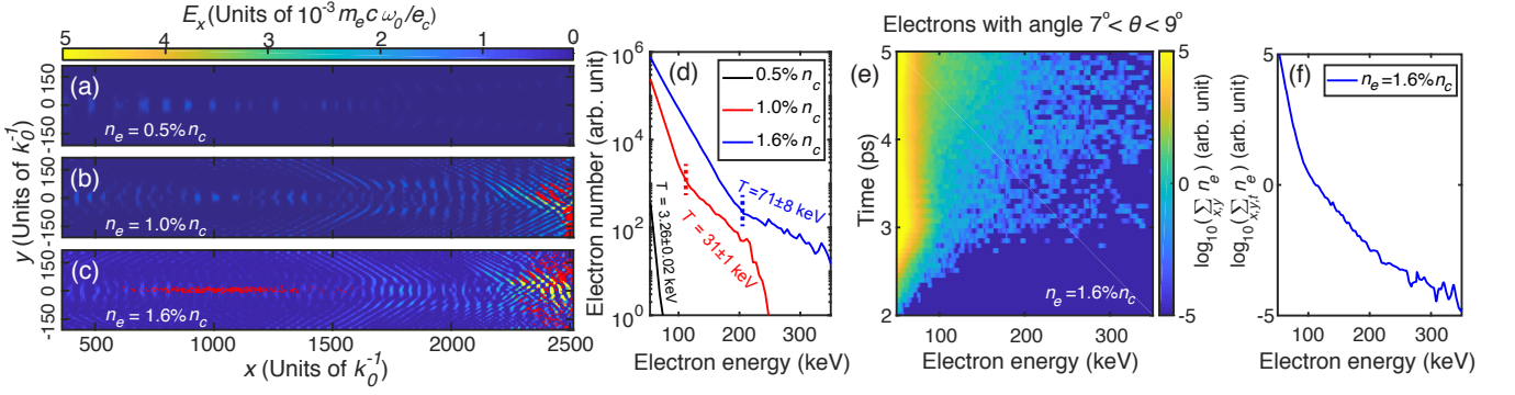
FIG. 3. (a-c) Electron plasma wave activity (laser propagating from left to right, entering at x = 0 ) for a peak laser intensity I_0 = 1 \times 10^{17} \text{ Wcm}^{-2} at t = 4.3 ps for electron densities: (a) n_e = 0.5\% n_c , (b) n_e = 1.0\% n_c and (c) n_e = 1.6\% n_c , with electrons of energy \epsilon > 150 keV overlaid as red circles. For clarity only 10% of these electrons are displayed in (c). (d) Net electron spectra of all electrons present in the simulation domain at t = 4.3 ps. The slope temperatures are given in (d) for the high energy portion of the spectra (minimum computed energy indicated by the dashed lines). (e) Histogram of electron density for the n_e = 1.6\% n_c case, for all electrons accelerated at an angle equal to 8^\circ \pm 1^\circ - similar to the collection angle of the electron spectrometer used experimentally. (f) Summation of the electron density shown in (e) for the whole simulated time.
