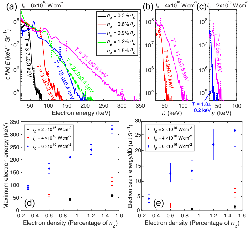
FIG. 2. (a-c) Electron spectra recorded by the electron spectrometer for five values of plasma electron density n_e and peak laser intensities I_0 equal to: (a) I_0 = 6 \times 10^{16} \text{ Wcm}^{-2} , (b) I_0 = 4 \times 10^{16} \text{ Wcm}^{-2} and (c) I_0 = 2 \times 10^{16} \text{ Wcm}^{-2} . A temperature fit to each spectrum was performed, with the hot electron slope temperature T labelled next to the corresponding spectrum. The fit was performed in the range bound by the colored dashed vertical lines, where the electron temperature can be accurately described by a single temperature dependence. Note that the data series shown in (a-c) correspond to the legend shown in (a). (d) \varepsilon_{max} and (e) total energy contained in the accelerated electron population per solid angle \Omega as a function of n_e for the three values of I_0 explored experimentally.
