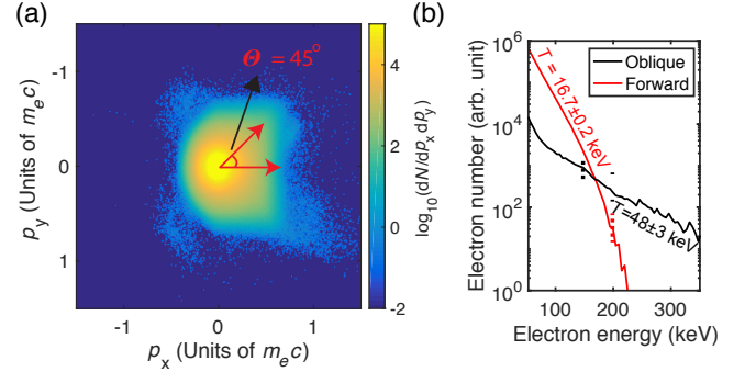
FIG. 5. (a) Electron phase space plot for a peak laser intensity I_0 = 1 \times 10^{17} \text{ Wcm}^{-2} and electron density n_e = 1.6\% n_c at time t = 4.3 ps, showing the angular dependence of the accelerated electrons. The plasma wave angle \theta is shown for the oblique wave. (b) Separate electron spectra (at t = 4.3 ps) showing those electrons accelerated due to forward SRS and those accelerated by near-forward SRS. Slope temperatures T are given; in the case of forward SRS-driven electrons the dashed red line indicates the cut-off energy the fit is performed to. In the case of oblique electrons, the dashed black line indicates the starting energy in the fit protocol.
