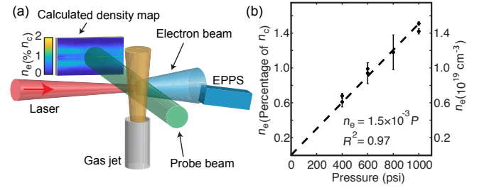
FIG. 1. (a) Schematic displaying the experimental configuration, where EPSS is the electron spectrometer. An example density map measured by the interferometer is shown, for a peak laser intensity I_0 = 2 \times 10^{16} \text{ Wcm}^{-2} and pressure P = 400 \text{ psi} . The electron density n_e is shown as a percentage of the critical density n_c . (b) Measured n_e as a function of P obtained from multiple interferograms for I_0 = 2 \times 10^{16} \text{ Wcm}^{-2} . The dashed black line is a linear fit to the data intercepting at n_e = 0 , with the fit parameters labelled.
