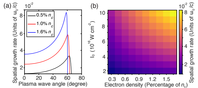
FIG. 6. (a) Spatial growth rate of the electron plasma wave (EPW) as a function of plasma wave angle for the three electron densities used in the simulations ( 0^\circ refers to the angle of laser propagation) and peak laser intensity I_0 = 10^{17} \text{ W cm}^{-2} . (b) Laser intensity and electron density map of the spatial growth rate of the EPW for the full domain investigated experimentally, at the angle of maximum growth rate for each case.
