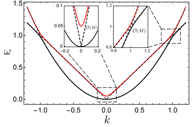
FIG. 2. (color online) Dispersion relation of a uniformly curved rod of infinite extent with M = 0.05 . The degeneracy between the M = 0 dispersion curves (dashed black lines) is lifted due to curvature. Level splitting between the upper branch (red) and lower branch (black) is \mathcal{O}(M) near wavenumbers k = \pm 1 and k = 0 .
