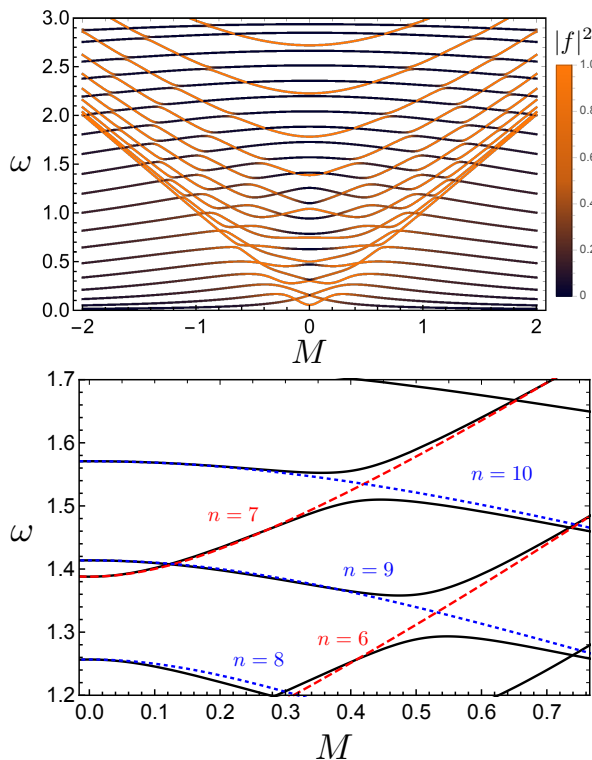
FIG. 4. (color online) The frequency spectrum of a clamped rod of length \ell = 20 as a function of curvature M . Top: the M -dependence of the frequency spectrum, color coded by the relative amplitude of its f to u mode, where lighter colors represent more bending f -amplitude. Due to parametric M -dependence, each curve represents one eigenmode. We find three distinct regimes: high \omega where the curves look like their infinite-rod counterparts, intermediate \omega , where the spectrum is approximated by free dispersion curves with level splitting, and low \omega where curvature strongly distorts the spectrum. Bottom: a close up view of the frequency spectrum (black solid lines) overlaid with the infinite rod dispersion curves for several modes labeled by n in the figure (dashed lines). Level splitting occurs between even and odd numbered modes, as explained in the text.
