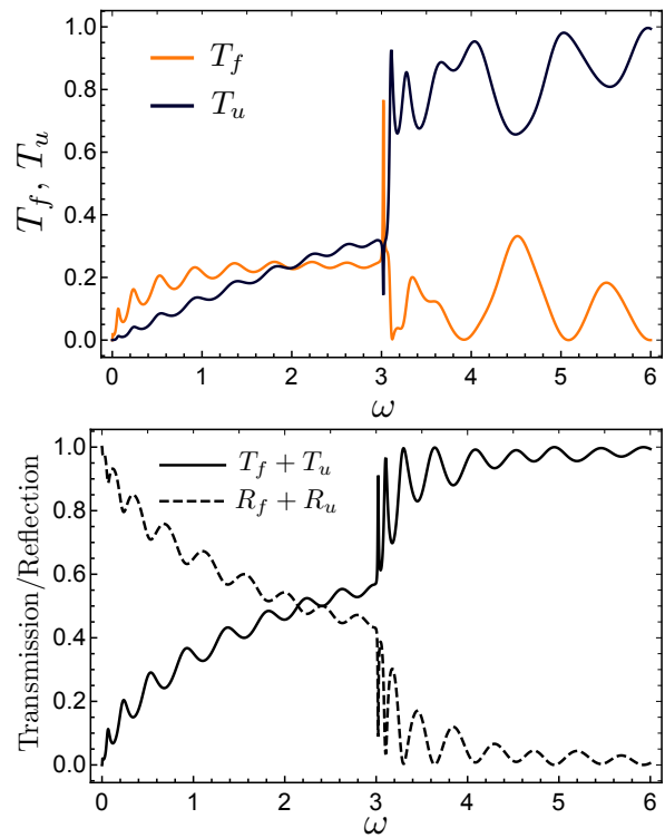
FIG. 7. (color online) Transmission and reflection coefficients for a compression wave of unit amplitude incident on a region of length \ell = 10 , with uniform curvature M = 3 . Top: the transmission coefficients for bending (orange) and compression (black) waves. Bottom: the total transmission and reflection coefficients. In contrast to an incident bending wave, see Fig. 6, the transmission coefficients vanish as \omega \rightarrow 0 .
