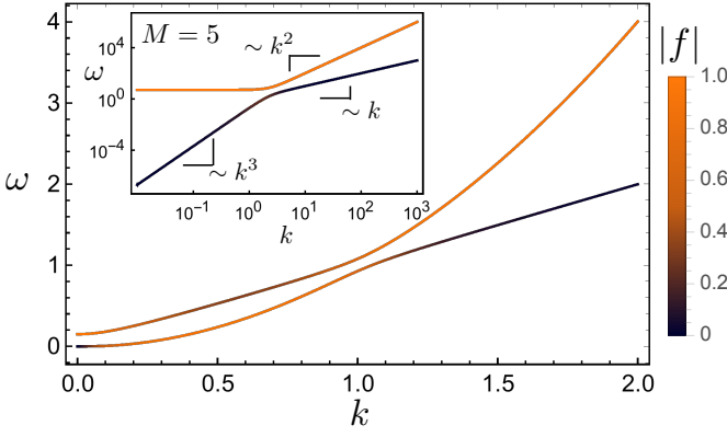
FIG. 3. (color online) The dispersion relation of a rod with uniform curvature, color-coded according to the normalized amplitude of its corresponding |f\rangle eigenstate. M = 0.15 and \ell = 1 . Mode mixing is strongest near the degeneracy points of the M = 0 case. In the inset, we show the behavior for larger curvature M > 1 . At small k , the upper branch is essentially flat, while the lower branch develops an \omega_- \approx |k|^3/M power law, in contrast to its quadratic dispersion relation at small curvature.
