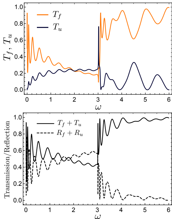
FIG. 6. (color online) Transmission and reflection coefficients for a bending wave of unit amplitude incident on a region of length \ell = 10 , with uniform curvature M = 3 . Top: the transmission coefficients for bending (orange) and compression (black) waves. Bottom: the total transmission and reflection coefficients. Due to conservation of energy, the coefficients obey T_f + T_u + R_f + R_u = 1 . Curvature mixes eigenmodes, converting the incident pure bending wave into a linear combination of bending and compression waves.
