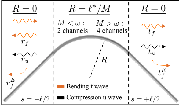
FIG. 5. (color online) Schematic representation of an elastic rod (solid gray line) formed by adjoining two semi-infinite straight rods at the (black) dashed lines to the left ( s = -\ell/2 ) and right ( s = \ell/2 ) of the curved rod segment (arc of a circle with radius R ), such that the rod and its tangent are everywhere continuous. We consider the scattering of an incoming bending f wave from the left, through the region of constant curvature M . Curvy arrows correspond to propagating asymptotic states, and decaying arrows to evanescent states. The darker (lighter) colors refer to u ( f ) modes. There are six unknown transmission/reflection amplitudes. In the curved region, there are either two or four propagating channels, determined by the value of M .
