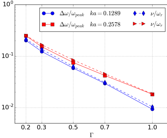
FIG. 10. (Color online) Comparison between the relative (right) HWHM obtained from the RPA S(\mathbf{k}, \omega) and the ratio of the imaginary over the real part of the complex solution of \epsilon(k, \omega) = 0 . \kappa = 0.5 .
