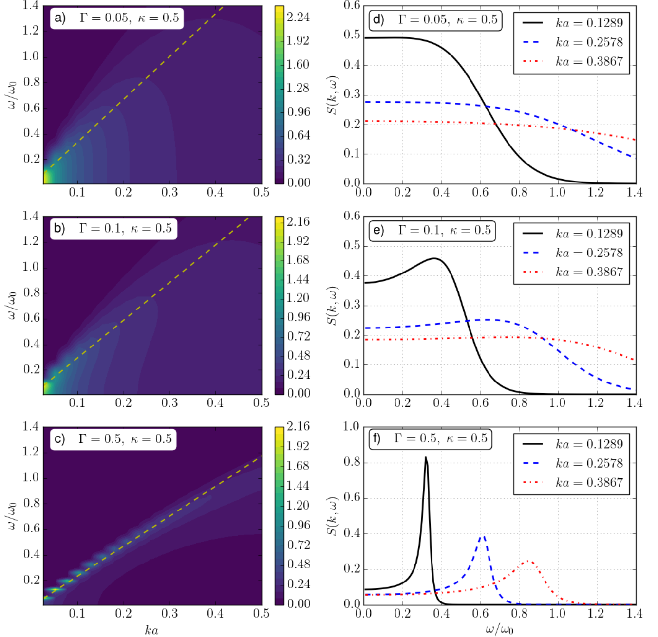
FIG. 3. (Color online) Panels a) - c): color maps of S(\mathbf{k}, \omega) , calculated using eqs. (15) and (21), showing the dispersion (or lack of) of the longitudinal acoustic mode, the dashed lines indicate the acoustic mode \omega(k) = s_{\text{RPA}}k where s_{\text{RPA}} is given by eq. (19). Panels d) - f): line plots of S(\mathbf{k}, \omega) at three ka values showing the presence (or lack of) of the acoustic peak. The ka values are the same for all plots and indicate in the bottom one. The \Gamma, \kappa values are indicated in the inserts. Panels a) and d) belong to Domain 1, b) and e) on the boundary between Domain 1 and Domain 2, and c) and f) plots belong to Domain 2.
