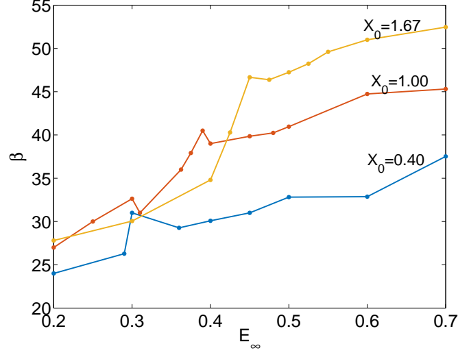
FIG. 6. (Color online) Double cone angle \beta versus E_\infty , for X_0 = 0.4, 1, 1.67 .
