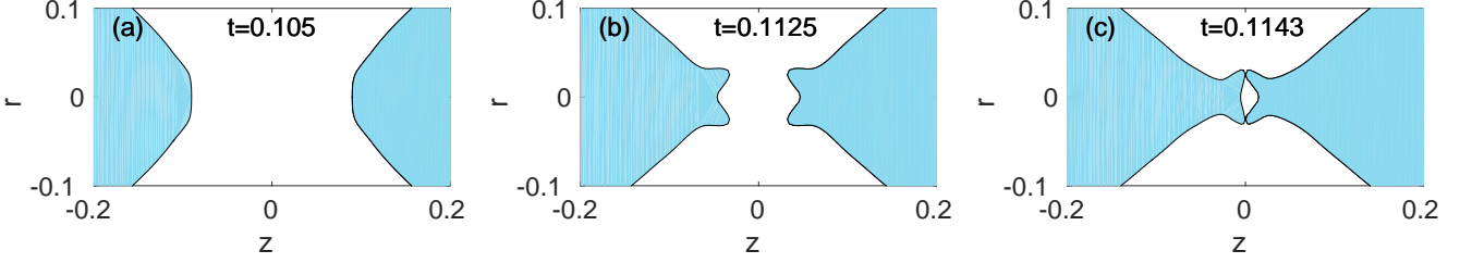
FIG. 9. (Color online) Zoomed drops facing shapes for E_\infty = 0.7 . The individual droplets are about to emit jets and an air bubble is trapped inside the fluid.
