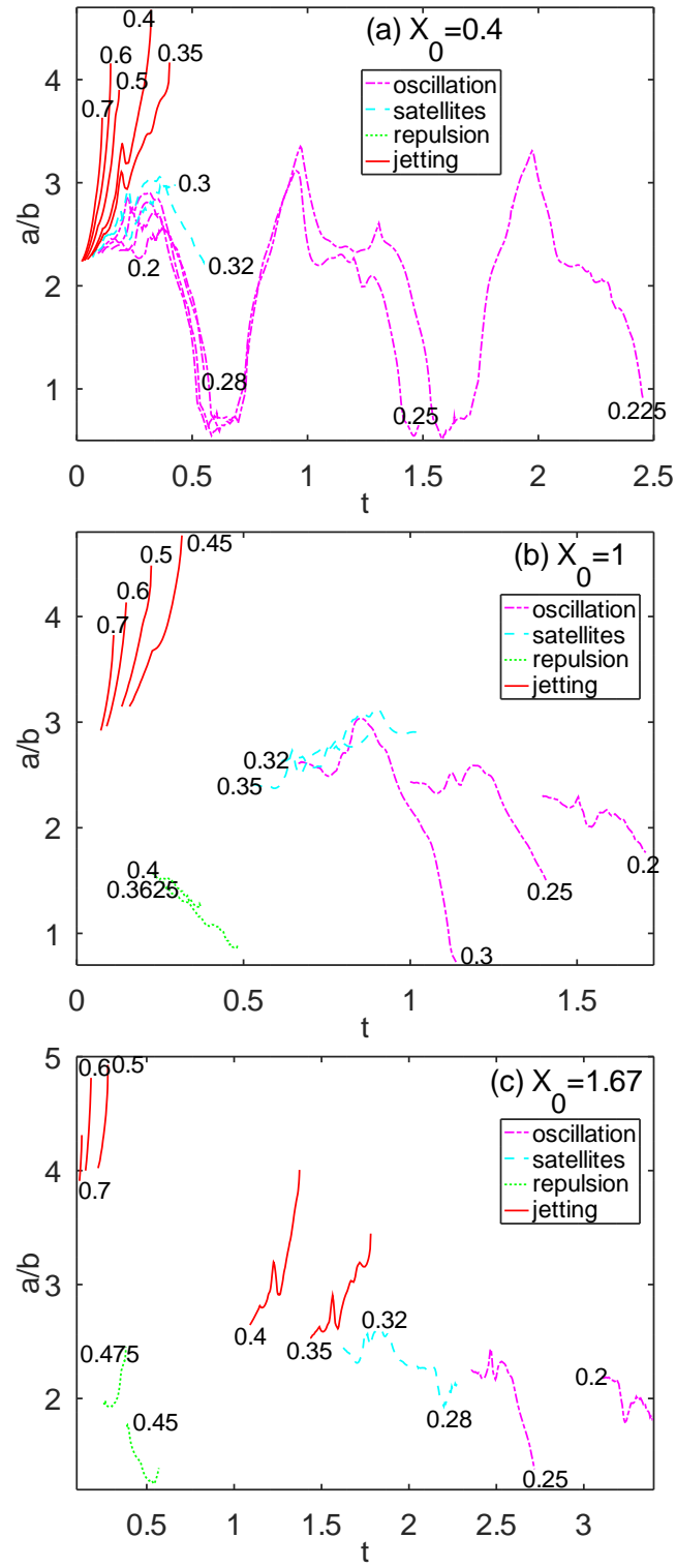
FIG. 11. (Color online) Evolution of the post-coalesced droplets aspect ratio a/b for various electric fields intensities. Each graph specifies the corresponding X_0 value.
