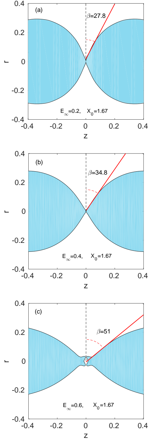
FIG. 8. (Color online) Calculated cone angles at contact points for X_0 = 1.67 and E_\infty = 0.2, 0.4, 0.6 .
