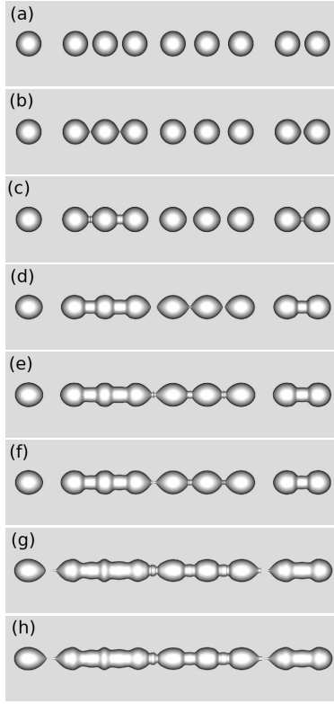
FIG. 21. 3D renderings of nine droplets front profiles for E_\infty = 0.4 at times: (a) t = 0 , (b) t = 0.0281 , (c) t = 0.0488 , (d) t = 0.0785 , (e) t = 0.0850 , (f) t = 0.0910 , (g) t = 0.1176 , (h) t = 0.1213 . The horizontal axis is z \in [-5, 4] and the vertical axis is r \in [-0.5, 0.5] . Coalescence fronts start propagating where the droplets are closer.
