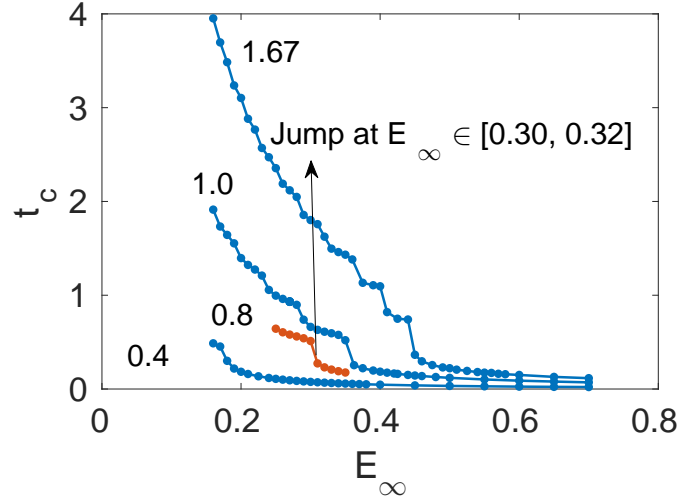
FIG. 17. (Color online) Coalescence times t_c versus E_\infty for X_0 = 0.8 . The curves corresponding to X_0 = 0.4, 1, 1.67 has been included as a reference. The transition zone between regimes occurs in the interval E_\infty \in [0.3, 0.32] where recoiling takes place.
