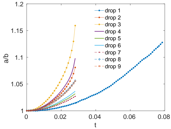
FIG. 19. (Color online) Nine droplets aspect ratio a/b evolution for E_\infty = 0.4 before first coalescence. All droplets deform differently.
