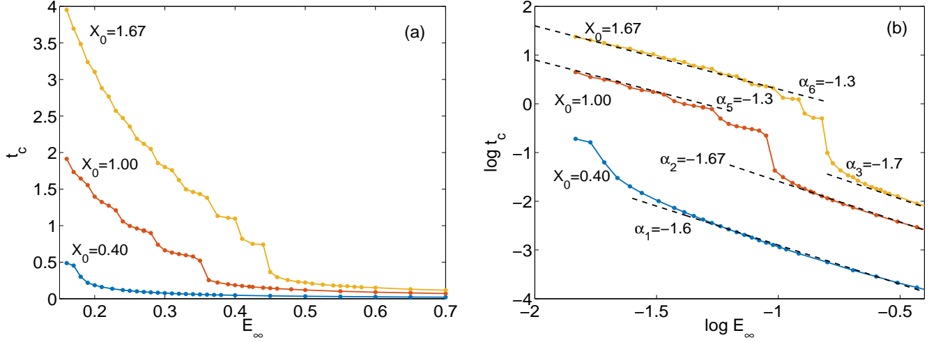
FIG. 5. (Color online) (Left) Coalescence times t_c versus E_\infty . (Right) Corresponding log-log plot with the exponents of the linear fittings. The log is natural logarithm. For X_0 = 1, 1.67 there is a curve jump between the two distinct flow regimes.
