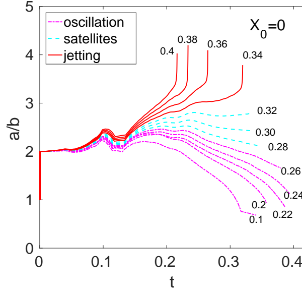
FIG. 10. (Color online) Aspect ratio a/b evolution after contact for X_0 = 0 at indicated E_\infty values. The post-coalescence sequence is: oscillation, satellites and jetting.
