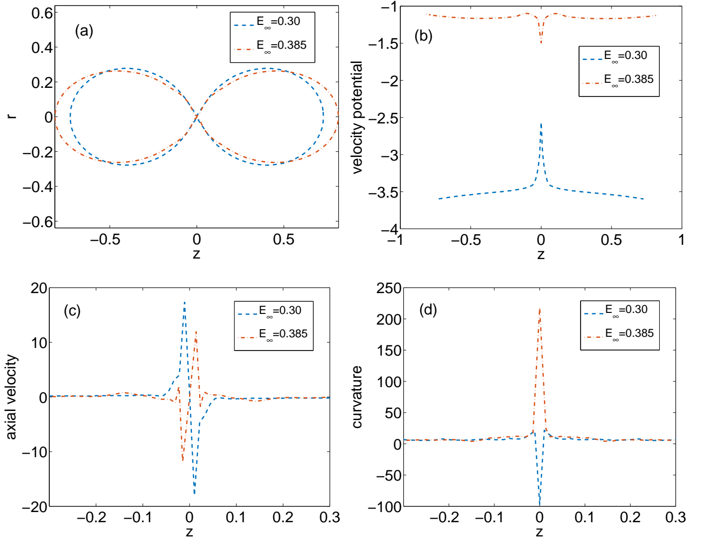
FIG. 16. (Color online) Comparison between flow variables for repulsion, E_\infty = 0.385 , versus coalescence, E_\infty = 0.3 at contact time. The re-scaled separation is X_0 = 1 . Panel (a) shows that the repulsion front profile is more deformed than the coalescence profile, panel (b) shows velocity potentials. In panel (c) the opposite axial velocity behavior is depicted and panel (d) shows the opposite curvature signs at contact point.
