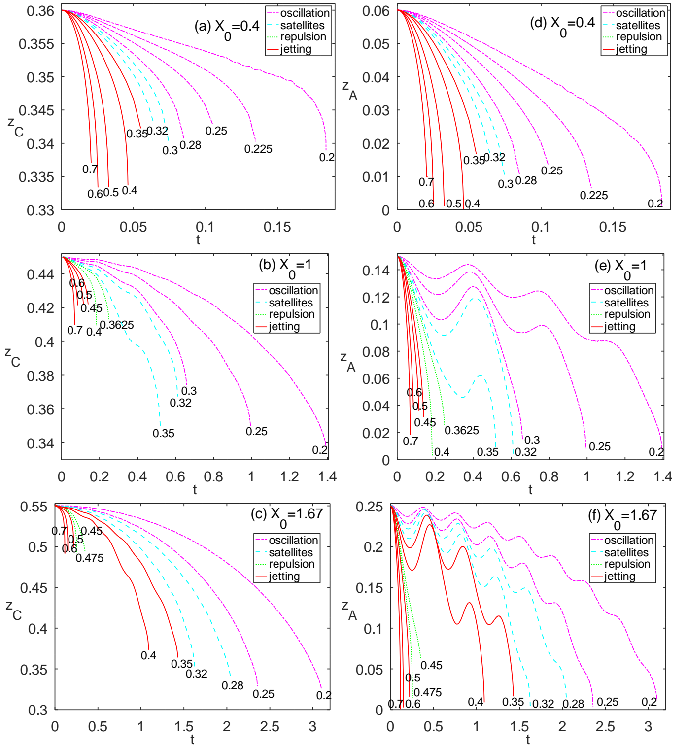
FIG. 4. (Color online)(Left) Evolution of the droplets center axial coordinate z_C for various electric field intensities and indicated X_0 values. (Right) Same for the evolution of the drop left point z_A . The curves color and line styles represent the corresponding post-coalescence modes.
