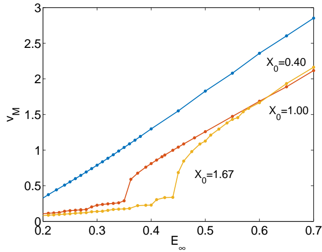
FIG. 7. (Color online) Average droplet velocity V_M = D_0/t_c versus E_\infty for X_0 = 0.4, 1, 1.67 . For X_0 = 1, 1.67 the average velocity is V_M \approx 0.5 at the curve jumps.
