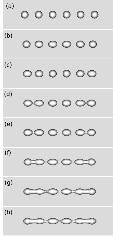
FIG. 20. 3D renderings of six droplets front profiles for E_\infty = 0.4 at times: (a) t = 0 , (b) t = 1 , (c) t = 1.2 , (d) t = 1.2858 , (e) t = 1.3001 , (f) t = 1.3648 , (g) t = 1.3985 , (h) t = 1.4099 . The horizontal axis is z \in [-4, 4] and the vertical axis is r \in [-0.5, 0.5] . Note that the coalescence front propagates inwards.
