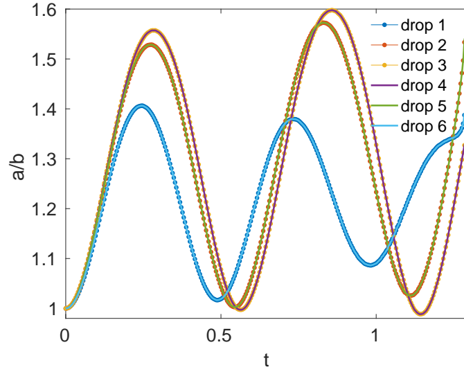
FIG. 18. (Color online) Six droplets aspect ratio a/b evolution for E_\infty = 0.4 before first coalescence. Droplets 1,6 undergo same deformation. Same behavior for droplets 2,5 and droplets 3,4.
