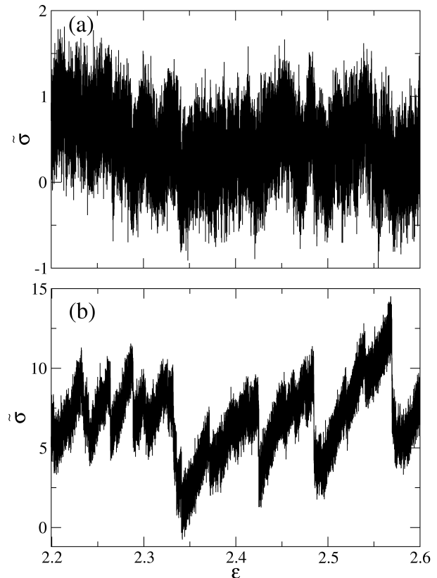
FIG. 3: (a) Section of stress-strain curve for lowest-density state point on the higher-temperature isomorph ( \rho = 1.265, T = 0.550 ) at the lowest nominal strain rate 10^{-5} . (b) Section of stress-strain curve for a state point on the lower temperature isomorph ( \rho = 1.324, T = 0.100 ) at the lowest strain rate 10^{-5} . The abrupt drops can be identified with avalanches of plastic activity. The difference in vertical scale between (a) and (b) can be attributed partly to the definition of reduced units for stress.
