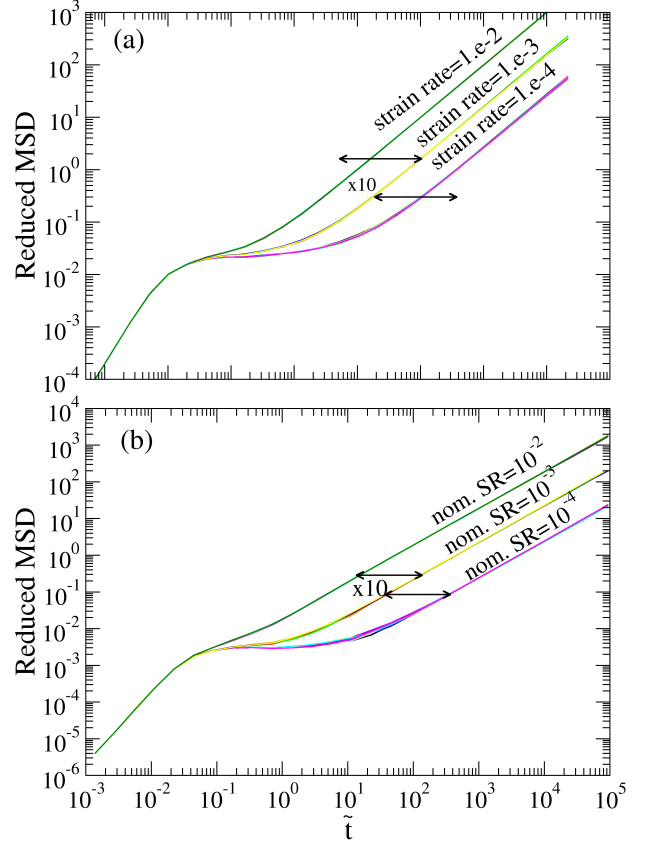
FIG. 12: Mean squared transverse displacement plotted in reduced units for (a) high temperature isomorph and (b) low temperature isomorph. The horizontal arrows indicate a factor of ten in the time axis, and can be used to judge by what factor the curves can be shifted onto each other in time.
