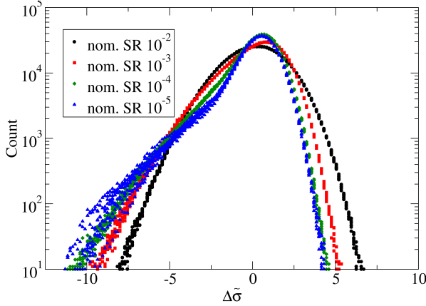
FIG. 10: Histograms of (reduced) stress changes over strain intervals \varepsilon_s chosen to minimize skewness for each strain rate, on the low temperature isomorph. Data for different points on the isomorph are plotted in the same color for each nominal strain rate. In order of decreasing strain the minimum-skew strain intervals, as judged by eye from Fig. 9, are 0.02, 0.008, 0.004, 0.003.
