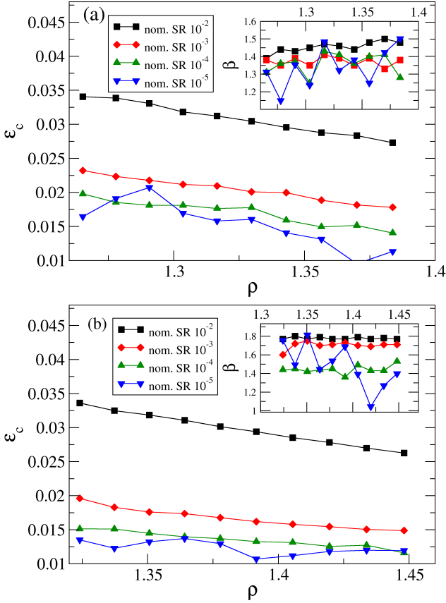
FIG. 6: Fits of shear stress autocorrelation to Eq. (6) shown as functions of density along the high (a) and low temperature (b) isomorphs. The characteristic strain over which decays occurs, \varepsilon_c , decreases approximately linearly as density increases.
