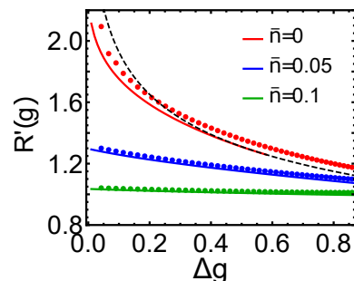
FIG. 7. The scaled inverse temperature R'(g) of the intrawell probability distribution as a function of the RWA energy g , \Delta g = (g - g_{\text{min}})/(g_s - g_{\text{min}}) . The scaled driving amplitude is f = 0.5 . The dots refer to R' obtained by solving the balance equation (13) using the Wannier functions, R'(g_n) = -\lambda \log(\rho_{n+1}/\rho_{n-1})/(g_{n+1} - g_{n-1}) . The scaled Planck constant is \lambda = 0.004 . There are approximately 50 levels in each well. The solid lines refer to R' obtained from Eq. (27), which does not contain \lambda . The black dashed line shows 2\tau_\infty(g) . At \bar{n} = 0 , R'(g) obtained using Eq. (27) (red solid line) becomes equal to 2\tau_\infty(g) for g = g_{\text{NL}} . For larger g , where R'(g) > 2\tau_\infty(g) , the local approximation breaks down, Eq. (27) no longer applies, and this is why the red line terminates at g_{\text{NL}} . The difference between the dots and the solid lines of the same color is due to \lambda being nonzero and is most significant when R' becomes close to 2\tau_\infty .
