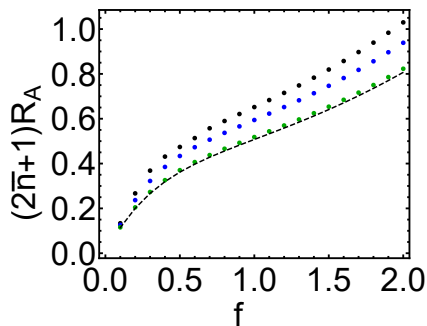
FIG. 10. The semiclassical activation energy R_A as a function of the scaled drive amplitude f . The black, blue, and green dots refer to \bar{n} = 0.01, 0.1 , and 1 , respectively. The dashed line refers to the result of the classical limit obtained from Eq. (28).
