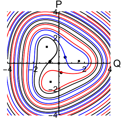
FIG. 12. The phase portrait of a classical oscillator driven close to three times its eigenfrequency; Q and P are the scaled coordinate and momentum in the rotating frame. The scaled amplitude of the driving field is f = 1 , the scaled decay rate is \kappa = 0.5 , and \delta\omega > 0 . The squares show the positions of the stable period-three states, whereas the circles show the positions of the saddle points. The solid lines show the separatrices that separate the basins of attraction to different stable period-three states and to the zero-amplitude state at the origin. As \kappa \rightarrow 0 , the squares and the saddles rotate and shift and approach their position in Fig. 1 (c).
