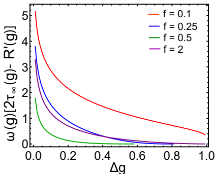
FIG. 5. The rate \omega(g)[2\tau_\infty(g) - R'(g)] of the fall-off of the relative probability flux \mathcal{J}_{-|m|}^{\text{in}}(g) , Eq. (30), into the intrawell state with a given RWA energy g from lower-lying states, for different \Delta g = (g - g_{\min})/(g_s - g_{\min}) . The lines refer to the scaled driving amplitude f = 0.1 (red), 0.25 (blue), 0.5 (green), and 2 (purple). As the RWA energy g approaches g_{\min} , one can show that \omega(g)[2\tau_\infty(g) - R'(g)] diverges \propto |\ln(g - g_{\min})| .
