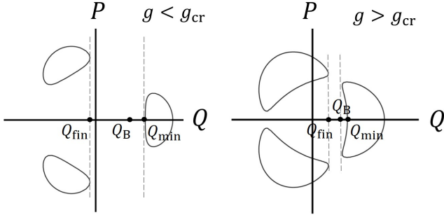
FIG. 16. An example of elliptical (left) and horseshoe-like (right) classical orbit when g < g_{\text{cr}} and g > g_{\text{cr}} , respectively; \delta\omega > 0 .
