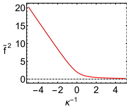
FIG. 11. The interrelation between the amplitude and frequency of the drive where the period tripling emerges. The abscissa shows the detuning of the driving field frequency \delta\omega divided by the oscillator relaxation rate in the unscaled time, \kappa^{-1} = \delta\omega/\Gamma . The ordinate shows the scaled squared amplitude of the driving field \tilde{f}^2 = F^2/24\omega_0^2\gamma\Gamma ; the scaling is independent of the frequency detuning. Above the bifurcation curve the oscillator has three stable period-3 states and a stable zero-amplitude state; below this curve, only the zero-amplitude state is stable. The plot refers to \gamma\delta\omega > 0 .
