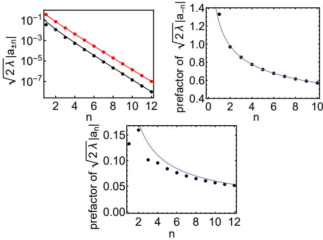
FIG. 14. Upper left panel: the absolute value of the semiclassical matrix elements |a_{\pm n}| on the logarithmic scale. The red and black dots refer to |a_{-n}| and |a_n| , respectively. The red and black solid lines are the corresponding asymptotic expressions (18) and (19). Upper right and lower panels: the prefactor of the semiclassical matrix element a_{\pm n} . Dots and solid lines show the numerical and analytical results, respectively. The value of the scaled drive amplitude is f = 0.5 , and the quasienergy of the orbit is g = -0.1 .
