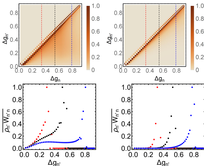
FIG. 8. Top panels: The normalized stationary probability flux |n'\rangle \rightarrow |n\rangle given by the function \overline{\rho_{n'}W_{n'n}} , Eq. (33). \Delta g_n = (g_n - g_{\text{min}})/(g_s - g_{\text{min}}) . The left and right panels refer to \bar{n} = 0 and \bar{n} = 0.05 , respectively. The scaled drive amplitude and the dimensionless Planck constant are f = 0.5 and \lambda = 0.004 in the both panels, so that the number of levels in a well of g(Q, P) is \approx 50 . Bottom panels: the normalized flux \overline{\rho_{n'}W_{n'n}} as a function of n' for the three values of n that correspond to the vertical red, black and blue cuts in the corresponding top panels. The dots are the cross-sections of the flux shown in the upper panels along the cuts, and the color coding of the dots corresponds to the color coding of the cuts. The left lower panel shows that, for \bar{n} = 0 , the decay of \overline{\rho_{n'}W_{n'n}} with the increasing interstate distance slows down for larger g_n and even becomes non-monotonic (see the blue dots). The right lower panel shows that, as the temperature increases, the decay of the flux \overline{\rho_{n'}W_{n'n}} becomes exponential in |g_n - g_{n'}| , indicating that the locality has been recovered.
