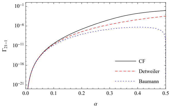
FIG. 1. Decay width \Gamma_{21-1} computed using continued fractions (solid black), the Detweiler approximation (dashed red) and the calculation of Ref. [25] (dotted blue), for a BH spin that saturates the superradiant amplification of the \ell = m = 1 mode [cf. Eq.(13)].
