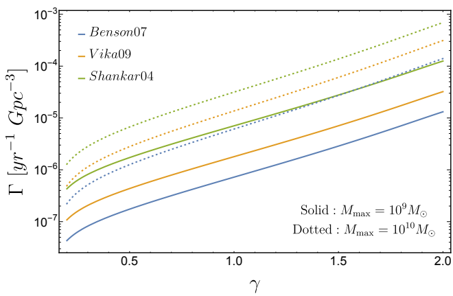
FIG. 5. \Gamma(\gamma) from the (fully) relaxed DM spikes with 3 different halo mass functions represented in the same colors. This result assumes the effect of loss-cone refilling on the DM spikes is negligible compared to the effect of relaxation. We plot \Gamma with M_{\max} = 10^9 M_{\odot} as solid lines and M_{\max} = 10^{10} M_{\odot} as dotted lines. Compared to the rate \Gamma from the original DM spikes in Fig. 4, it is significantly reduced for all \gamma values.
