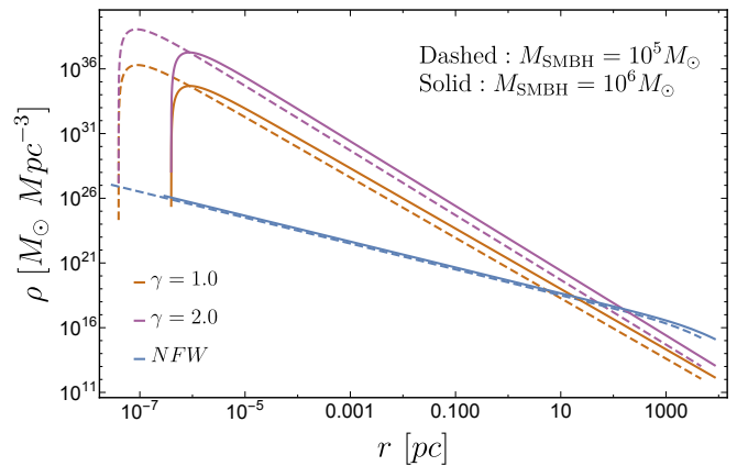
FIG. 1. A comparison of the NFW and spike-density profiles with \gamma = 1 or \gamma = 2 surrounding a SMBH with mass M_{\text{SMBH}} = 10^5 M_\odot or M_{\text{SMBH}} = 10^6 M_\odot . The spike profiles cross the NFW profile at r = R_{\text{sp}}(\gamma, M_{\text{SMBH}}) , defining the radius within which the merger rate will be calculated. Note that the NFW profile displays a \sim r^{-1} behavior inside this region, as expected.
