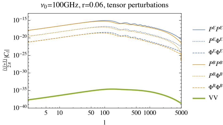
FIG. 2. The power spectra C_l for tensor perturbations. The blue and green curves are as in Fig. 1, but we now also have orange curves to indicate the analogous quantities for B modes.
