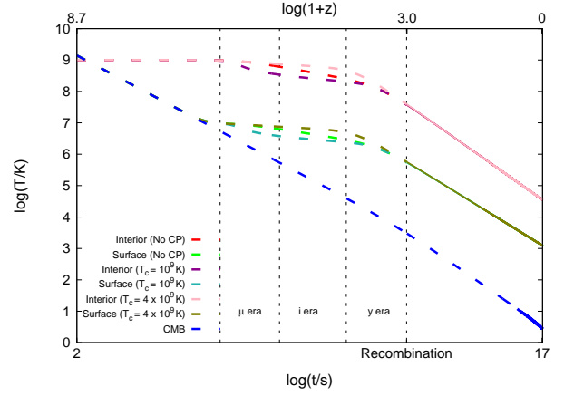
FIG. 1. Interior temperature T_X and surface temperature T_s of a Macro for M_X = M_\odot , \lambda = 1 and \rho_X = \rho_N , plotted versus time t and redshift z . Cooling is without DURca, and both without CP and with CP for two values of T_c . The ambient photon temperature T_{\text{CMB}} is shown for comparison, and the eras when \mu and y distortions occur are indicated.
