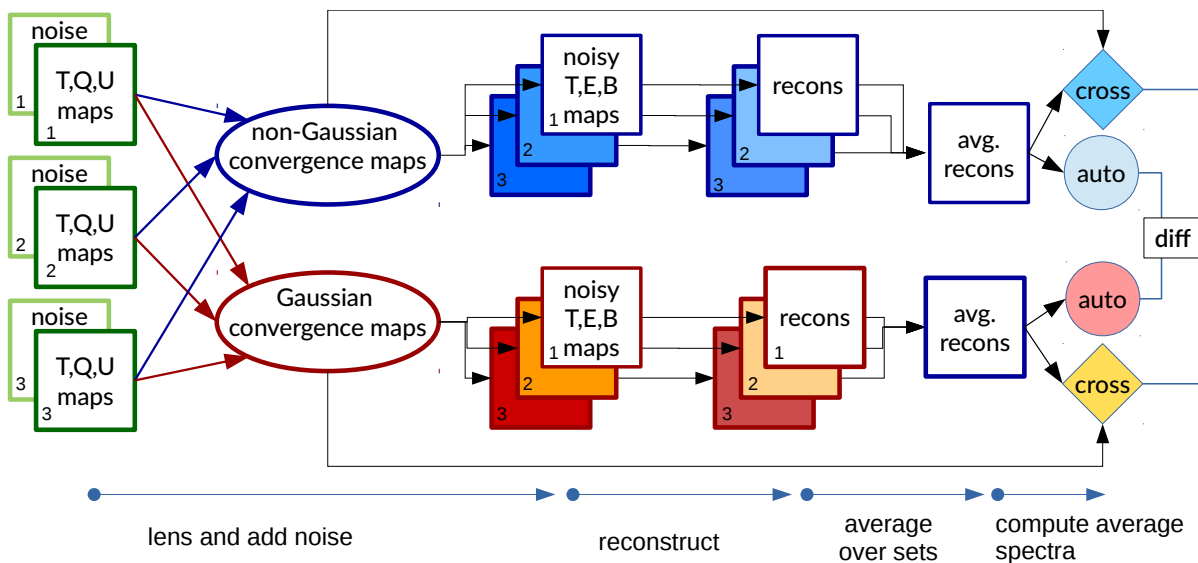
FIG. 1. Schematic outline of the simulation pipeline: Squares and ellipses represent sets of 10240 maps each. We start by generating 3 times 10240 unlensed CMB and noise realizations. We then lens each CMB realization with both a Gaussian and a non-Gaussian convergence map. Since we have 10240 Gaussian and non-Gaussian convergence maps, each of them is used to lens three independent CMB realizations. This results in two times three sets of 10240 lensed CMB maps. We convolve each of these maps with a Gaussian beam and add the same 3 times 10240 noise realizations to the Gaussian and non-Gaussian maps. After beam-deconvolution of the noisy maps, we run the standard quadratic estimator on every lensed CMB map. We average the reconstruction results over the maps that have been lensed with the same lensing convergence to beat down the reconstruction noise originating from the CMB sample variance. This leaves us with one set of 10240 averaged Gaussian and another set of 10240 averaged non-Gaussian reconstructed convergence maps. We compute the average power spectrum in each of these sets as well as the average cross correlation with the true underlying convergence realizations. Any significant difference between the average power spectra of the non-Gaussian and Gaussian simulations is a non-Gaussian bias.
