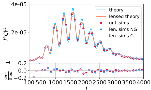
FIG. 6. The average power spectra of the unlensed and lensed polarization E-modes agree with the theory prediction except for large scales, where we find a significant deviation at l < 500 . We exclude these scales from the reconstruction. Note that the errorbars on the measured power spectra are smaller than the markers.
