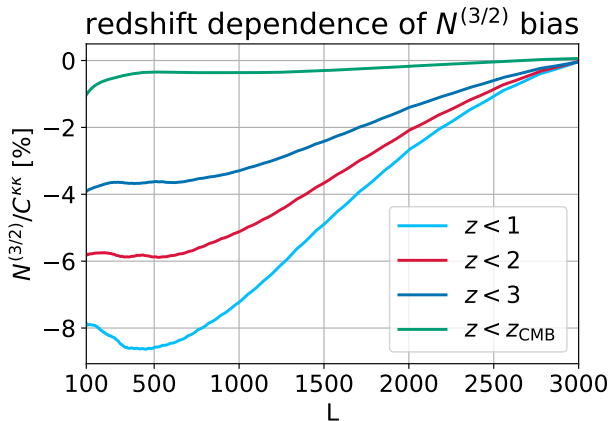
FIG. 15. The relative size of the non-Gaussian bias increases if we only consider lenses at low redshifts z_{\max} < z_{\text{CMB}} . This is a consequence of the different redshift-scalings of the competing terms in the lensing bispectrum from non-linear structure formation and post Born effects. To illustrate this we ignore any contributions to the lensing bispectrum and power spectrum with z > z_{\max} and plot the ratio of the resulting cross bias to the power spectrum. These results suggest that the non-Gaussian bias could be more important for measurements of cross correlations of CMB lensing with low-redshift tracers. We note that the curves shown here are still preliminary and should be seen as a motivation to investigate the bias on cross correlations in future work (Böhm et al. in prep.). Note that the curves show the bias from gradient modes only and do not take into account lensing by curl modes.
