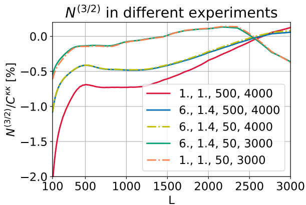
FIG. 14. Bispectrum-induced N^{(3/2)} bias in temperature-based measurements for different experimental configurations. Different to the results shown in BSS16, these curves are derived from a lensing bispectrum model that includes post-Born correction and uses a simulation-calibrated fitting formula to the matter bispectrum. The lines are labeled by noise in \mu K —arcmin, beam FWHM in arcmin, l_{\min} and l_{\max} . The size of the bias is sensitive to the maximal, signal-dominated CMB scale that is used in the reconstruction.
