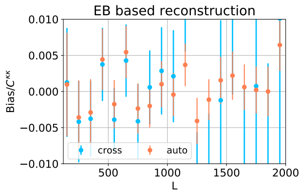
FIG. 12. The non-Gaussian bias to CMB lensing measurements from (EB, EB) is consistent with zero in both auto and cross correlations. This seems in agreement with BSS16, who have not numerically evaluated the bias expressions for polarization, but argue that they are expected to be smaller than in temperature due to their additional angular dependencies.
