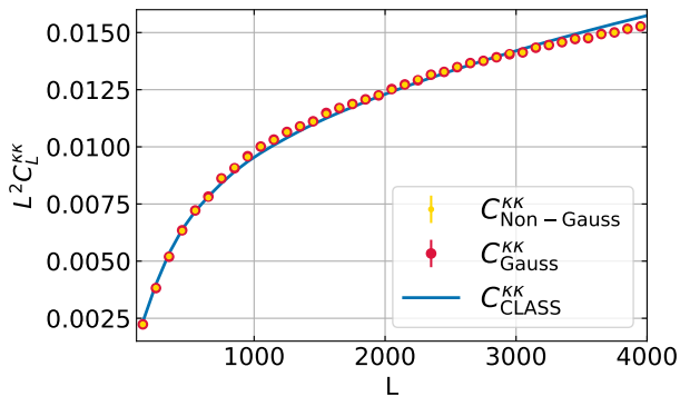
FIG. 2. Power spectra measured from 10240 Gaussian (red) and ray-traced non-Gaussian (yellow) convergence maps closely follow the theory curve computed with CLASS (blue). Errorbars corresponding to the standard deviation of the mean between the binned power spectra of the 10240 maps are plotted but too small to be visible. For modeling non-linear effects in the matter power spectrum CLASS uses a version of HALOFIT [62]. We use precision parameters tol_perturb_integration=1e-6 , perturb_sampling_stepsize=0.01 , k_min_tau0=0.002 , k_max_tau0_over_l_max=10. , halofit_k_per_decade=3000 and l_max_scalars=8000 to produce the theory curve. Missing power on small scales is owed to the finite resolution of the simulation.
