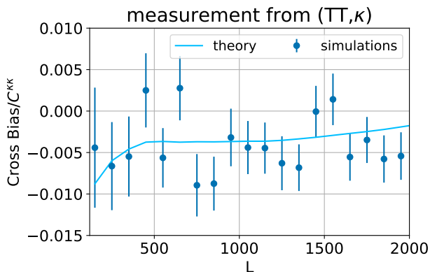
FIG. 8. We detect a non-Gaussian bias in the cross correlation of temperature-based reconstructions and input maps with a significance of 5.21\sigma . For a null-hypothesis of no bias we find a p-value of 0.0003. Using the theoretical bias curve computed with analytic expressions from BSS16 (plotted in light blue) as null-hypothesis results in a p-value of 0.3932.
