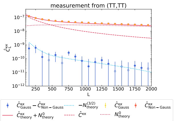
FIG. 10. Measured non-Gaussian bias in the CMB lensing four-point function. The reconstruction agrees well with the theory prediction (red curve) which we model as a sum of convergence power C_L^{\kappa\kappa} and N^{(0)} lensing bias. The measured non-Gaussian bias is consistent with the theory prediction of BSS16, but the null-hypothesis of no bias cannot be excluded with high statistical significance.
