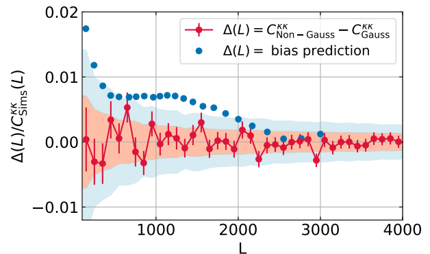
FIG. 3. For an accurate measurement of the non-linear bias in the reconstructions it is crucial that the power spectra of the original, non-reconstructed, Gaussian and non-Gaussian simulations are consistent within their sample variance. We show that this is indeed the case by checking that their difference is consistent with zero (red dots, \chi^2/\nu = 1.02 , with \nu = 38 degrees of freedom, corresponding to a p-value of 0.444). We further require the sample variance of both sets to be small enough to allow a detection of a bias at the percent-level. To see this, we plot the combined sample variance of both sets as shaded regions ( \pm\sigma, \pm 2\sigma ) and compare it to the expected size of the non-linear bias (blue dots).
