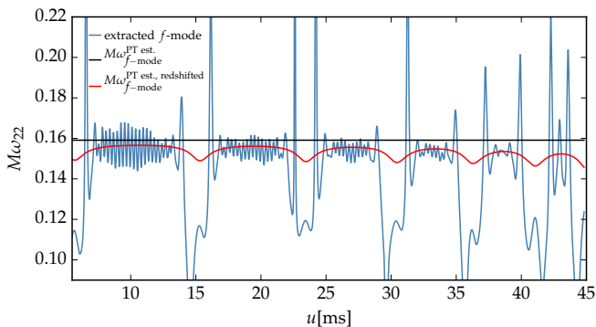
FIG. 12. Instantaneous frequency of \Psi_{2,2}^{4,f\text{-mode}} for SLy- e0.50^{00} -R4, compared to the prediction of the f -mode frequency of an isolated star, as well as the f -mode frequency including the estimated gravitational redshift due to the star's companion. These curves should only be compared away from the periastron bursts.
