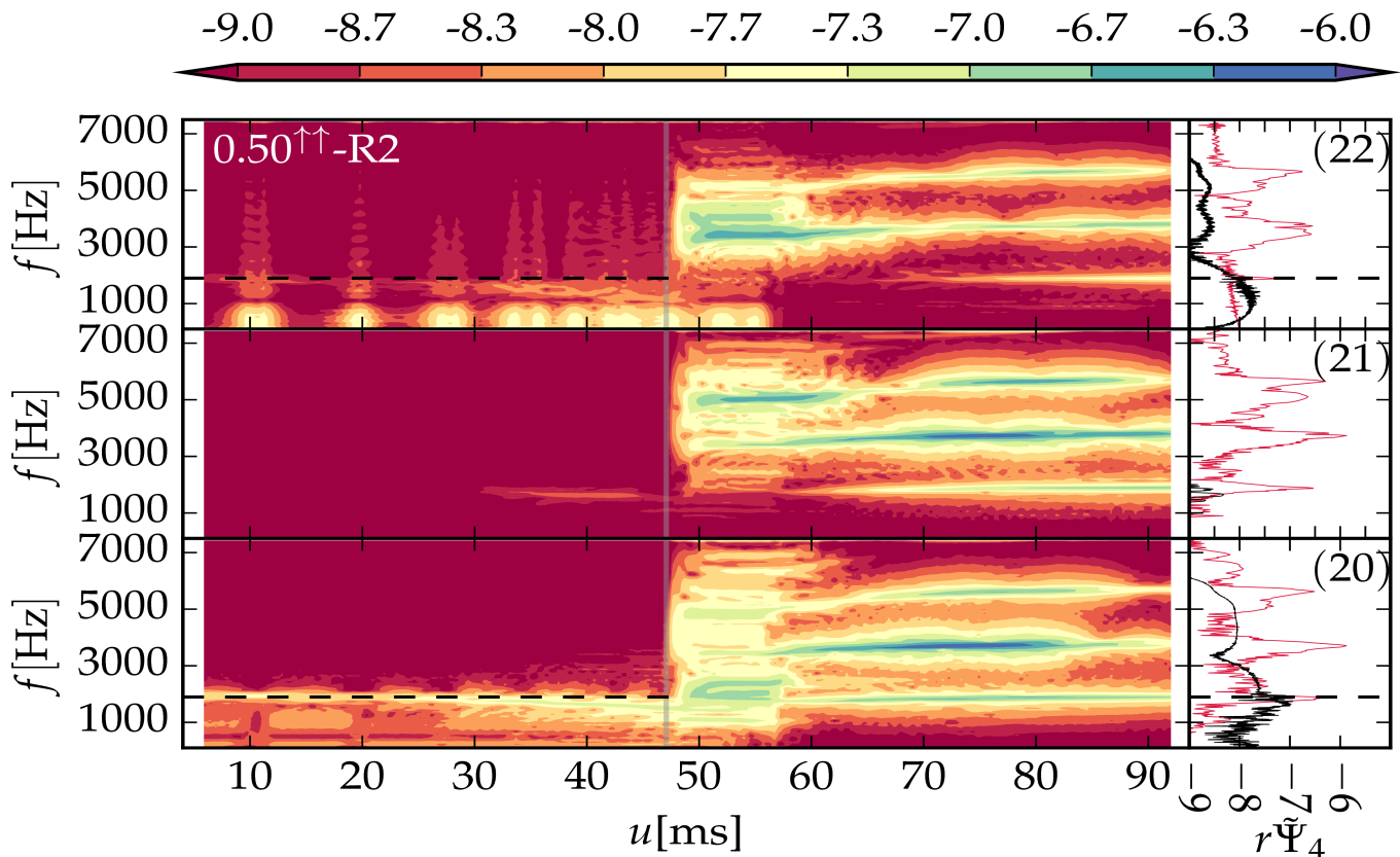
FIG. 11. Spectrogram (left) and power spectral density (right) of the curvature scalar r\tilde{\Psi}_4 for the SLy- e0.50^{\uparrow} -R2 configuration. The labels in the right panel plot refer to the (22), (21), and (20) modes of the curvature scalar. The black dashed line marks the PT estimate of the f -mode frequency for non-spinning stars and the gray line marks the moment of merger. The PSD is split into a part before the moment of merger (black) and a part after the merger (crimson).
