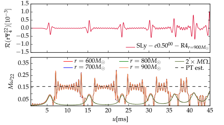
FIG. 9. r\Psi_4^{22} extracted at r = 900M_\odot and instantaneous GW frequency M\omega_{22} computed from the phase of r\Psi_4^{22} (note that the curves at different extraction radii are coincident) plotted alongside 2 \times M\Omega as computed from the coordinate tracks of the NSs, both for the inspiral part of the SLy- e0.50^{00} - R4 case. We find a good agreement for the relation M\omega_{22} = 2 \times M\Omega and similar results hold for all the other cases. The higher frequency in-between the periastron encounters correspond to the quasi-normal mode excitations of the NSs. We also plot the perturbation theory (PT) estimate for the f -mode frequency as a black dashed line.
