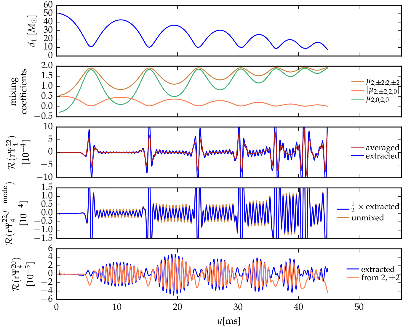
FIG. 13. Illustration of the effects of displacement-induced mode mixing on the waveforms extracted from SLy- \epsilon 0.50^{00} -R4: Coordinate distance from star 1 to the origin ( top ); mode mixing coefficients ( second-from-top ) ( |\mu_{2,\pm 2; 2, \mp 2}| is almost indistinguishable from 0 at this scale, so we do not show it); illustrating the averaging used to separate the f -mode and orbital signals ( third-from-top ); comparing the full mode mixing calculation of the intrinsic f -mode contribution to the real part of the (2, 2) mode from a single star to the naive calculation of taking half of the extracted mode ( second-from-bottom ) (the result for the imaginary part is exactly analogous); comparing the contribution to the real part of the (2, 0) mode from mode mixing to that extracted from the evolution of the binary ( bottom ) (the imaginary part vanishes). In all cases, the approximations used to compute the mode mixing are only valid during the inter-burst f -mode oscillations, and the predictions of the mode mixing calculation for the periastron bursts should not be considered.
