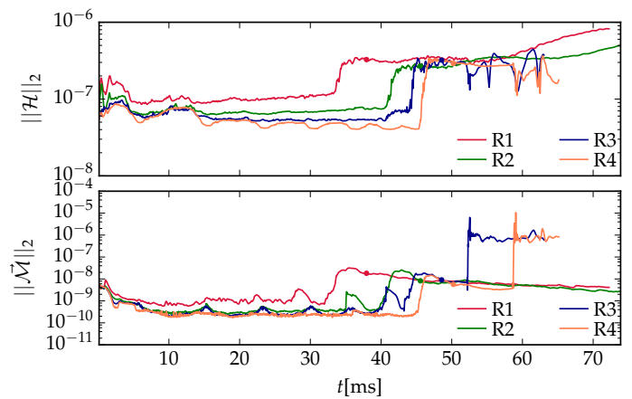
FIG. 16. ADM constraints for the \text{SLy}-e0.50^{00} case. The upper panel shows the L^2 volume norm of the Hamiltonian constraint, \|\mathcal{H}\|_2 . The lower panel shows the L^2 volume norms of the Cartesian components of the momentum constraint, \|\vec{\mathcal{M}}\|_2 = \sqrt{\|\mathcal{M}^x\|_2^2 + \|\mathcal{M}^y\|_2^2 + \|\mathcal{M}^z\|_2^2} . The constraints are evaluated on refinement level 4 and are decreasing for increasing resolution during the inspiral of the neutron stars. Note that here we restrict our convergence analysis to the refinement level 4, cf. Tab. I. This is needed since for the coarser refinement levels even the higher resolution setups are only barely able to resolve the star whereas for the coarser resolutions not a single point covers the NS leading to a non-convergent behavior. We have filtered our data with an average filter to give a better visualization and reduce high frequency noise and mark the times of merger by circles.
