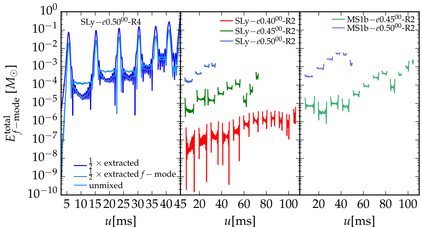
FIG. 14. Estimate of the energy stored in f -mode oscillations as a function of the retarded time. ( Left panel ): Comparison of the results after accounting for displacement-induced mode mixing to those obtained using half the extracted signal, both plain (i.e. the pure extracted signal), and with only the f -mode part for SLy- e0.50^{00} -R4. The energy estimate is only valid in the times between the periastron bursts. ( Middle and right panels ): The energy estimate computed accounting for displacement-induced mode mixing for the nonspinning SLy and MS1b cases that have multiple encounters before merger, considering the R2 resolutions for which we have data for the most eccentricities. In order to clarify these plots, we have excluded the portions of the traces that are close to the periastron bursts.
